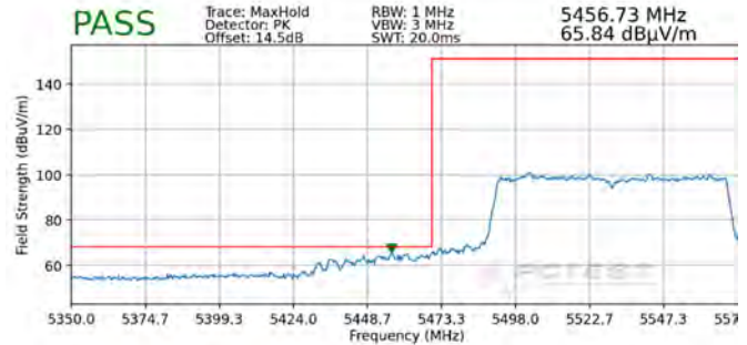
Plot 7-332. Radiated Lower Band Edge Plot MIMO (Peak – UNII Band 2C)
