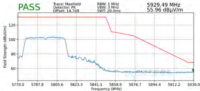
Plot 7-326. Radiated Upper Band Edge Plot MIMO (Peak – UNII Band 3)
