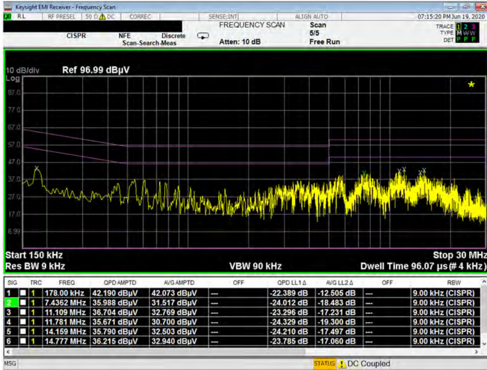
Plot 7-341. Line Conducted Plot with 802.11a UNII Band 3 (L1)
