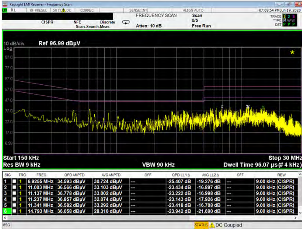
Plot 7-337. Line Conducted Plot with 802.11a UNII Band 2A (L1)
