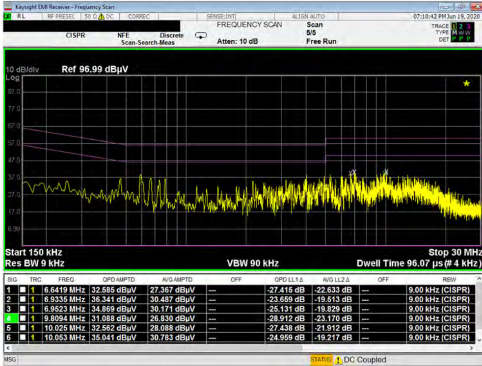
Plot 7-339. Line Conducted Plot with 802.11a UNII Band 2C (L1)
