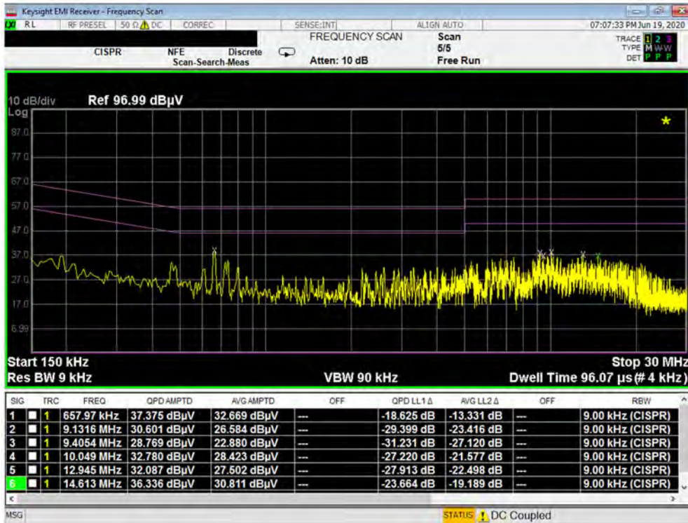
Plot 7-338. Line Conducted Plot with 802.11a UNII Band 2A (N)
