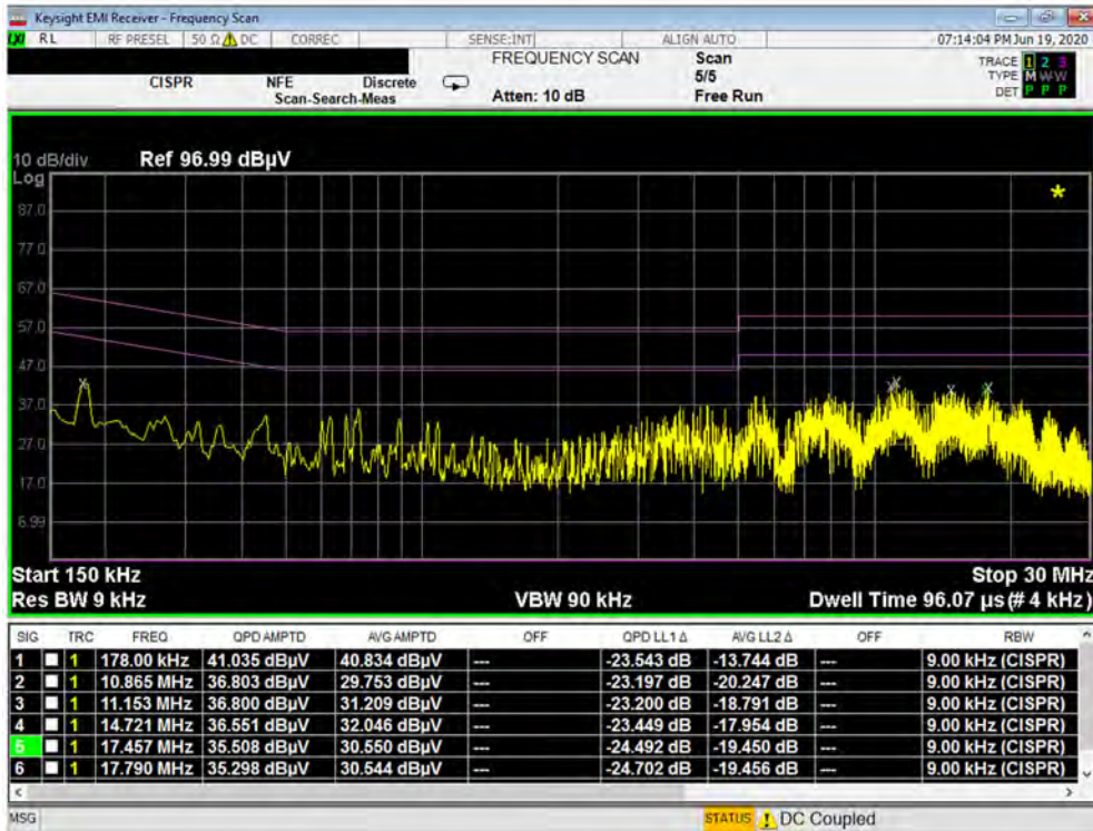
Plot 7-342. Line Conducted Plot with 802.11a UNII Band 3 (N)
