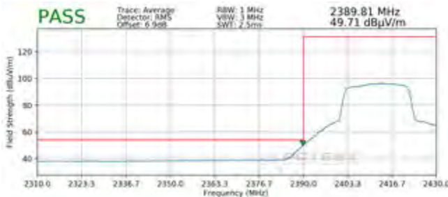
Plot 7-88. Radiated Restricted Lower Band Edge Measurement SISO ANT1 (Average)
