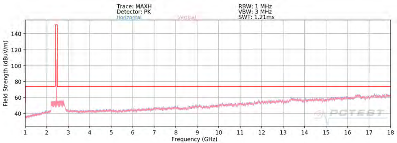
Plot 7-83. Radiated Spurious Plot above 1GHz SISO ANT2 (802.11b – Ch. 11)
