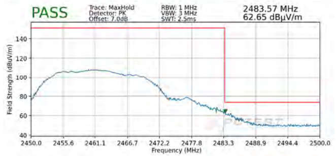
Plot 7-91. Radiated Restricted Upper Band Edge Measurement SISO ANT1 (Peak)
