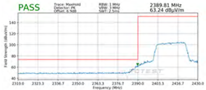
Plot 7-114. Radiated Restricted Lower Band Edge Measurement MIMO (Peak – 242 Tones)
