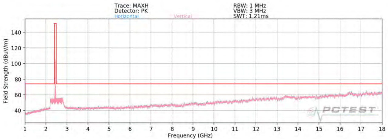
Plot 7-89. Radiated Spurious Plot above 1GHz MIMO (802.11ax OFDMA – 242 Tones – Ch. 6)
