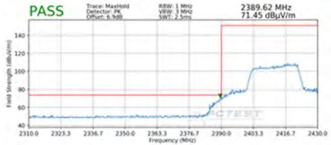
Plot 7-98. Radiated Restricted Lower Band Edge Measurement SISO ANT1 (Peak – 242 Tones)
