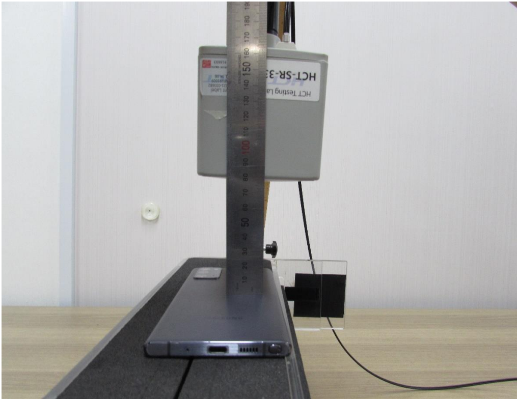
Distance from the rear side of the Device to the center of the Probe from 13.4 cm
