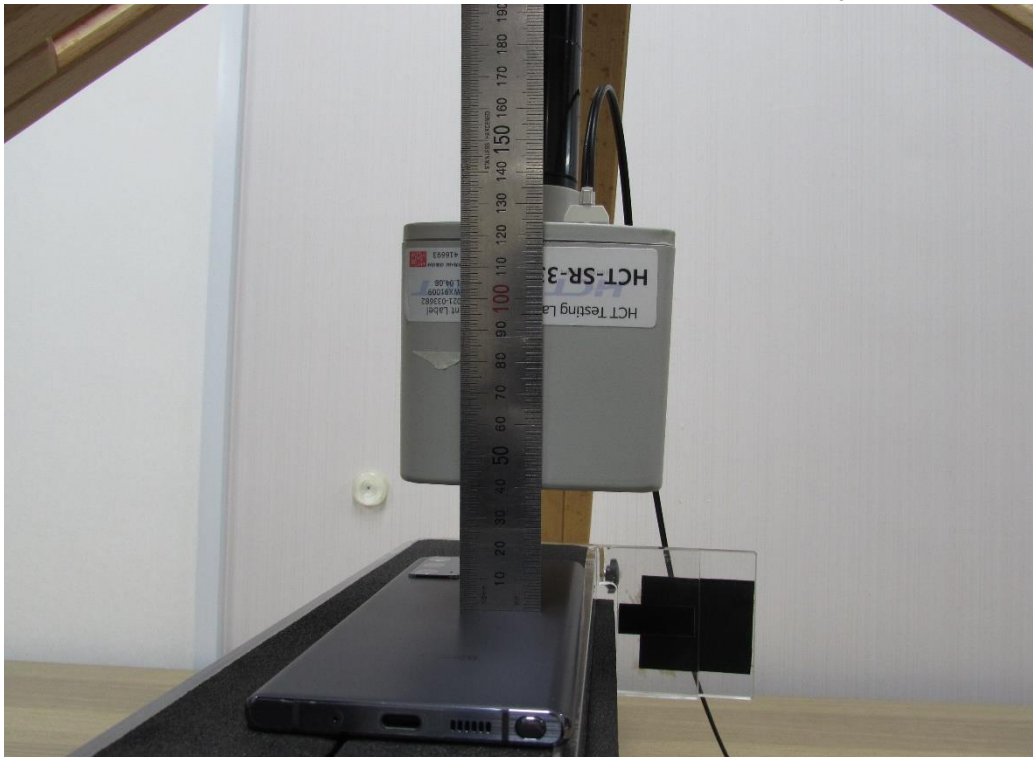
Distance from the rear side of the Device to the center of the Probe from 9.4 cm
