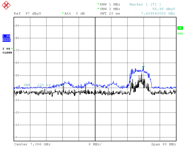
Radiated Spurious Emissions plot – Peak result (802.11ax(HE20), Ch.11 3rd Harmonic)
