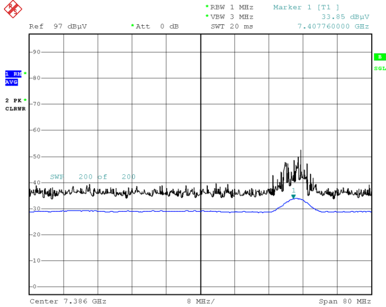
Radiated Spurious Emissions plot – Average result (802.11ax(HE20), Ch.11 3rd Harmonic)
