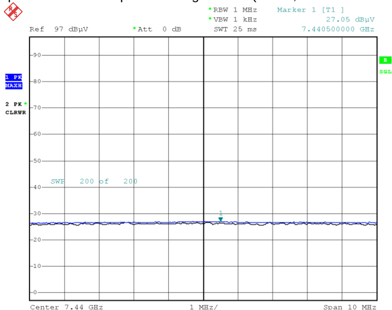
Radiated Spurious Emissions plot – Average Result (GFSK, Ch.78 3rd Harmonic, Z-H)
