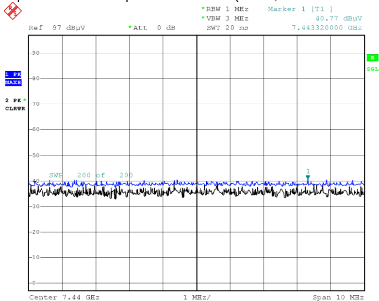
Radiated Spurious Emissions plot – Peak Result (GFSK, Ch.78 3rd Harmonic, Z-H)
