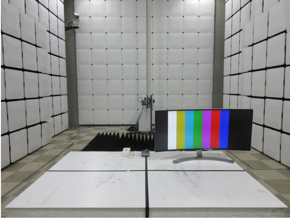
[EUT+LED Monitor]
