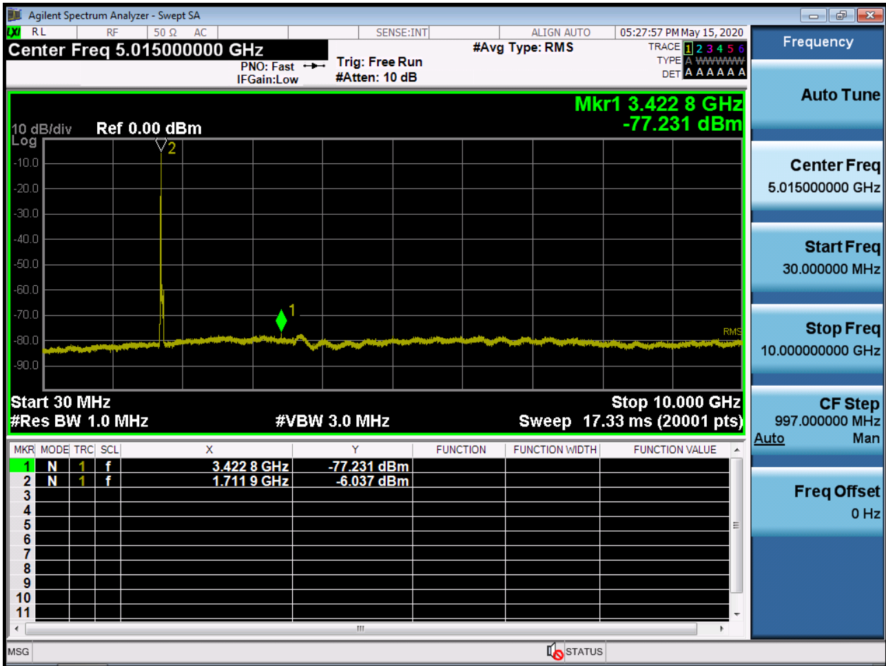
BAND 66/4. Conducted Spurious Plot_1 (132072ch_20MHz_QPSK_RB 1_0)
