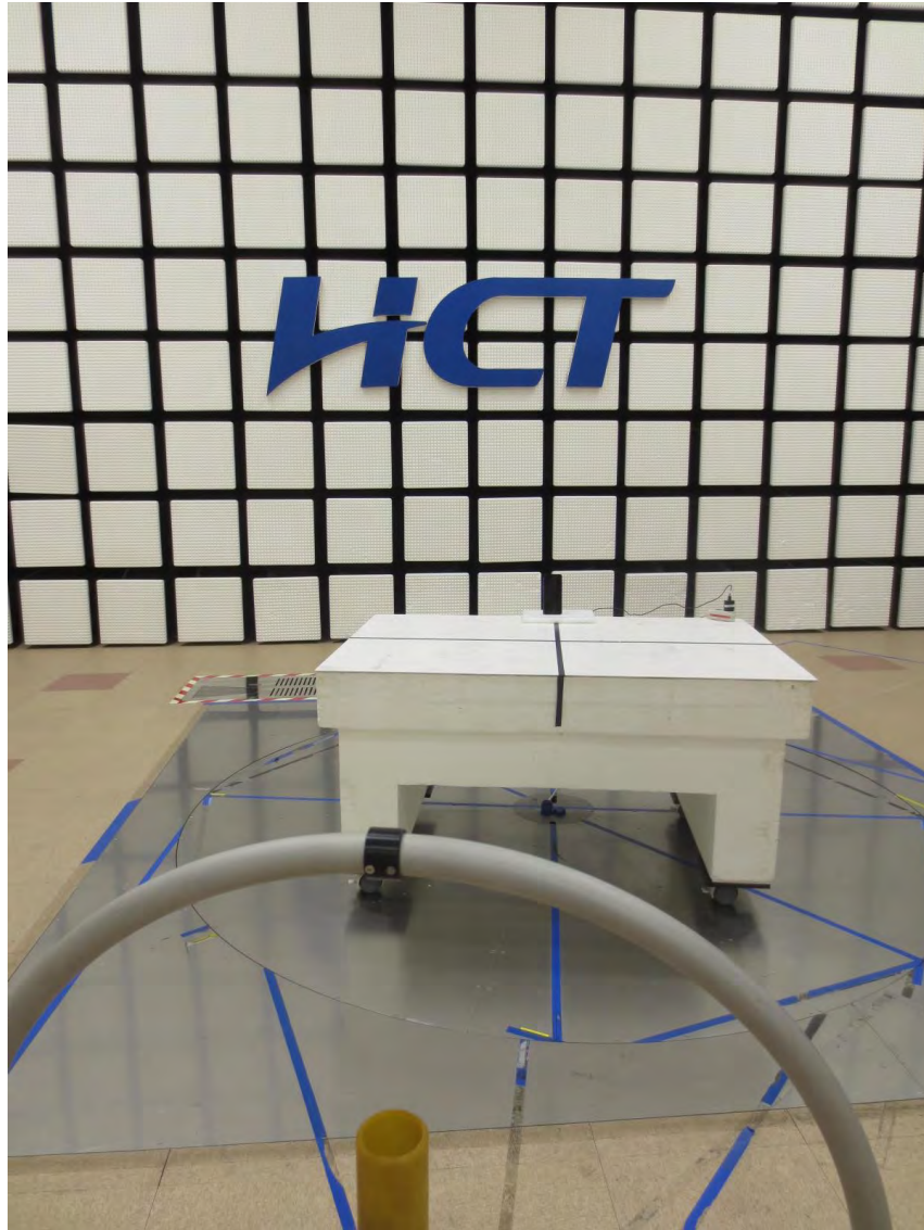
WPT Radiated Test Setup Photo for below 30 MHz: With TA aligned
