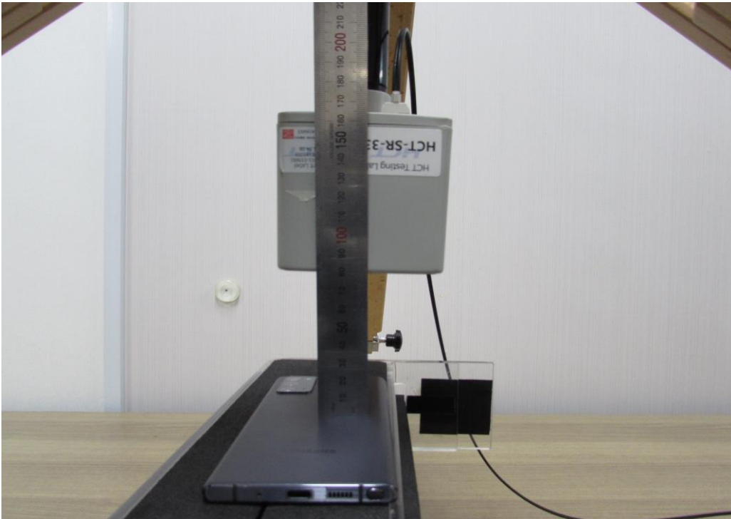
Distance from the rear side of the Device to the center of the Probe from 13.4 cm
