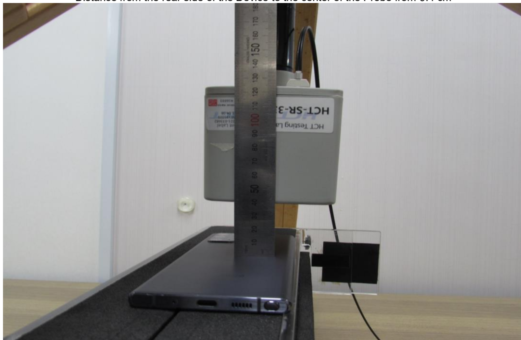
Distance from the rear side of the Device to the center of the Probe from 9.4 cm
