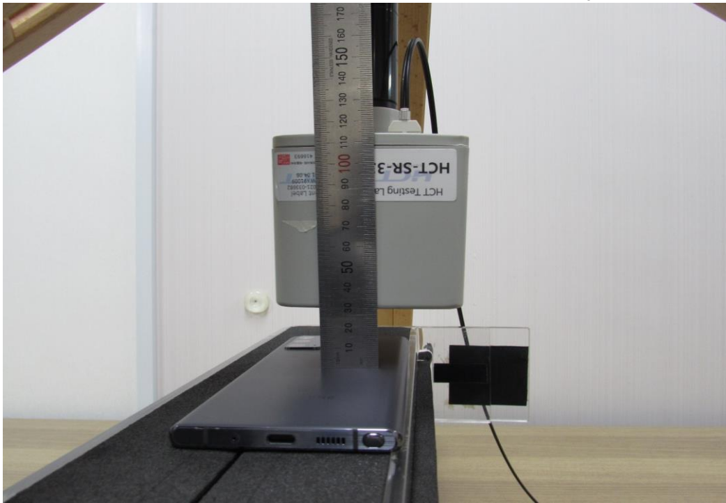
Distance from the rear side of the Device to the center of the Probe from 9.4 cm
