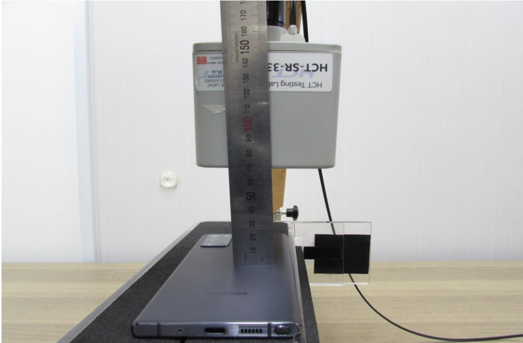
Distance from the rear side of the Device to the center of the Probe from 12.4 cm
