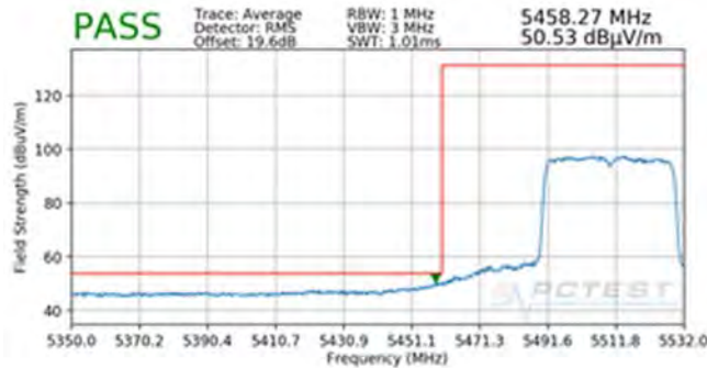
Plot 7-414. Radiated Lower Band Edge Plot MIMO (Average – UNII Band 2C – 484 Tones)
