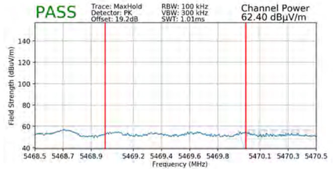
Plot 7-422. Radiated Lower Band Edge Plot MIMO (Peak – UNII Band 2C – 996 Tones)
