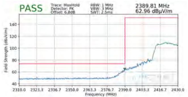
Plot 7-126. Radiated Restricted Lower Band Edge Measurement MIMO (Peak)
