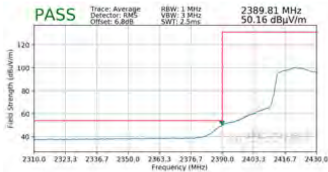
Plot 7-125. Radiated Restricted Lower Band Edge Measurement MIMO (Average)
