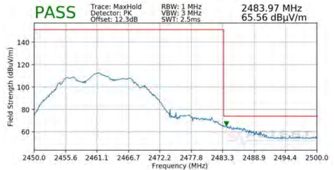
Plot 7-142. Radiated Restricted Upper Band Edge Measurement CDD (Peak)
