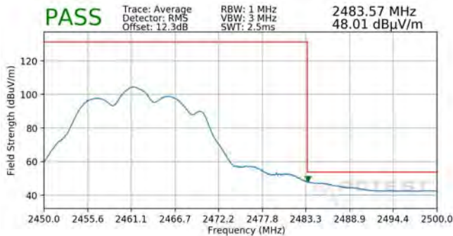
Plot 7-141. Radiated Restricted Upper Band Edge Measurement CDD (Average)
