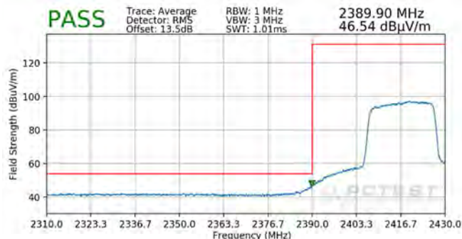
Plot 7-133. Radiated Restricted Lower Band Edge Measurement MIMO (Average – 242 Tones)
