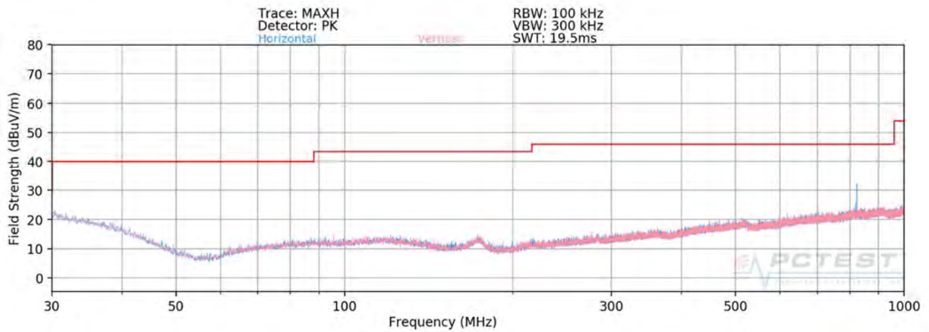
Plot 7-140. Radiated Spurious Plot below 1GHz MIMO (242 Tones)
