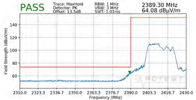
Plot 7-124. Radiated Restricted Lower Band Edge Measurement MIMO (Peak – 106 Tones)
