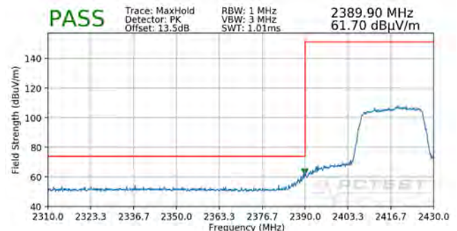
Plot 7-134. Radiated Restricted Lower Band Edge Measurement MIMO (Peak – 242 Tones)
