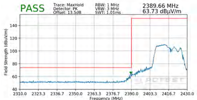
Plot 7-126. Radiated Restricted Lower Band Edge Measurement MIMO (Peak – 106 Tones)
