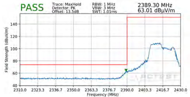
Plot 7-110. Radiated Restricted Lower Band Edge Measurement SISO ANT2 (Peak – 106 Tones)
