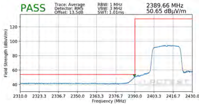
Plot 7-115. Radiated Restricted Lower Band Edge Measurement SISO ANT2 (Average – 242 Tones)
