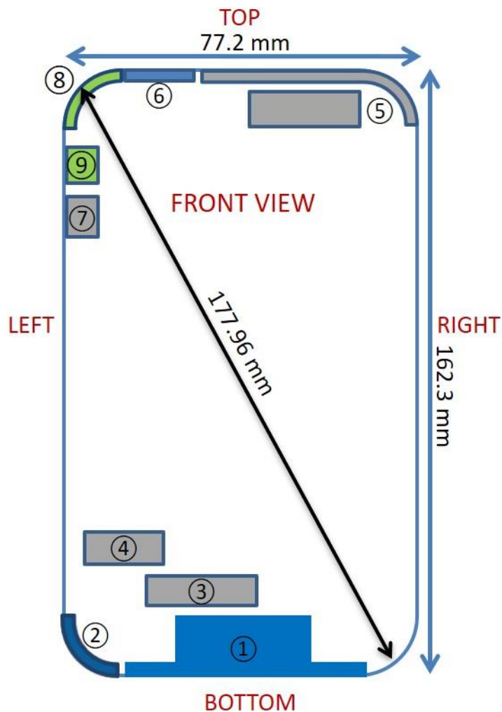
Figure E-1 DUT Antenna Locations
