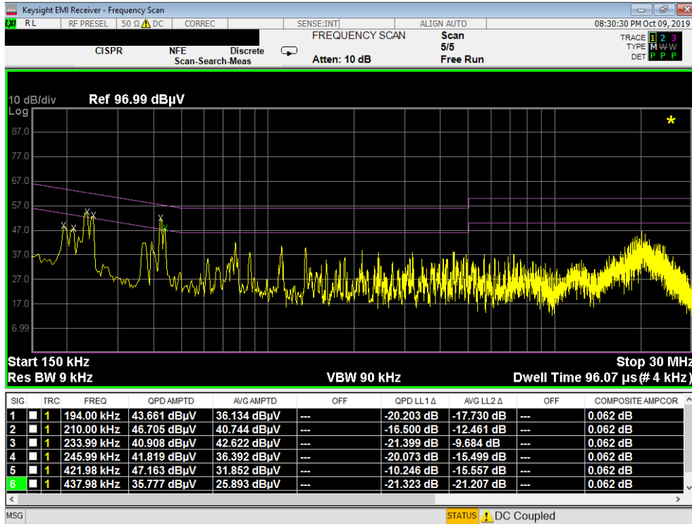
Plot 7-56. Line Conducted Plot with Bluetooth LE with WCP (L1)
