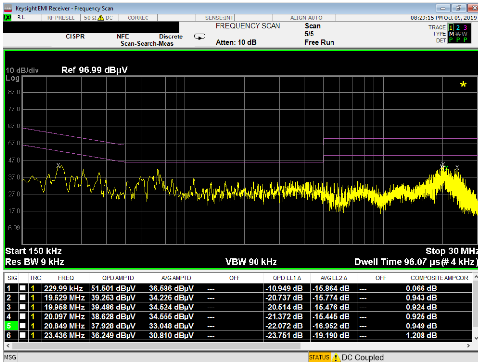
Plot 7-57. Line Conducted Plot with Bluetooth LE with WCP (N)
