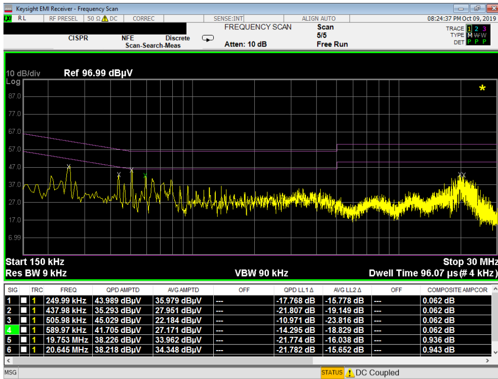
Plot 7-55. Line Conducted Plot with Bluetooth LE (N)
