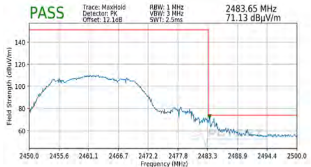
Plot 7-104. Radiated Restricted Upper Band Edge Measurement MIMO (Peak)
