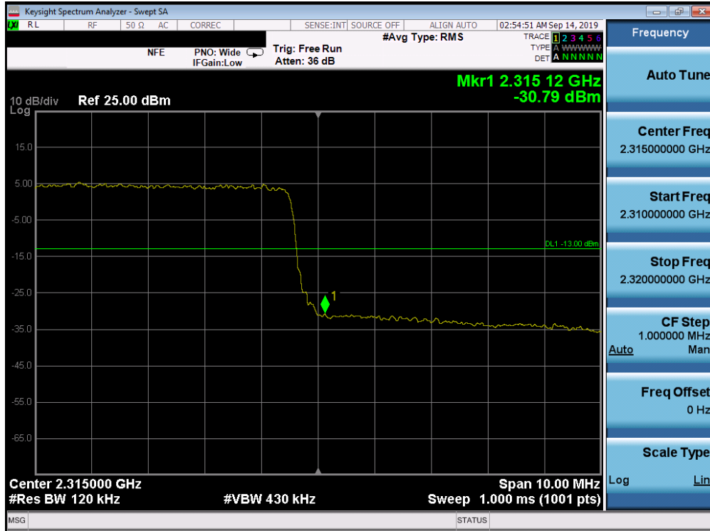
Plot 7-343. Upper Band Edge Plot (Band 30 - 10.0MHz QPSK - Full RB Configuration)
