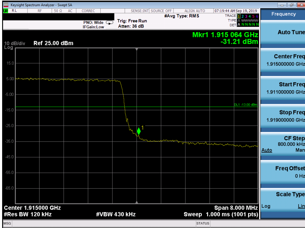
Plot 7-323. Upper Band Edge Plot (Band 25 - 10.0MHz QPSK - Full RB Configuration)
