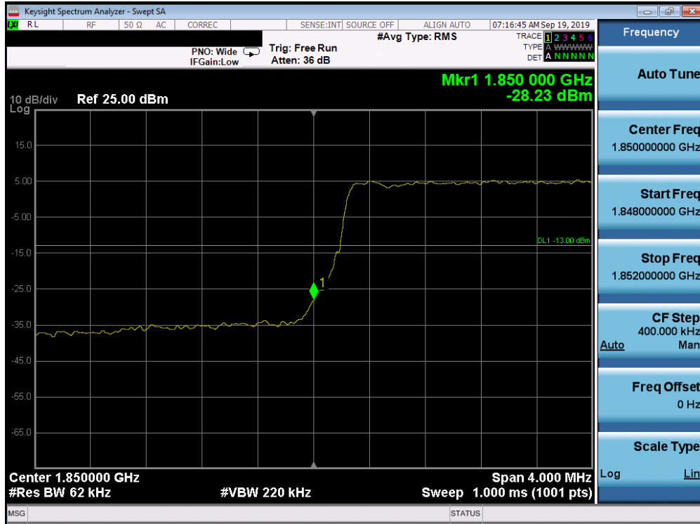
Plot 7-313. Lower Band Edge Plot (Band 25/2 - 5.0MHz QPSK - Full RB Configuration)
