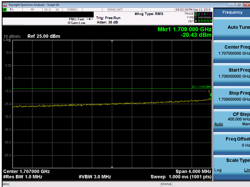
Plot 7-284. Lower Extended Band Edge Plot (Band 66/4 - 10.0MHz QPSK - Full RB Configuration)
