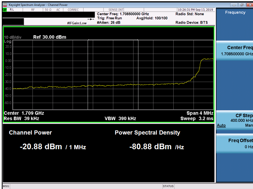
Plot 7-278. Lower Extended Band Edge Plot (Band 66/4 - 5.0MHz QPSK - Full RB Configuration)
