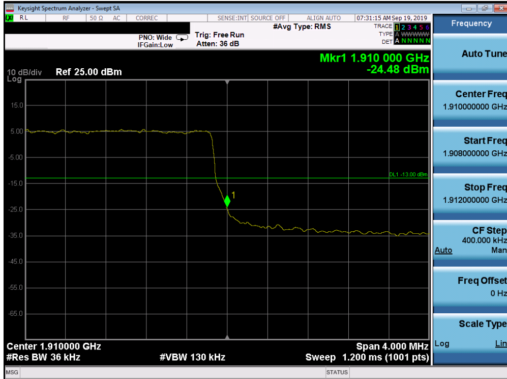
Plot 7-309. Upper Band Edge Plot (Band 2 - 3.0MHz QPSK - Full RB Configuration)
