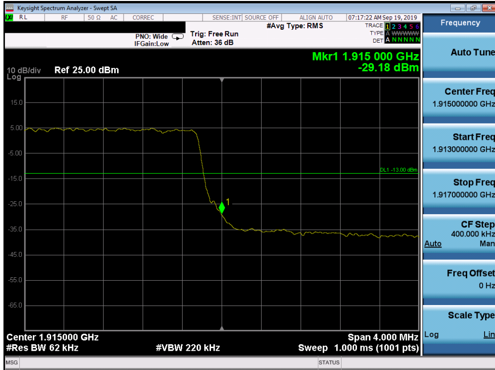
Plot 7-317. Upper Band Edge Plot (Band 25 - 5.0MHz QPSK - Full RB Configuration)
