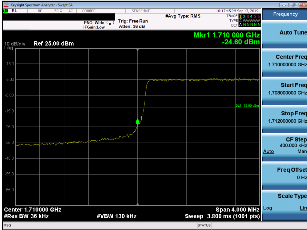
Plot 7-271. Lower Band Edge Plot (Band 66/4 - 3.0MHz QPSK - Full RB Configuration)
