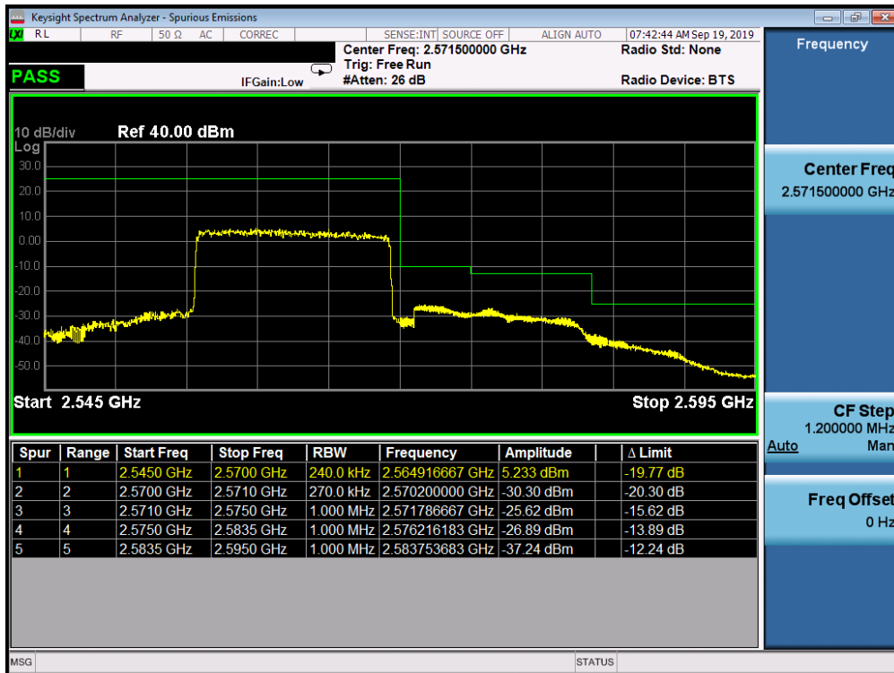
Plot 7-350. Higher ACP Plot (Band 7 - 15.0MHz QPSK - Full RB Configuration)
