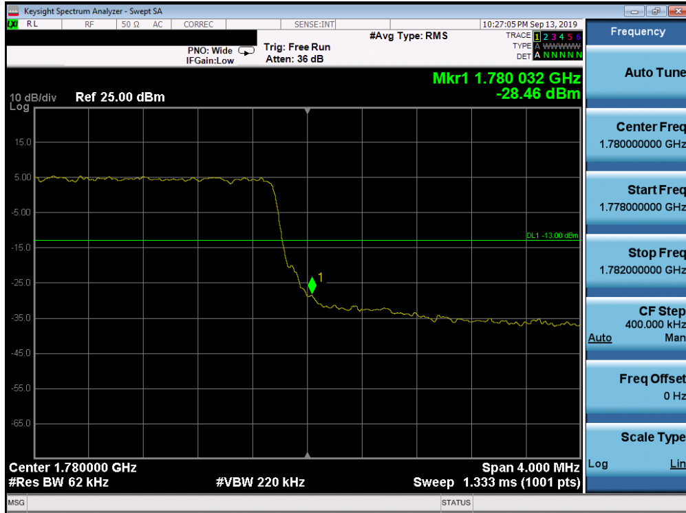
Plot 7-281. Upper Band Edge Plot (Band 66 - 5.0MHz QPSK - Full RB Configuration)
