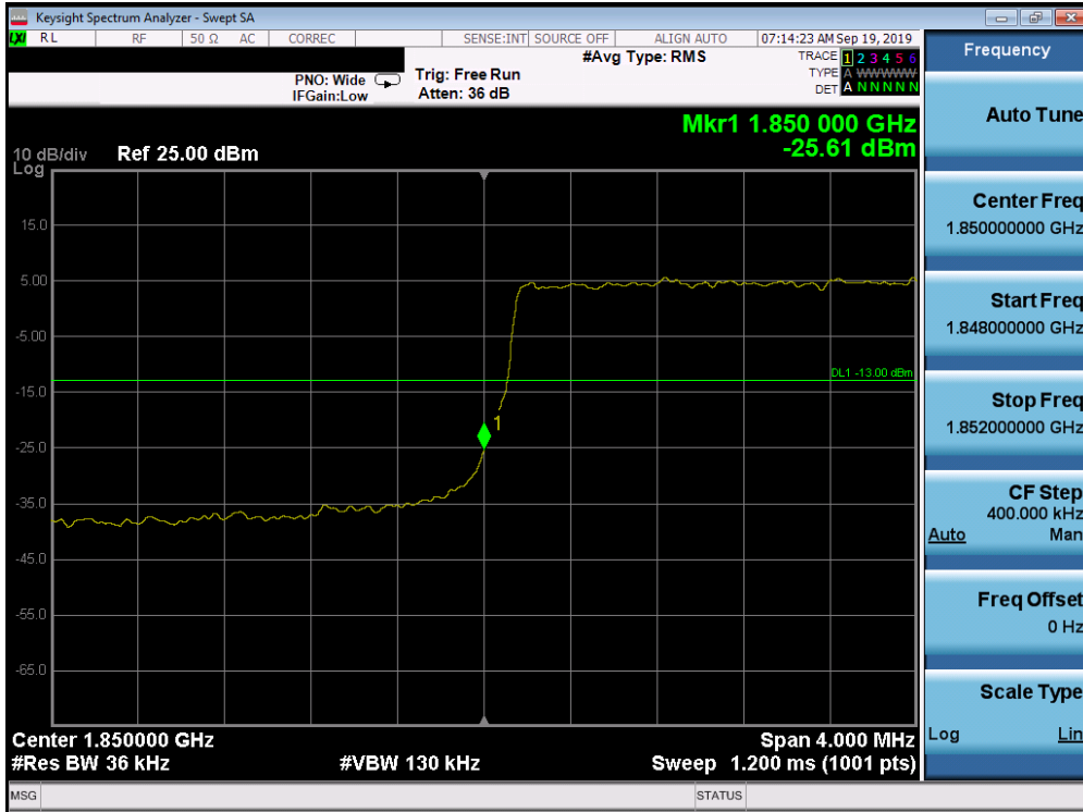
Plot 7-307. Lower Band Edge Plot (Band 25/2 - 3.0MHz QPSK - Full RB Configuration)
