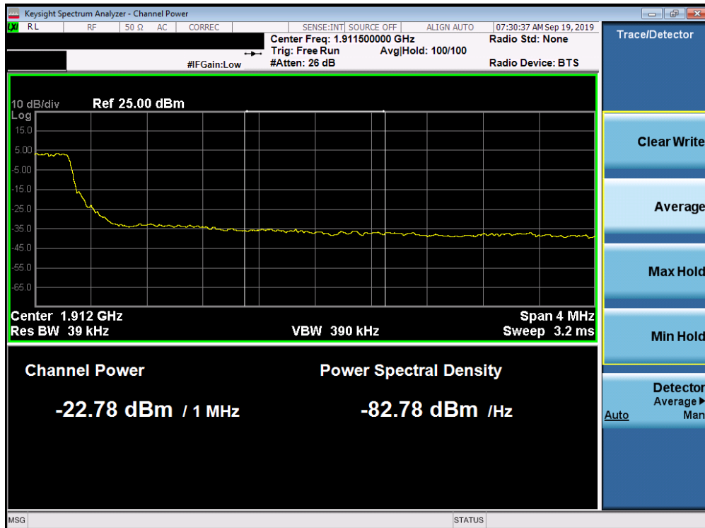
Plot 7-316. Upper Extended Band Edge Plot (Band 2 - 5.0MHz QPSK - Full RB Configuration)
