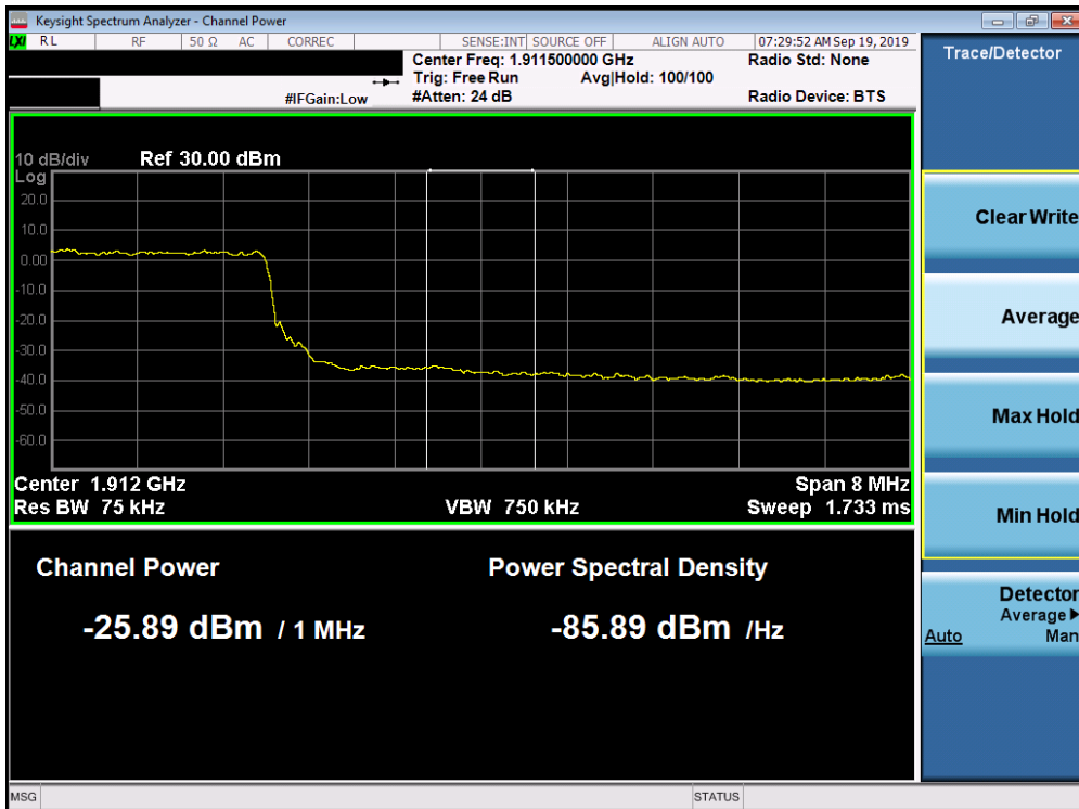
Plot 7-322. Upper Extended Band Edge Plot (Band 2 - 10.0MHz QPSK - Full RB Configuration)
