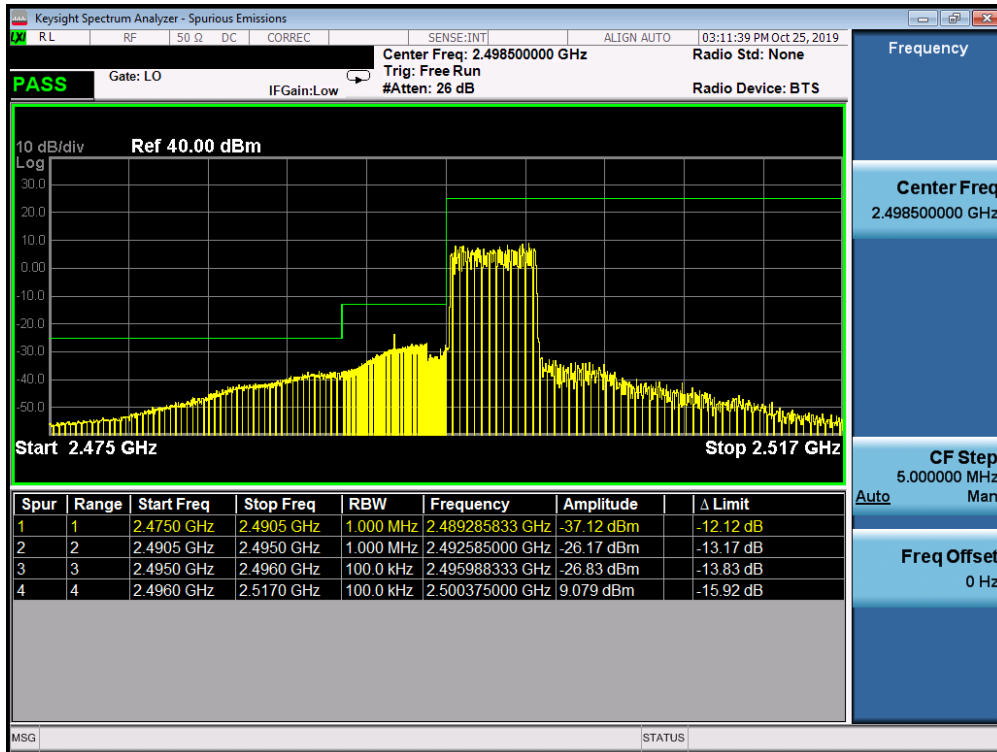
Plot 7-353. Lower ACP Plot at 2496 MHz (Band 41 - 5.0MHz QPSK - Full RB Configuration)
