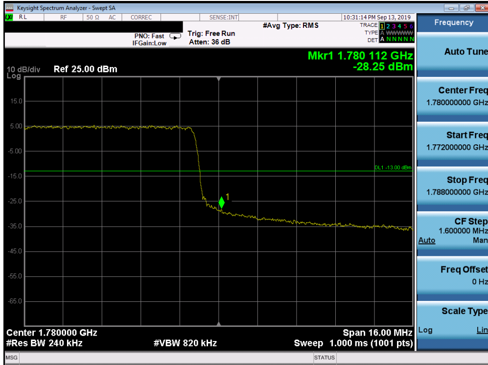
Plot 7-299. Upper Band Edge Plot (Band 66 - 20.0MHz QPSK - Full RB Configuration)
