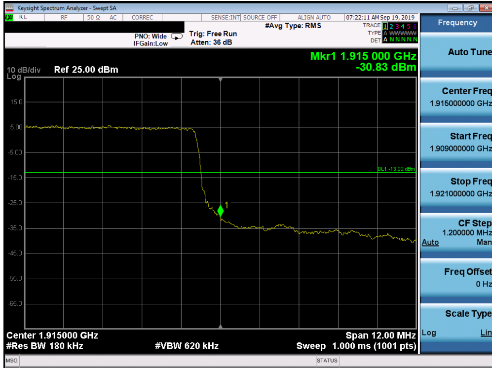
Plot 7-329. Upper Band Edge Plot (Band 25 - 15.0MHz QPSK - Full RB Configuration)
