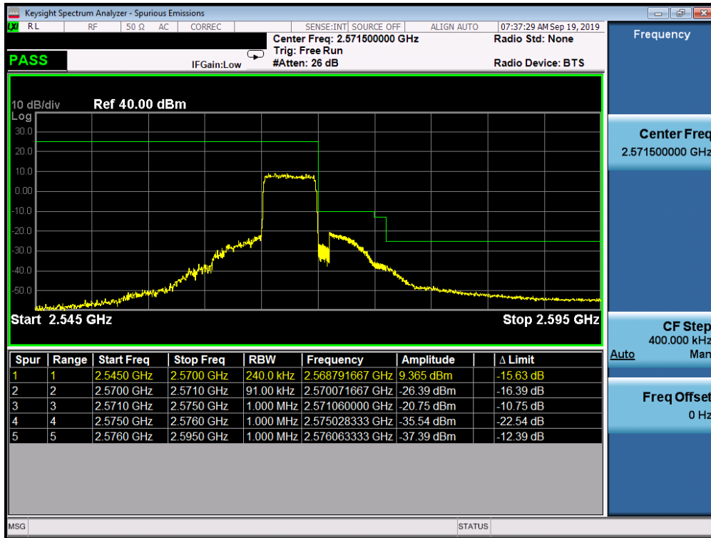
Plot 7-346. Higher ACP Plot (Band 7 - 5.0MHz QPSK - Full RB Configuration)
