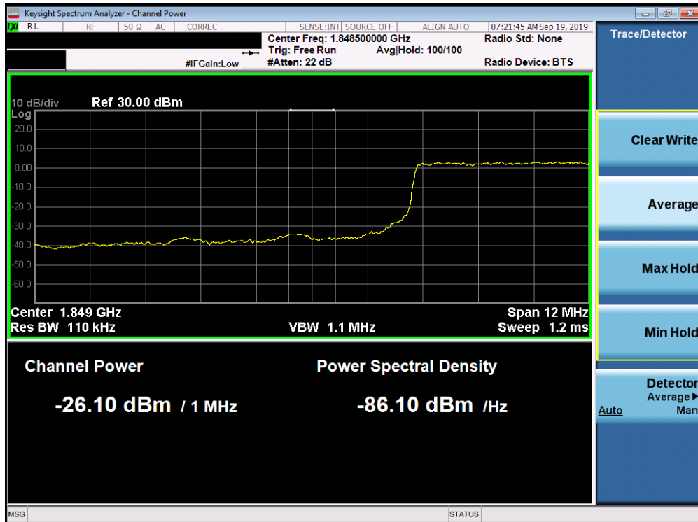
Plot 7-326. Lower Extended Band Edge Plot (Band 25/2 - 15.0MHz QPSK - Full RB Configuration)
