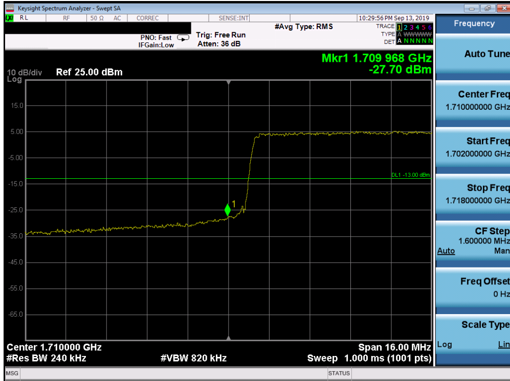
Plot 7-295. Lower Band Edge Plot (Band 66/4 - 20.0MHz QPSK - Full RB Configuration)
