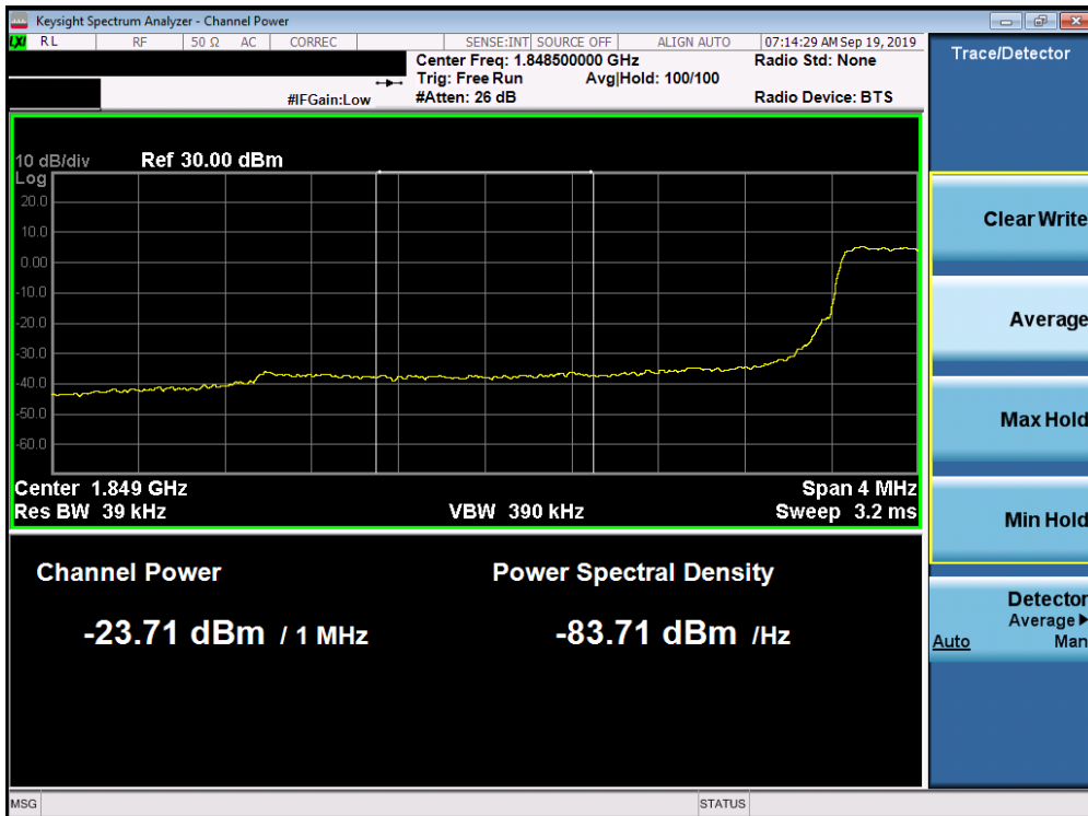
Plot 7-308. Lower Extended Band Edge Plot (Band 25/2 - 3.0MHz QPSK - Full RB Configuration)
