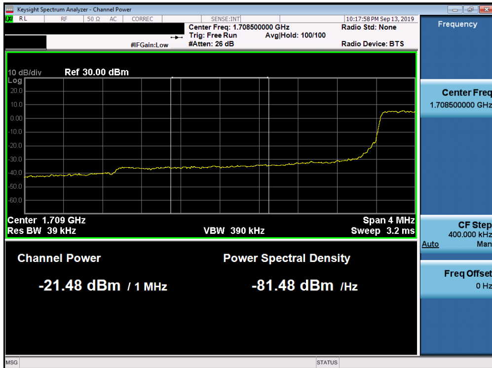
Plot 7-272. Lower Extended Band Edge Plot (Band 66/4 - 3.0MHz QPSK - Full RB Configuration)
