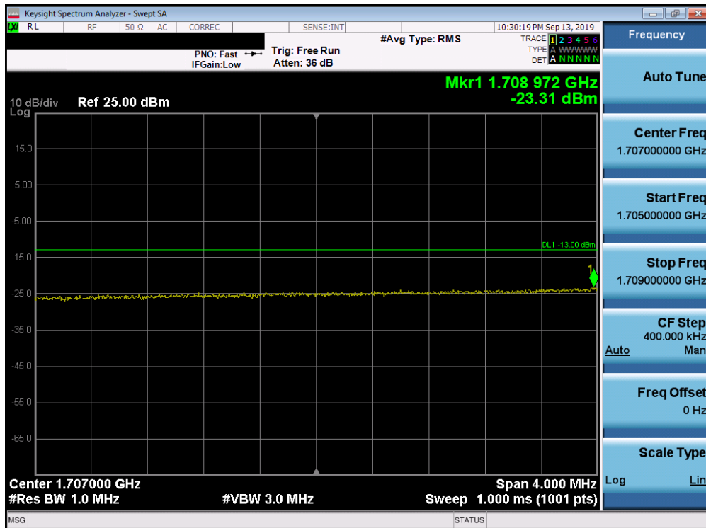
Plot 7-296. Lower Extended Band Edge Plot (Band 66/4 - 20.0MHz QPSK - Full RB Configuration)
