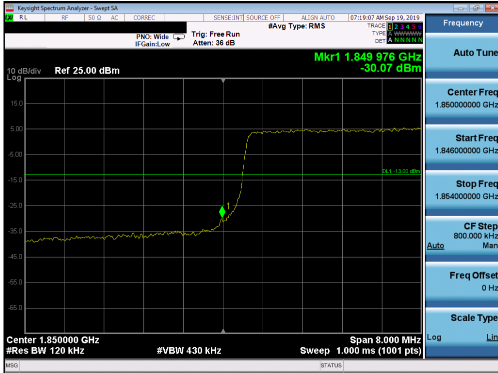
Plot 7-319. Lower Band Edge Plot (Band 25/2 - 10.0MHz QPSK - Full RB Configuration)
