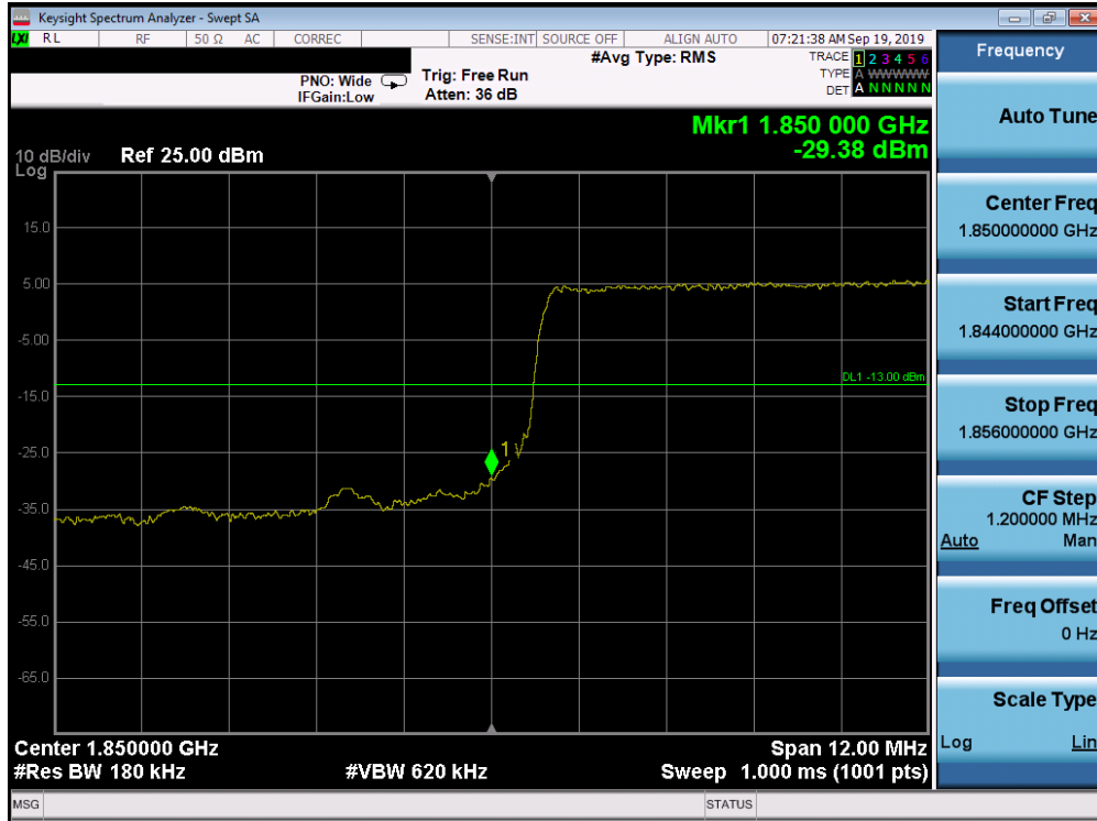
Plot 7-325. Lower Band Edge Plot (Band 25/2 - 15.0MHz QPSK - Full RB Configuration)
