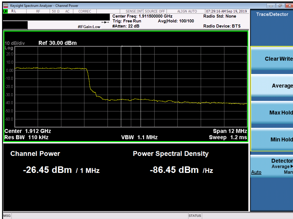
Plot 7-328. Upper Extended Band Edge Plot (Band 2 - 15.0MHz QPSK - Full RB Configuration)
