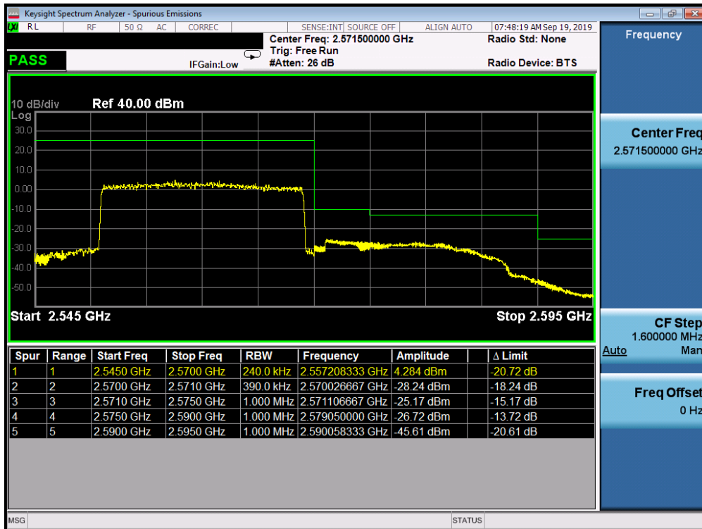
Plot 7-352. Upper ACP Plot (Band 7 - 20.0MHz QPSK - Full RB Configuration)
