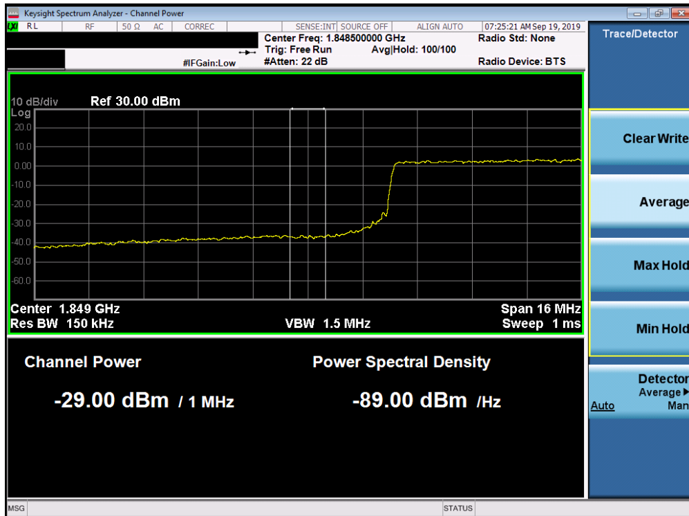
Plot 7-332. Lower Extended Band Edge Plot (Band 25/2 - 20.0MHz QPSK - Full RB Configuration)
