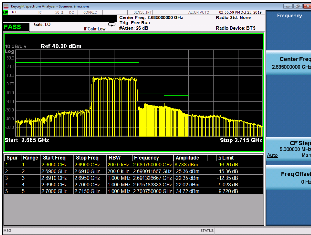
Plot 7-356. Upper ACP Plot (Band 41 - 10.0MHz QPSK - Full RB Configuration)
