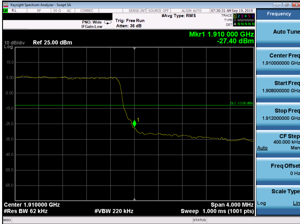
Plot 7-315. Upper Band Edge Plot (Band 2 - 5.0MHz QPSK - Full RB Configuration)
