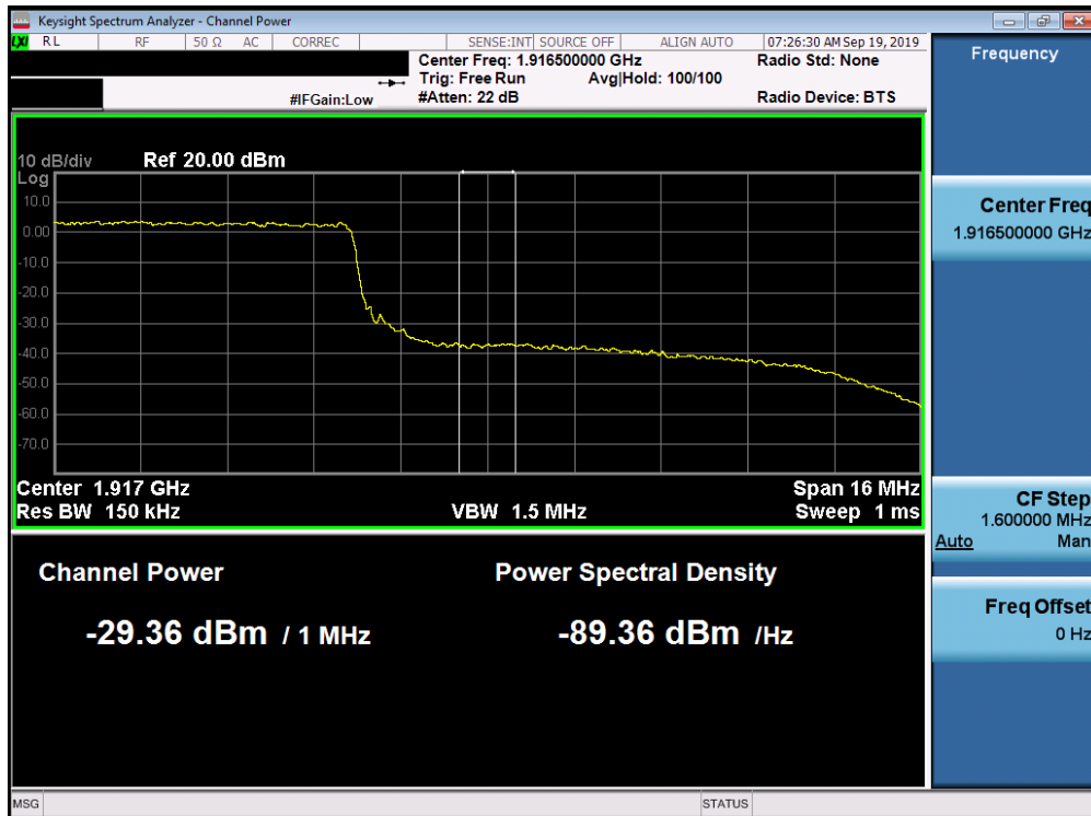
Plot 7-336. Upper Extended Band Edge Plot (Band 25 - 20.0MHz QPSK - Full RB Configuration)
