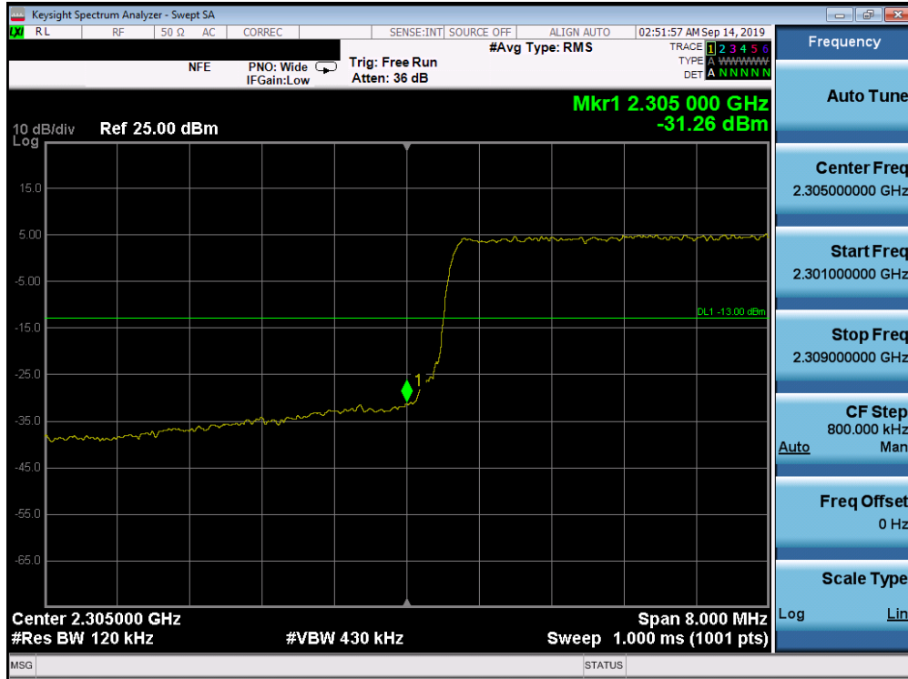
Plot 7-341. Lower Band Edge Plot (Band 30 - 10.0MHz QPSK - Full RB Configuration)
