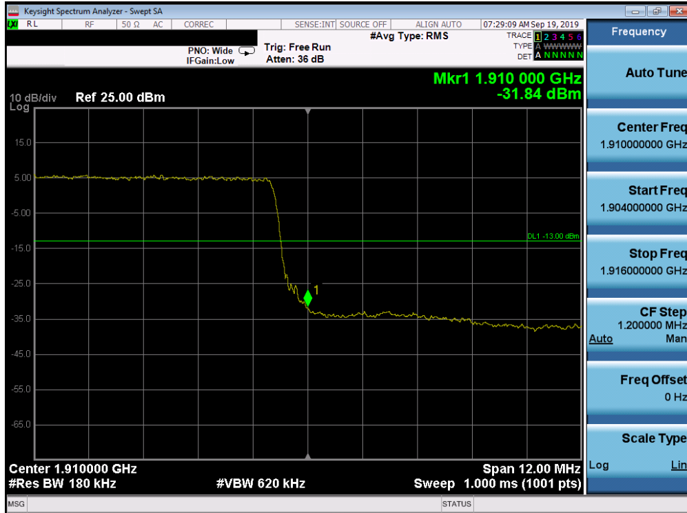
Plot 7-327. Upper Band Edge Plot (Band 2 - 15.0MHz QPSK - Full RB Configuration)
