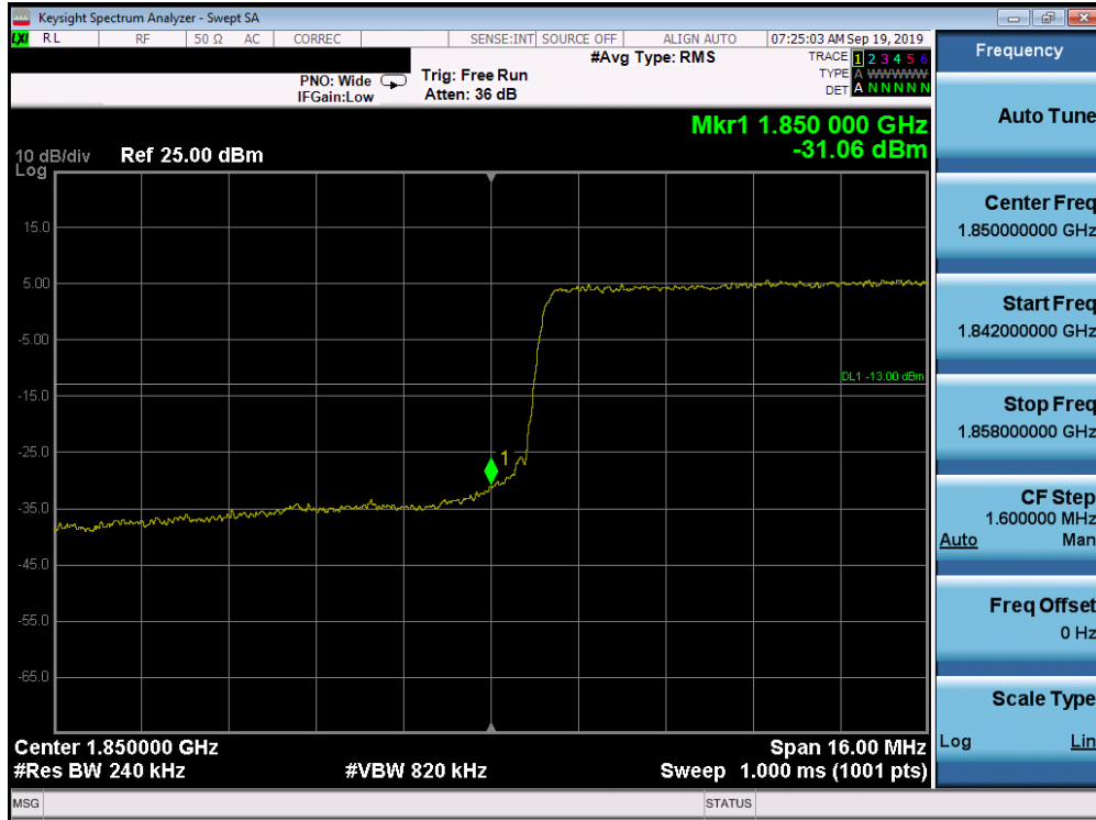
Plot 7-331. Lower Band Edge Plot (Band 25/2 - 20.0MHz QPSK - Full RB Configuration)
