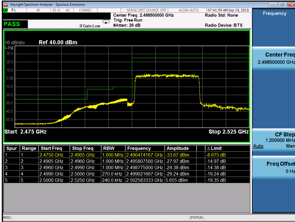
Plot 7-349. Lower ACP Plot (Band 7 - 15.0MHz QPSK - Full RB Configuration)
