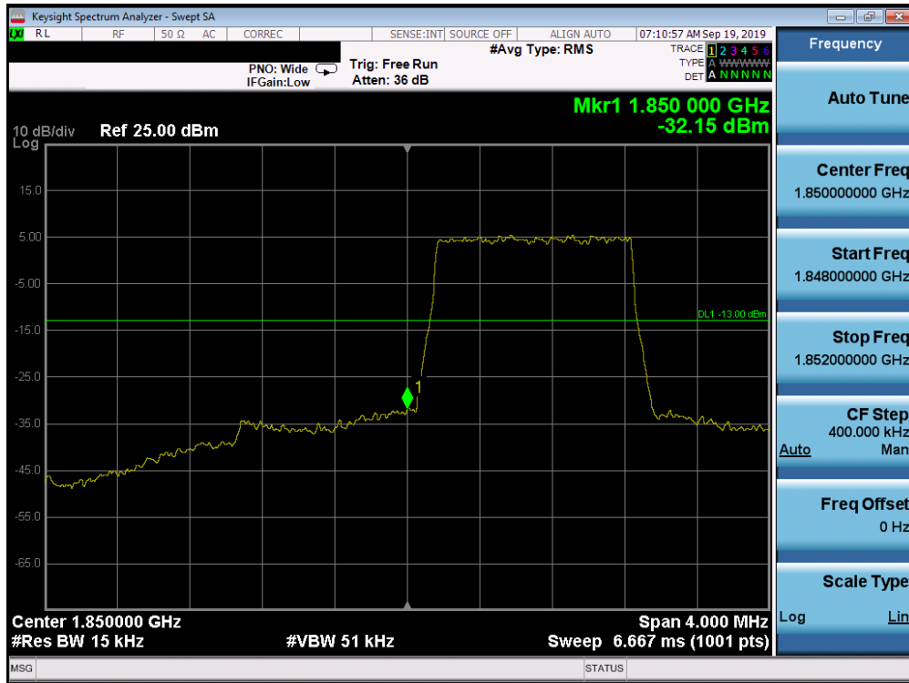
Plot 7-301. Lower Band Edge Plot (Band 25/2 - 1.4MHz QPSK - Full RB Configuration)
