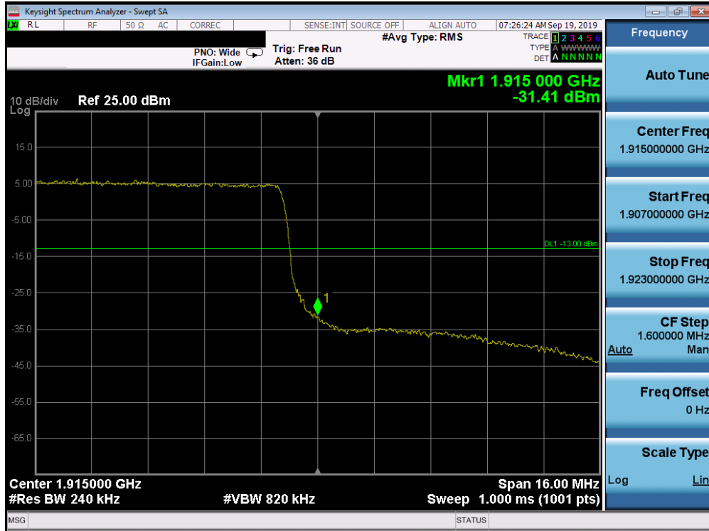
Plot 7-335. Upper Band Edge Plot (Band 25 - 20.0MHz QPSK - Full RB Configuration)
