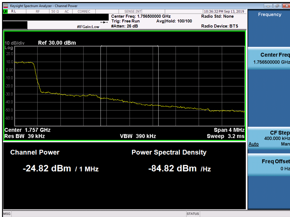
Plot 7-268. Upper Extended Band Edge Plot (Band 4 - 1.4MHz QPSK - Full RB Configuration)
