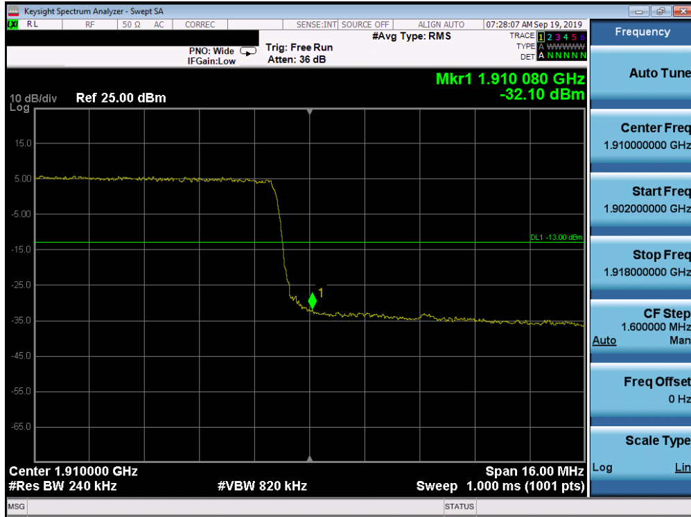
Plot 7-333. Upper Band Edge Plot (Band 2 - 20.0MHz QPSK - Full RB Configuration)
