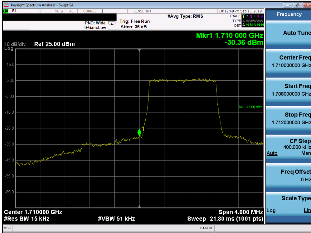
Plot 7-265. Lower Band Edge Plot (Band 66/4 - 1.4MHz QPSK - Full RB Configuration)
