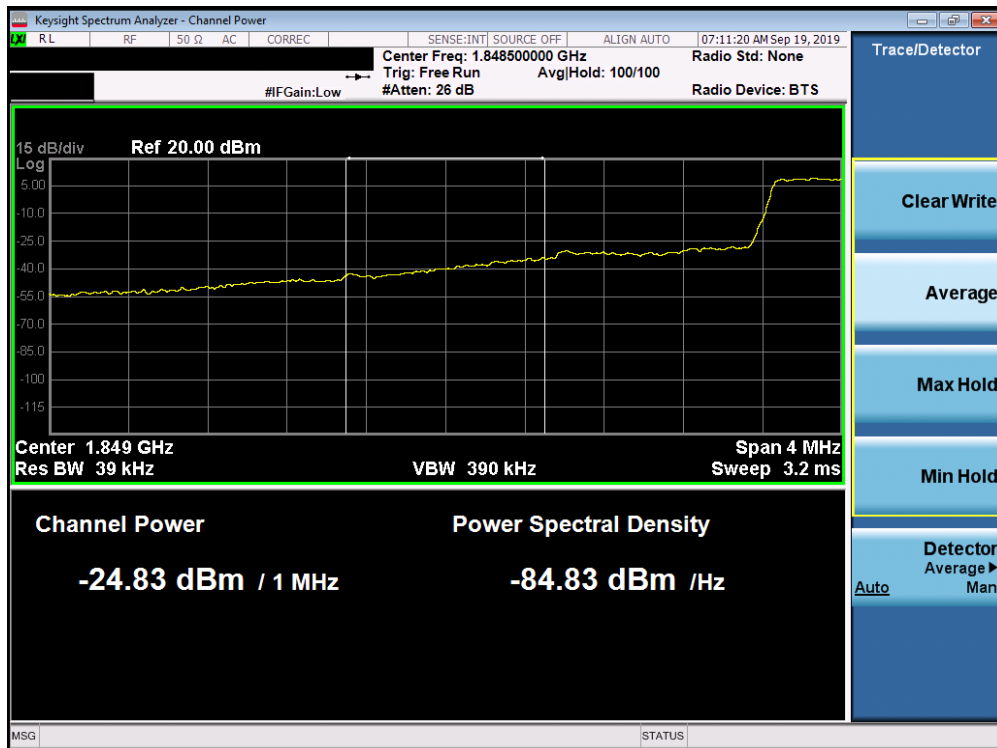
Plot 7-302. Lower Extended Band Edge Plot (Band 25/2 - 1.4MHz QPSK - Full RB Configuration)
