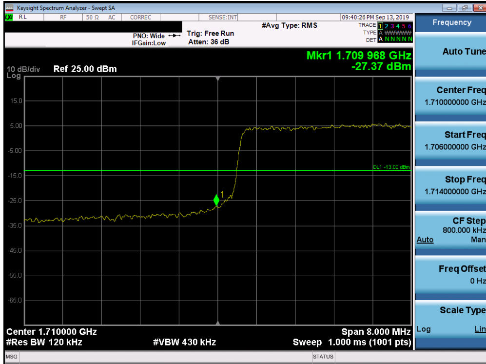
Plot 7-283. Lower Band Edge Plot (Band 66/4 - 10.0MHz QPSK - Full RB Configuration)
