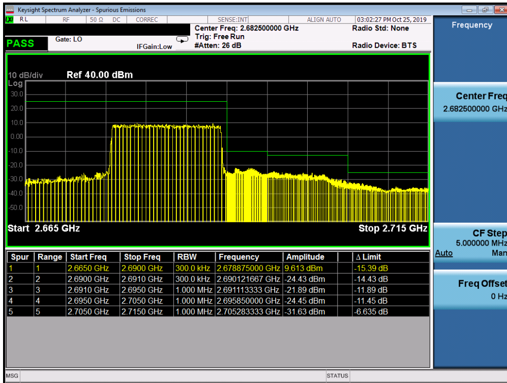
Plot 7-358. Upper ACP Plot (Band 41 - 15.0MHz QPSK - Full RB Configuration)
