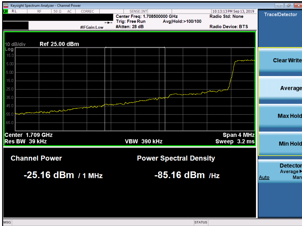
Plot 7-266. Lower Extended Band Edge Plot (Band 66/4 - 1.4MHz QPSK - Full RB Configuration)
