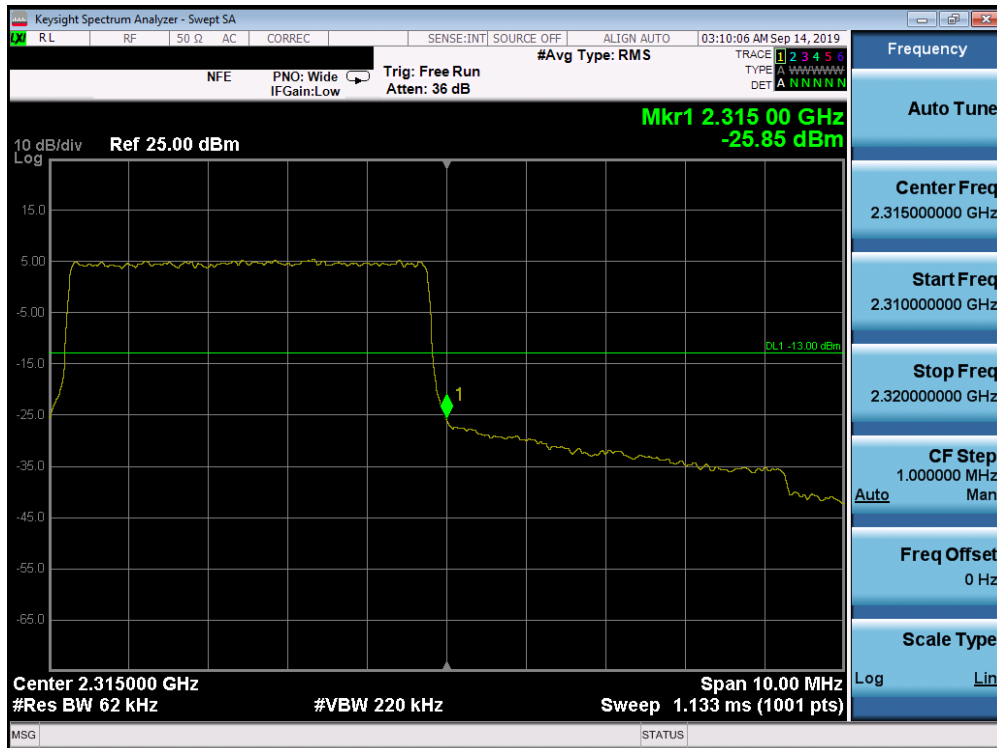
Plot 7-339. Upper Band Edge Plot (Band 30 - 5.0MHz QPSK - Full RB Configuration)
