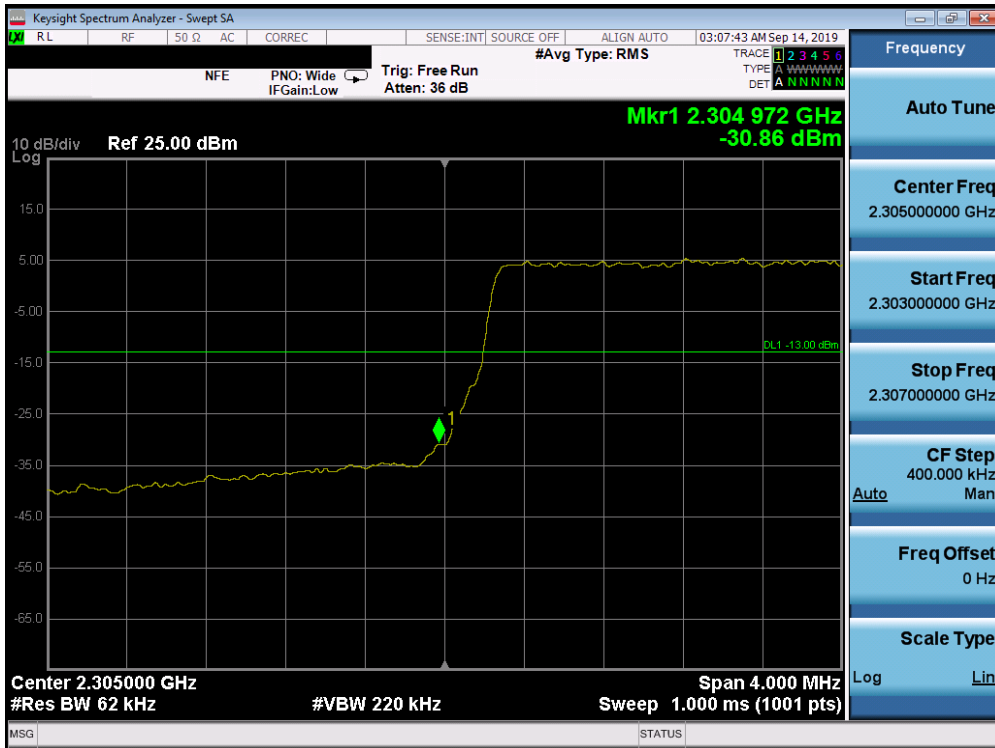
Plot 7-337. Lower Band Edge Plot (Band 30 - 5.0MHz QPSK - Full RB Configuration)
