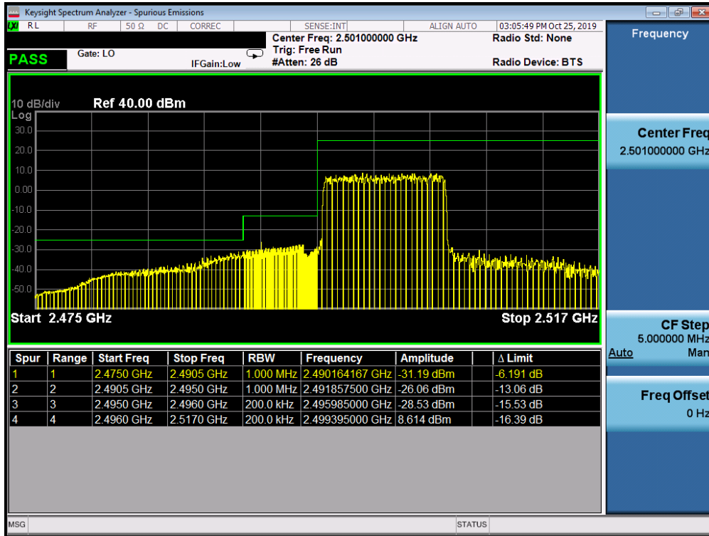
Plot 7-355. Lower ACP Plot at 2496 MHz (Band 41 - 10.0MHz QPSK - Full RB Configuration)
