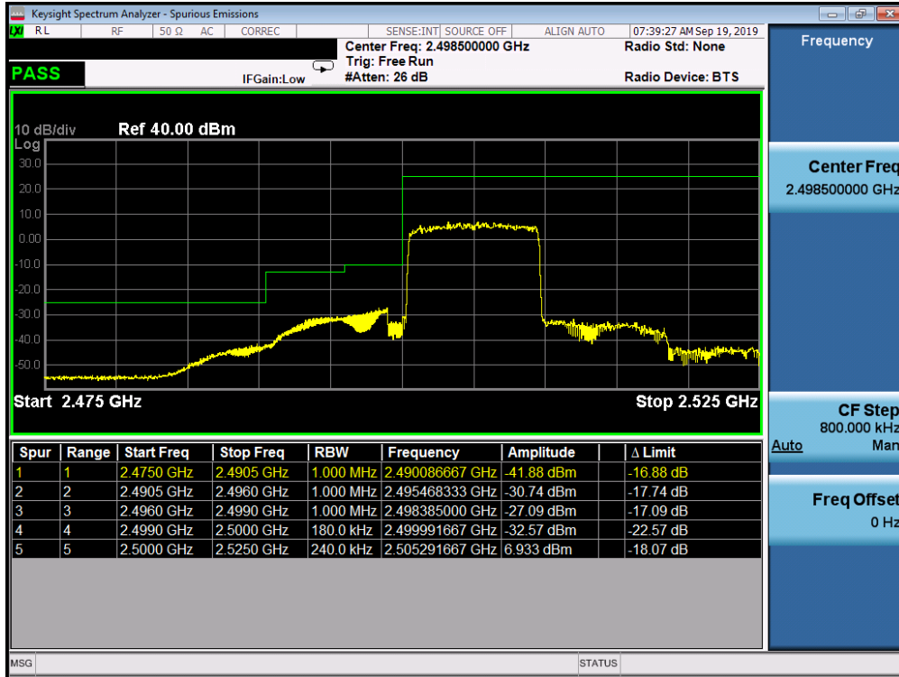
Plot 7-347. Lower ACP Plot (Band 7 - 10.0MHz QPSK - Full RB Configuration)
