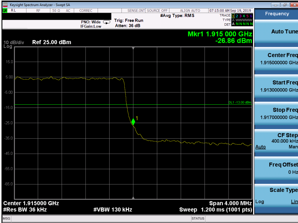
Plot 7-311. Upper Band Edge Plot (Band 25 - 3.0MHz QPSK - Full RB Configuration)
