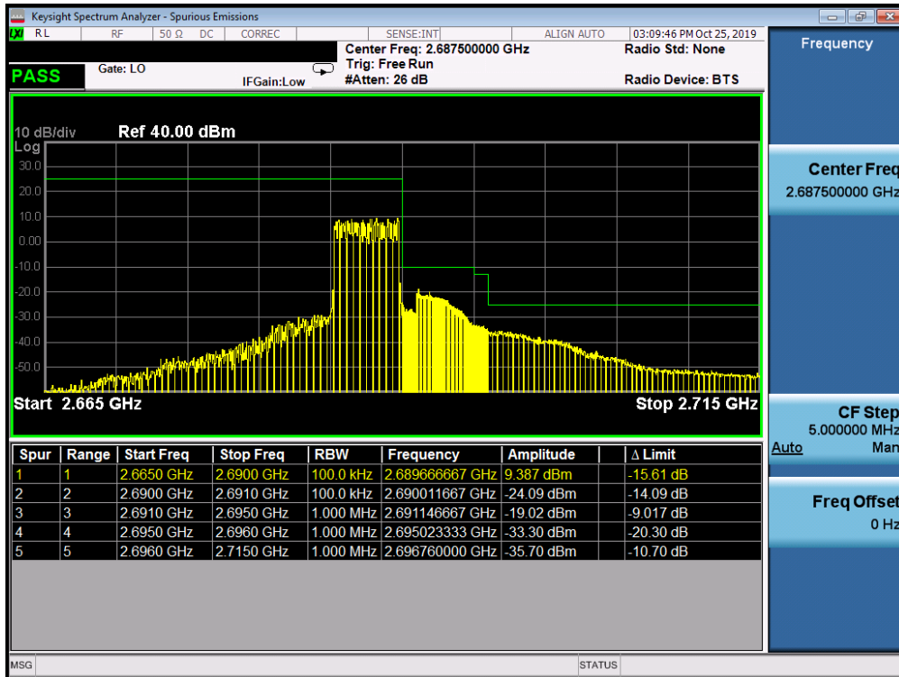
Plot 7-354. Upper ACP Plot (Band 41 - 5.0MHz QPSK - Full RB Configuration)
