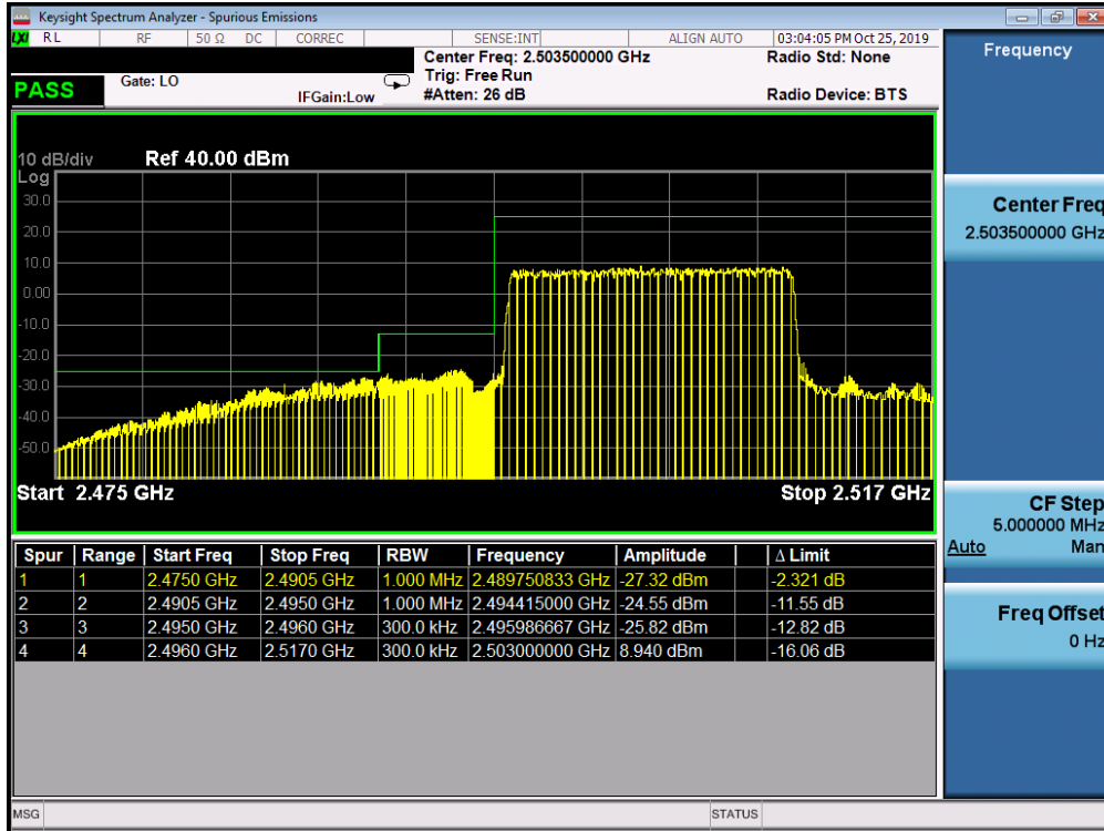
Plot 7-357. Lower ACP Plot at 2496 MHz (Band 41 - 15.0MHz QPSK - Full RB Configuration)
