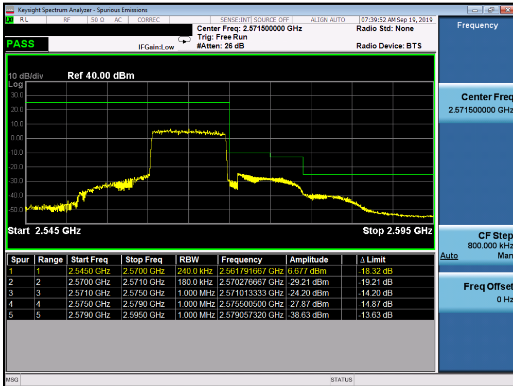
Plot 7-348. Higher ACP Plot (Band 7 - 10.0MHz QPSK - Full RB Configuration)
