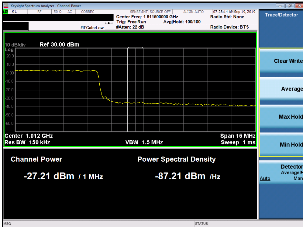
Plot 7-334. Upper Extended Band Edge Plot (Band 2 - 20.0MHz QPSK - Full RB Configuration)
