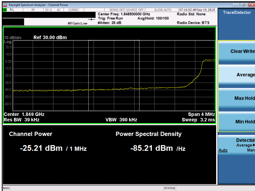
Plot 7-314. Lower Extended Band Edge Plot (Band 25/2 - 5.0MHz QPSK - Full RB Configuration)
