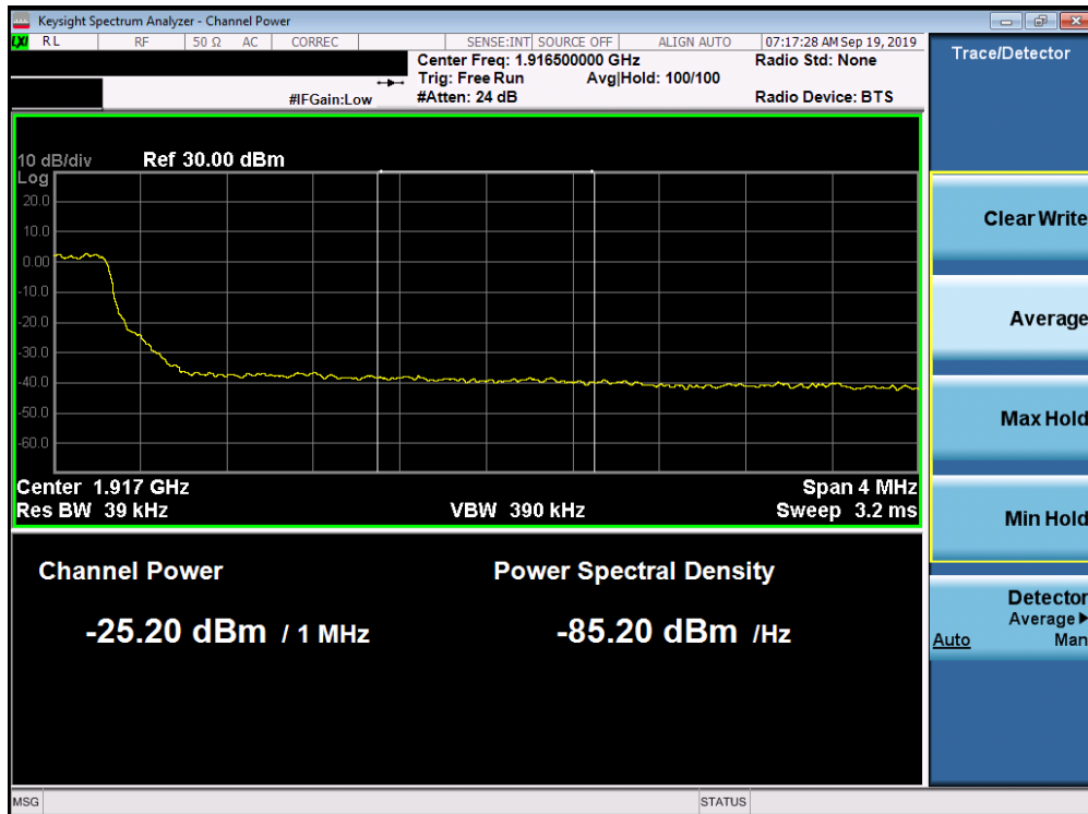
Plot 7-318. Upper Extended Band Edge Plot (Band 25 - 5.0MHz QPSK - Full RB Configuration)
