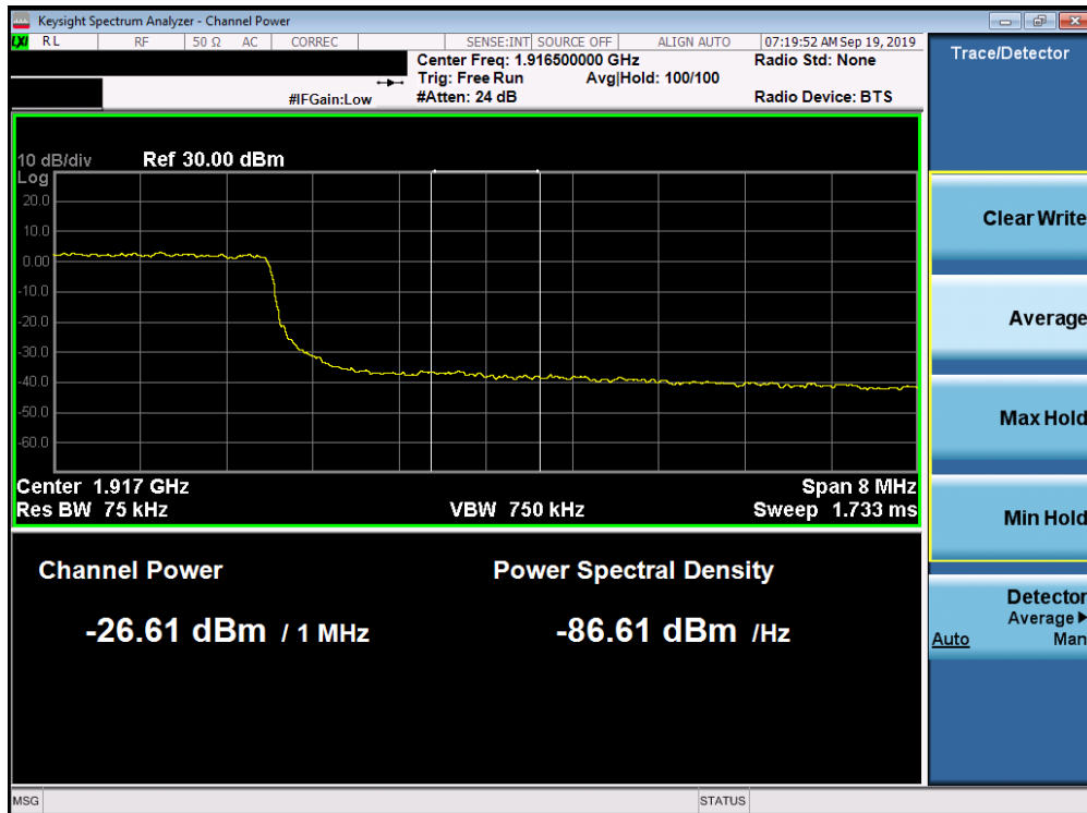
Plot 7-324. Upper Extended Band Edge Plot (Band 25 - 10.0MHz QPSK - Full RB Configuration)
