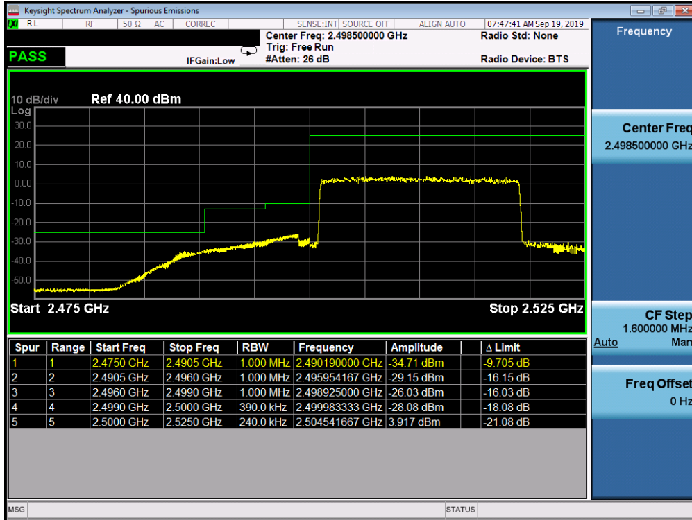
Plot 7-351. Lower ACP Plot (Band 7 - 20.0MHz QPSK - Full RB Configuration)
