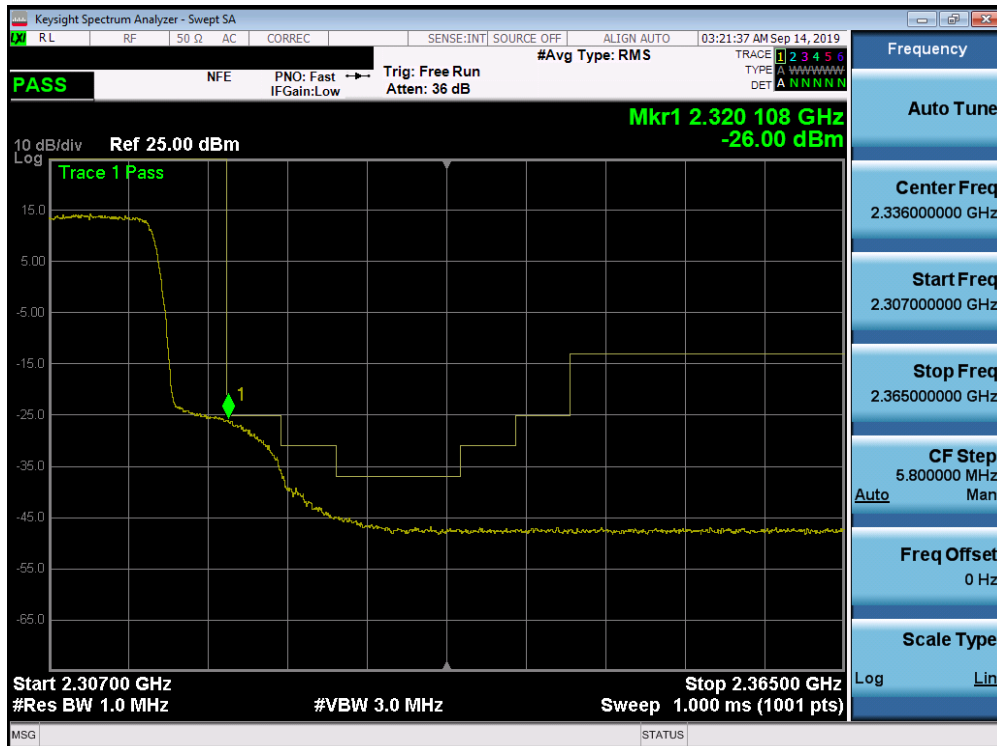
Plot 7-344. Upper Extended Band Edge Plot (Band 30 - 10.0MHz QPSK - Full RB Configuration)
