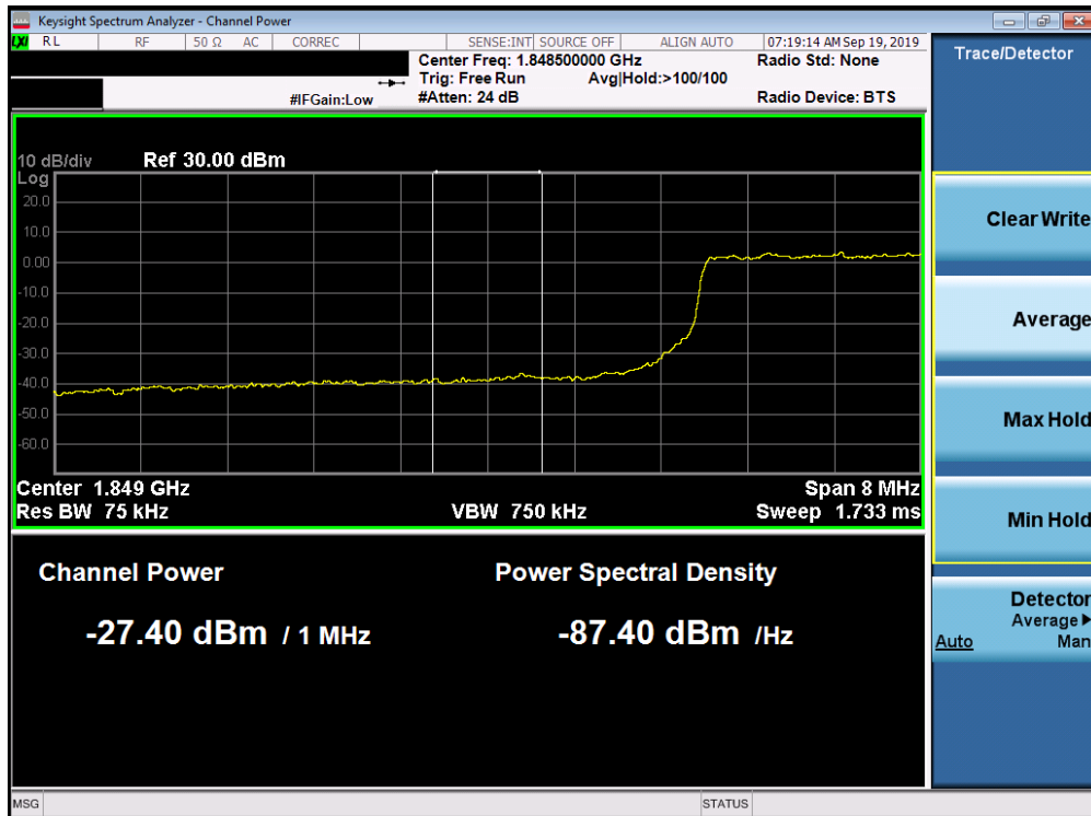
Plot 7-320. Lower Extended Band Edge Plot (Band 25/2 - 10.0MHz QPSK - Full RB Configuration)
