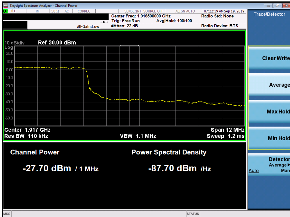
Plot 7-330. Upper Extended Band Edge Plot (Band 25 - 15.0MHz QPSK - Full RB Configuration)
