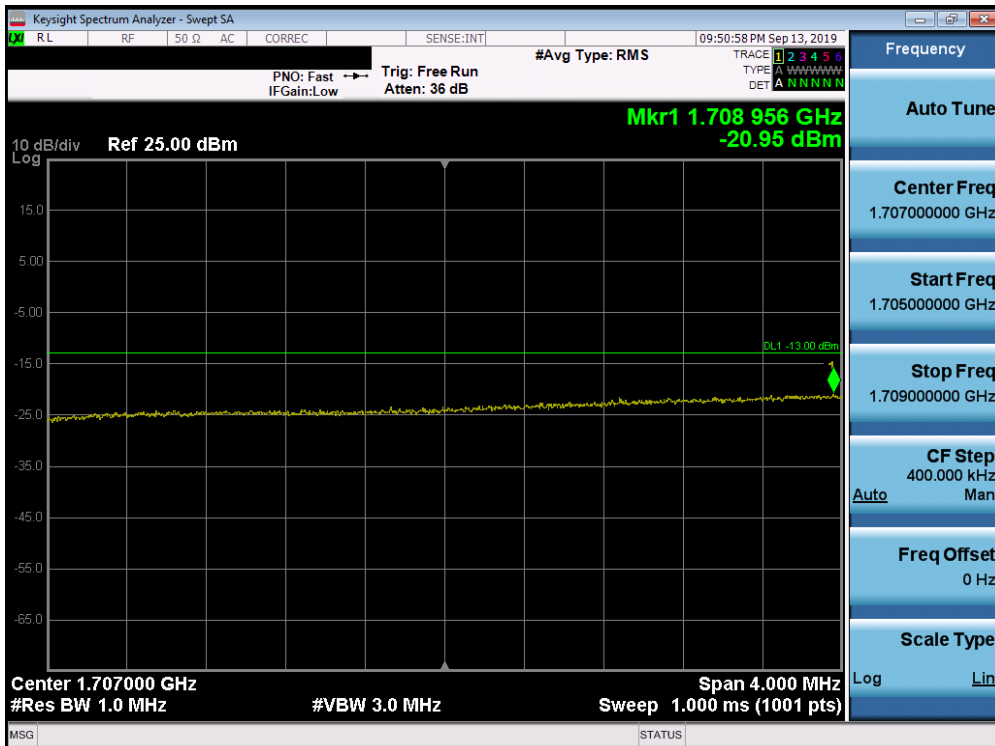
Plot 7-290. Lower Extended Band Edge Plot (Band 66/4 - 15.0MHz QPSK - Full RB Configuration)
