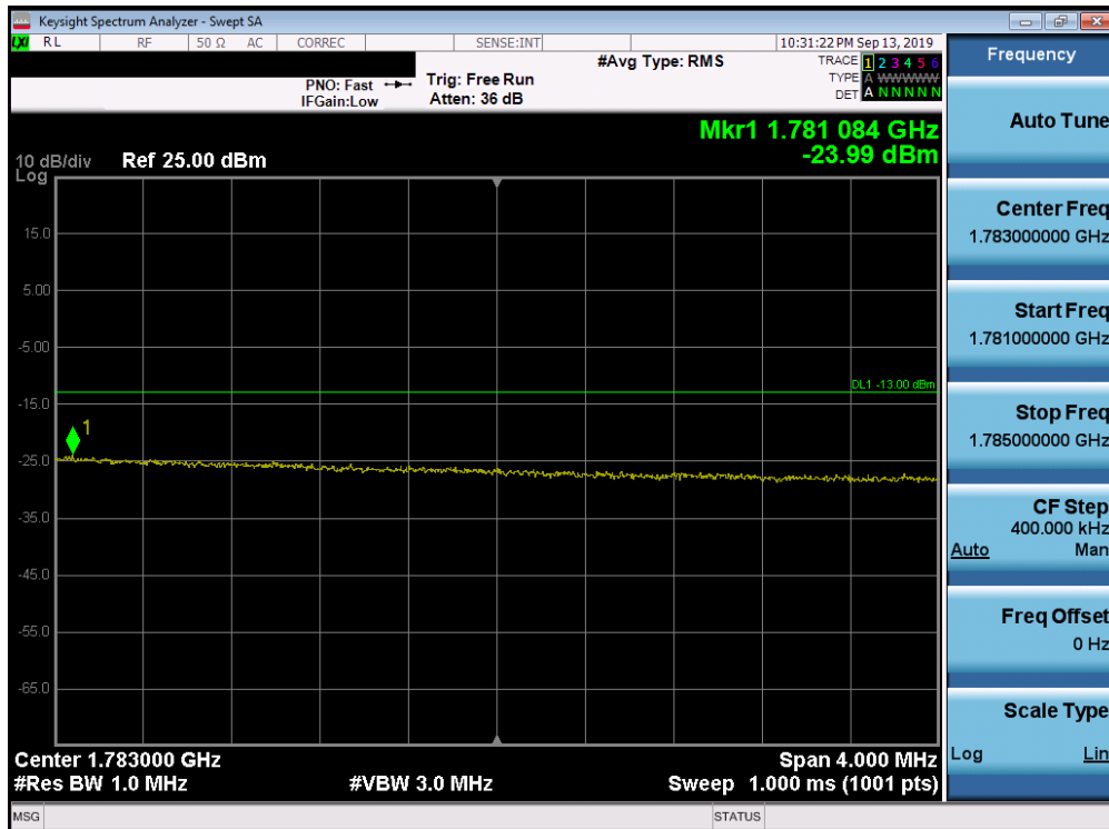
Plot 7-300. Upper Extended Band Edge Plot (Band 66 - 20.0MHz QPSK - Full RB Configuration)
