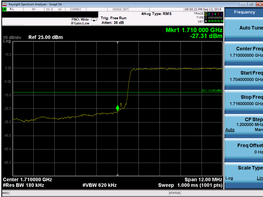
Plot 7-289. Lower Band Edge Plot (Band 66/4 - 15.0MHz QPSK - Full RB Configuration)
