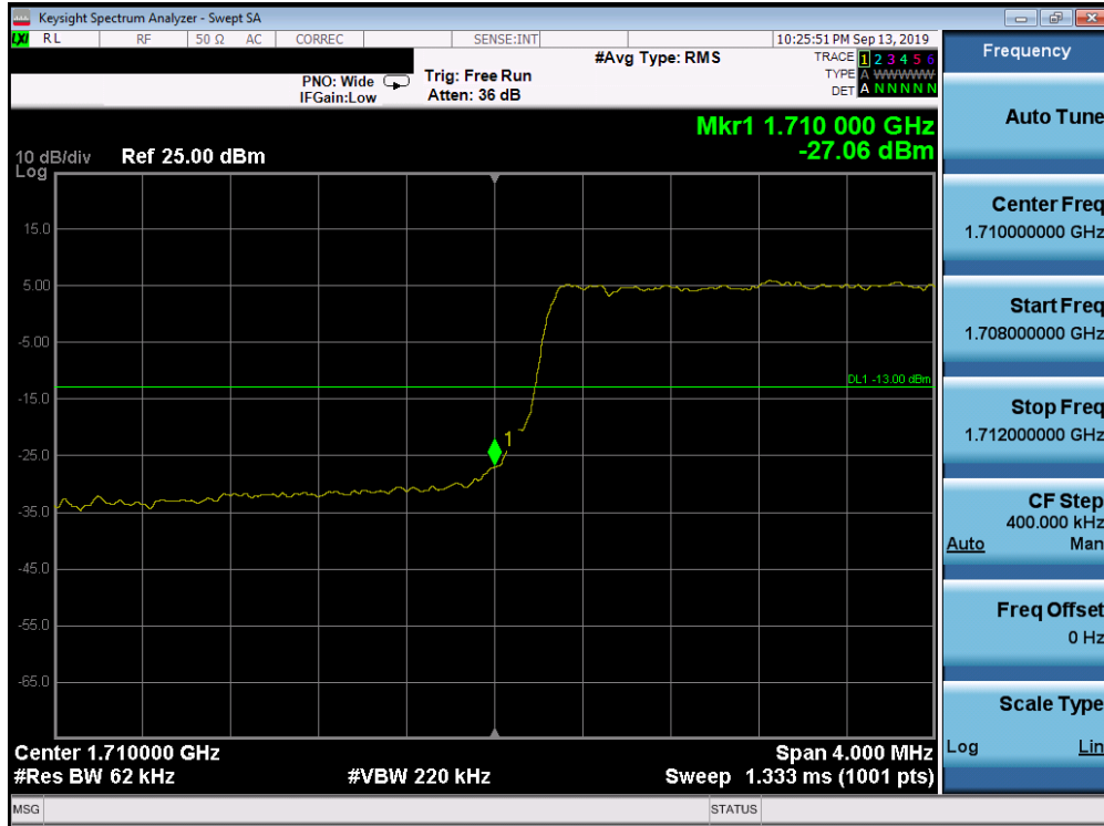
Plot 7-277. Lower Band Edge Plot (Band 66/4 - 5.0MHz QPSK - Full RB Configuration)
