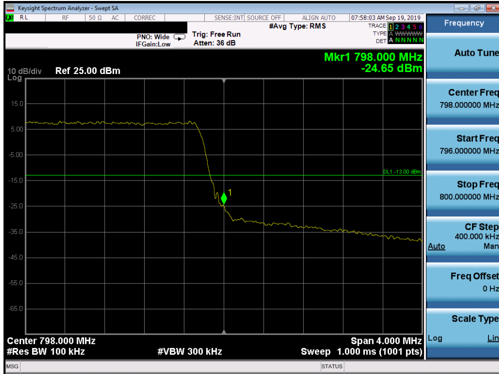
Plot 7-45. Upper Band Edge Plot (LTE Band 14, 5MHz QPSK – RB Size 25)
