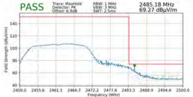
Plot 7-112. Radiated Restricted Upper Band Edge Measurement SISO ANT1 (Peak)
