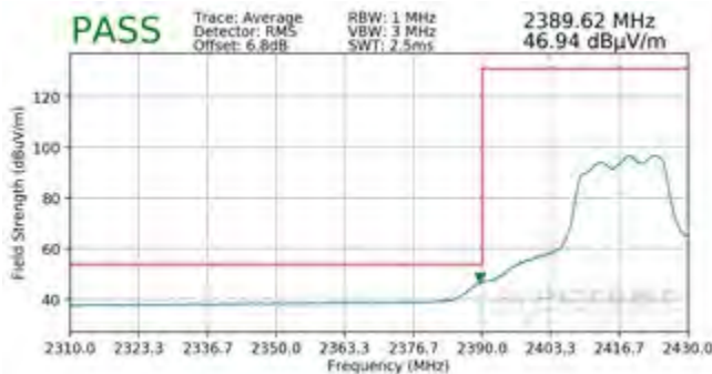
Plot 7-139. Radiated Restricted Band Edge Measurement CDD with WCP (Average)
