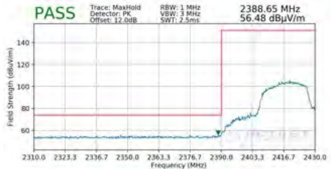
Plot 7-116. Radiated Restricted Lower Band Edge Measurement SISO ANT2 (Peak)
