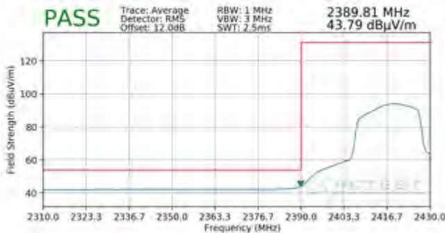
Plot 7-115. Radiated Restricted Lower Band Edge Measurement SISO ANT2 (Average)
