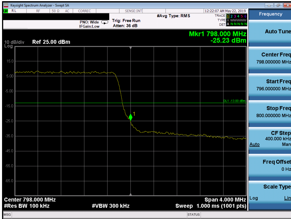
Plot 7-64. Upper Band Edge Plot (LTE Band 14, 5MHz QPSK – RB Size 25)
