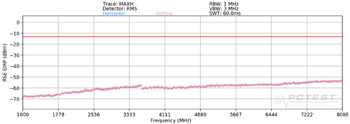
Plot 7-74. Radiated Spurious Plot above 1GHz (LTE Band 14)
