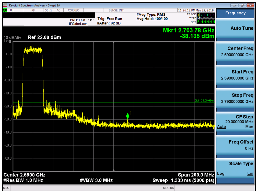
Plot 7-383. Upper ACP Plot (Band 38 - 20.0MHz QPSK - Full RB Configuration)
