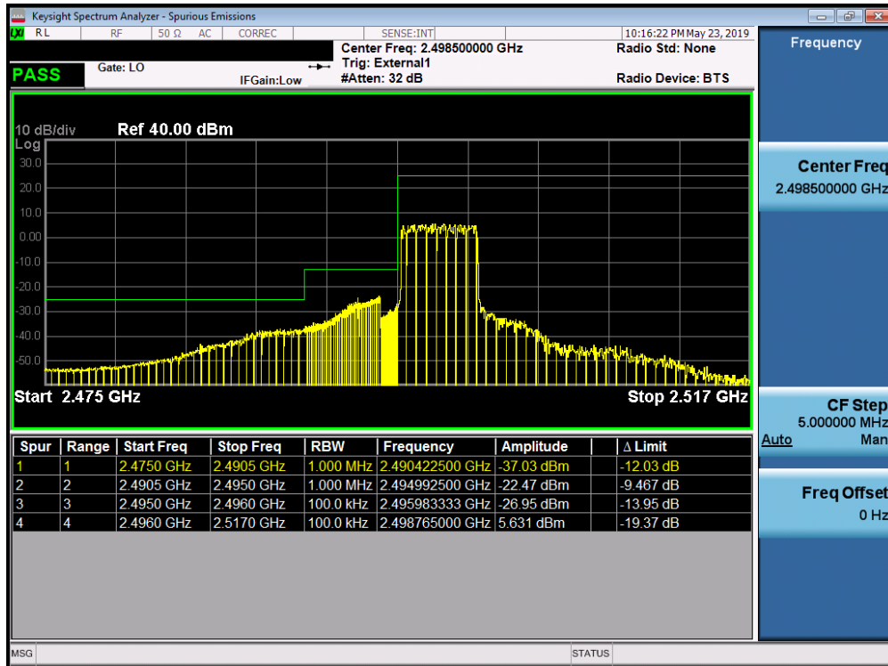
Plot 7-368. Lower ACP Plot (Band 41/38 (PC3)- 5.0MHz QPSK - Full RB Configuration)
