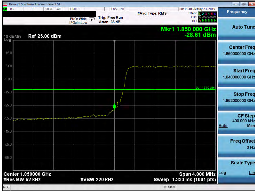
Plot 7-327. Lower Band Edge Plot (Band 25/2 - 5.0MHz QPSK - Full RB Configuration)
