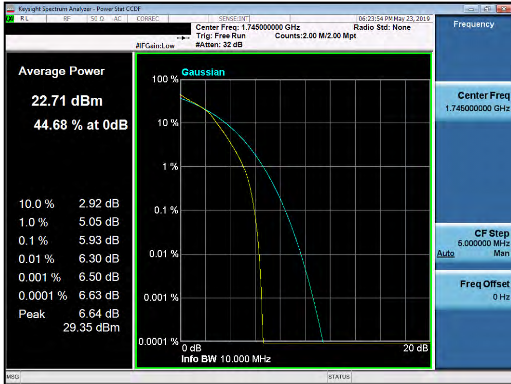
Plot 7-405. PAR Plot (Band 66/4 - 10.0MHz 16-QAM - Full RB Configuration)
