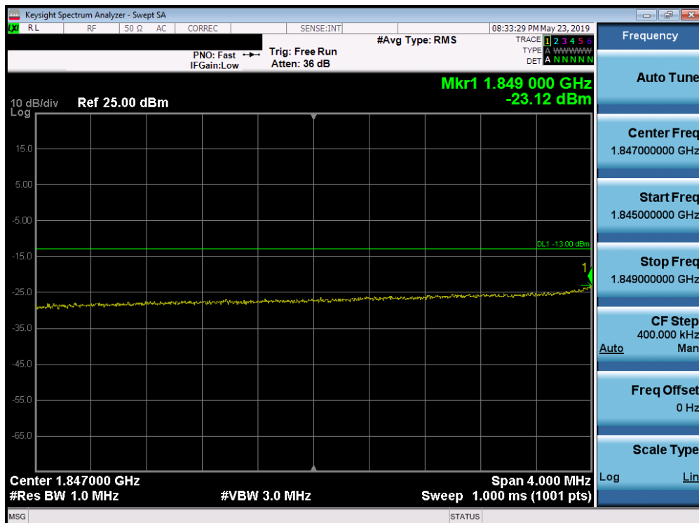
Plot 7-334. Lower Extended Band Edge Plot (Band 25/2 - 10.0MHz QPSK - Full RB Configuration)
