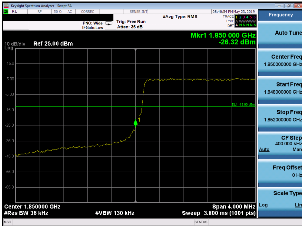
Plot 7-321. Lower Band Edge Plot (Band 25/2 - 3.0MHz QPSK - Full RB Configuration)
