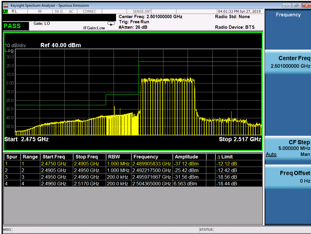
Plot 7-386. Lower ACP Plot (Band 41 (PC2)- 10.0MHz QPSK - Full RB Configuration)
