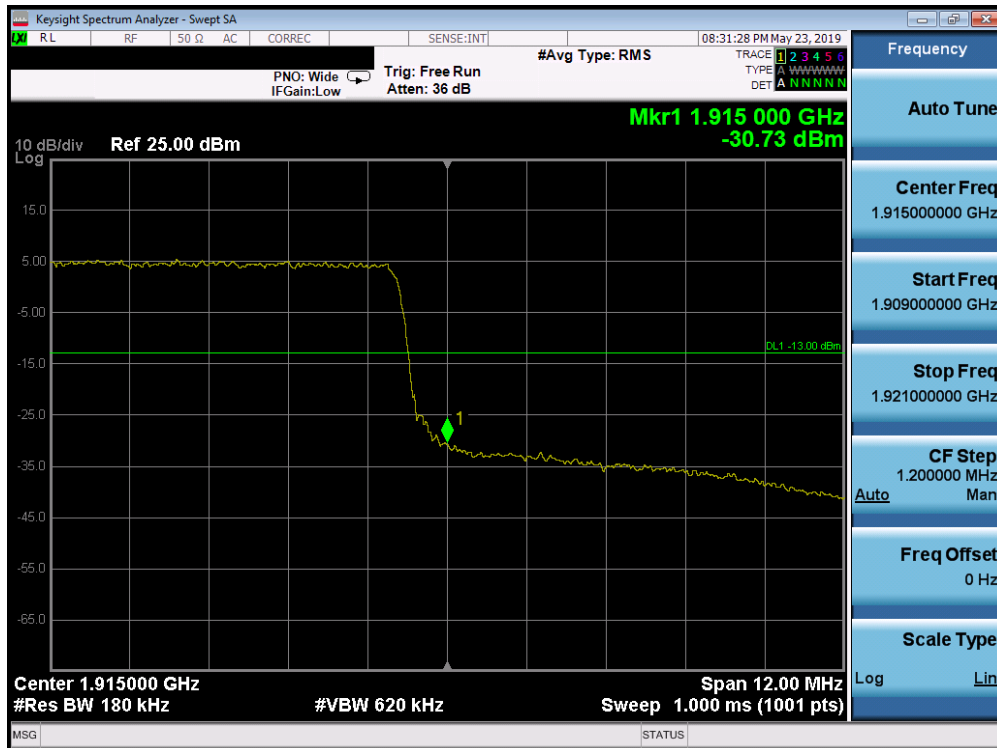
Plot 7-343. Upper Band Edge Plot (Band 25 - 15.0MHz QPSK - Full RB Configuration)
