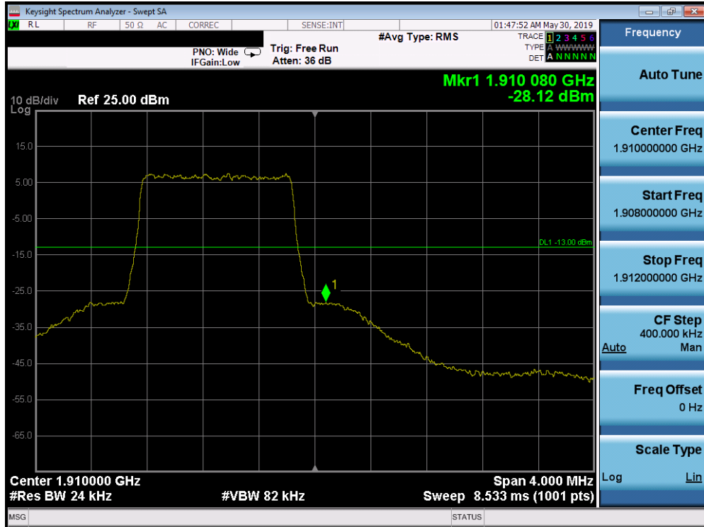
Plot 7-317. Upper Band Edge Plot (Band 2 - 1.4MHz QPSK - Full RB Configuration)
