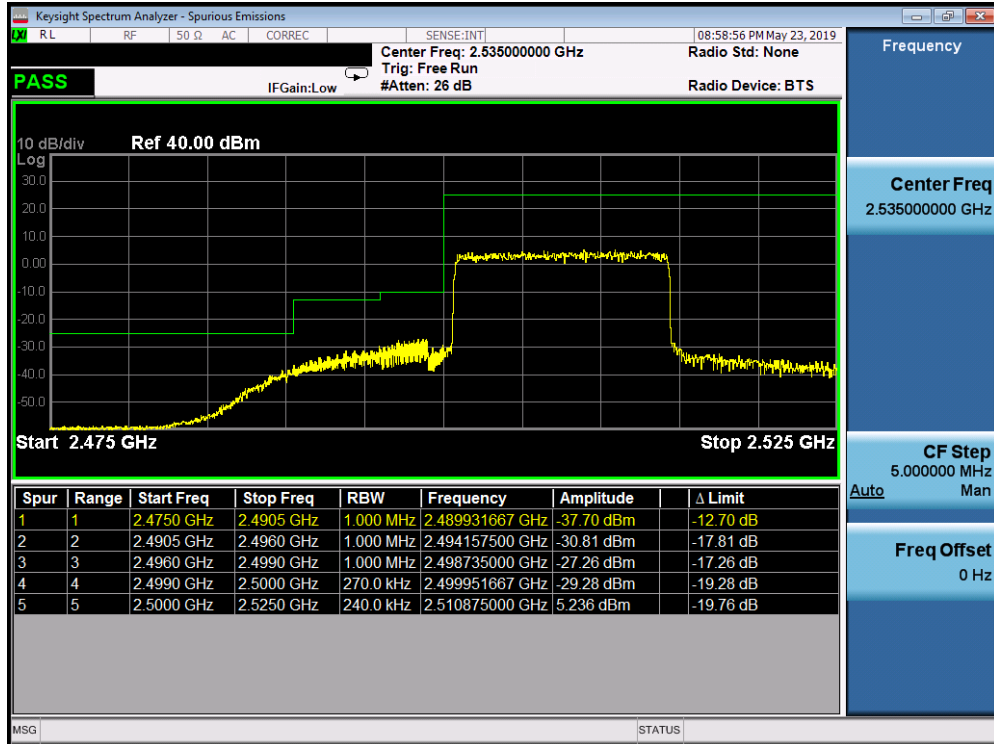
Plot 7-364. Lower ACP Plot at (Band 7 - 15.0MHz QPSK - Full RB Configuration)
