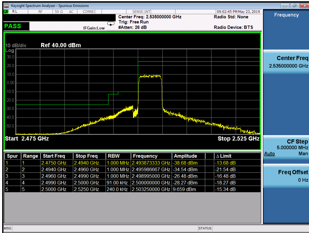
Plot 7-360. Lower ACP Plot (Band 7 - 5.0MHz QPSK - Full RB Configuration)
