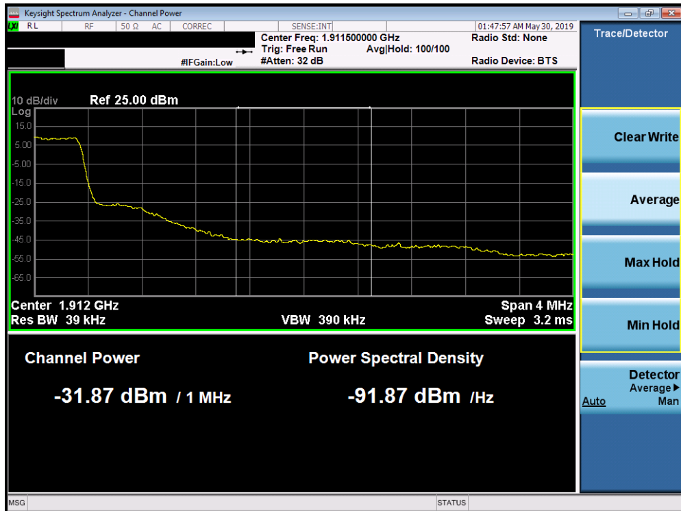
Plot 7-318. Upper Extended Band Edge Plot (Band 2 - 1.4MHz QPSK - Full RB Configuration)
