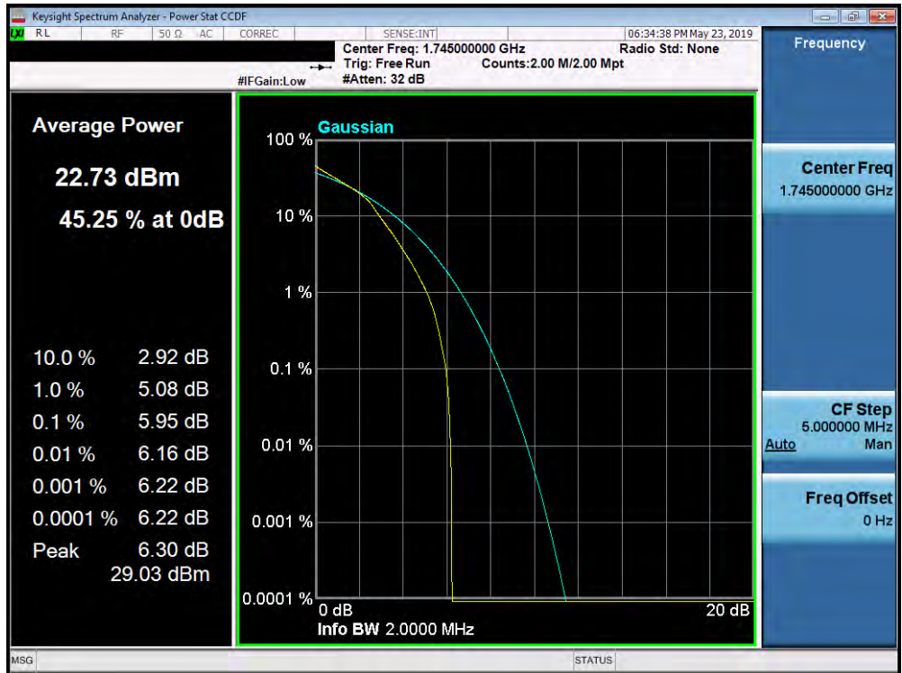
Plot 7-393. PAR Plot (Band 66/4 - 1.4MHz 16-QAM - Full RB Configuration)
