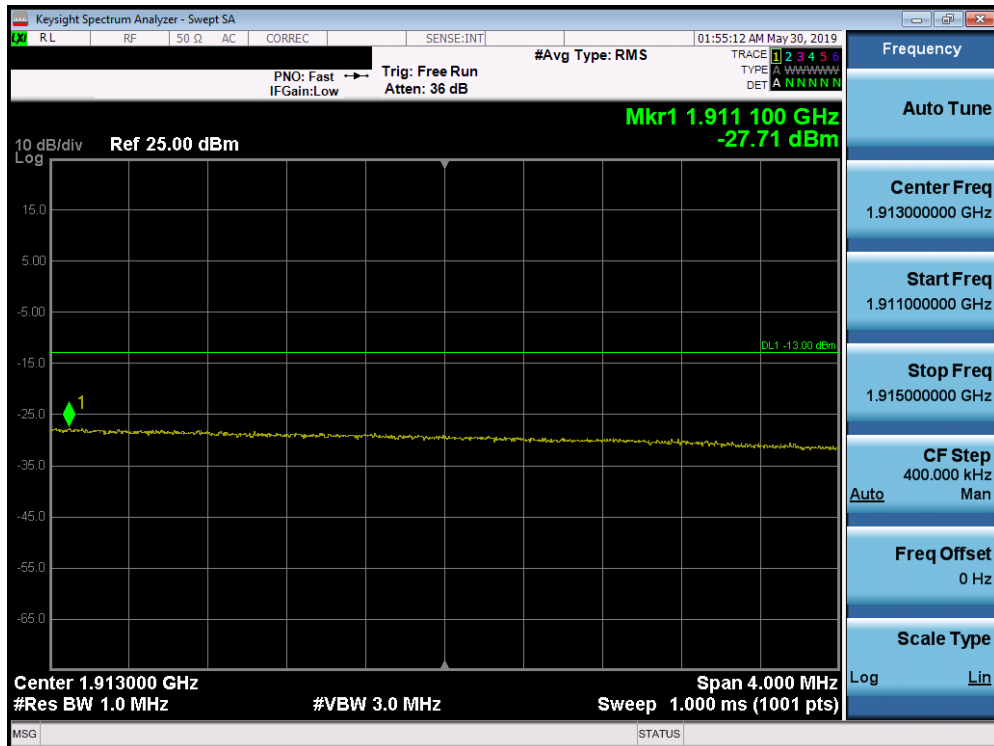
Plot 7-348. Upper Extended Band Edge Plot (Band 2 - 20.0MHz QPSK - Full RB Configuration)
