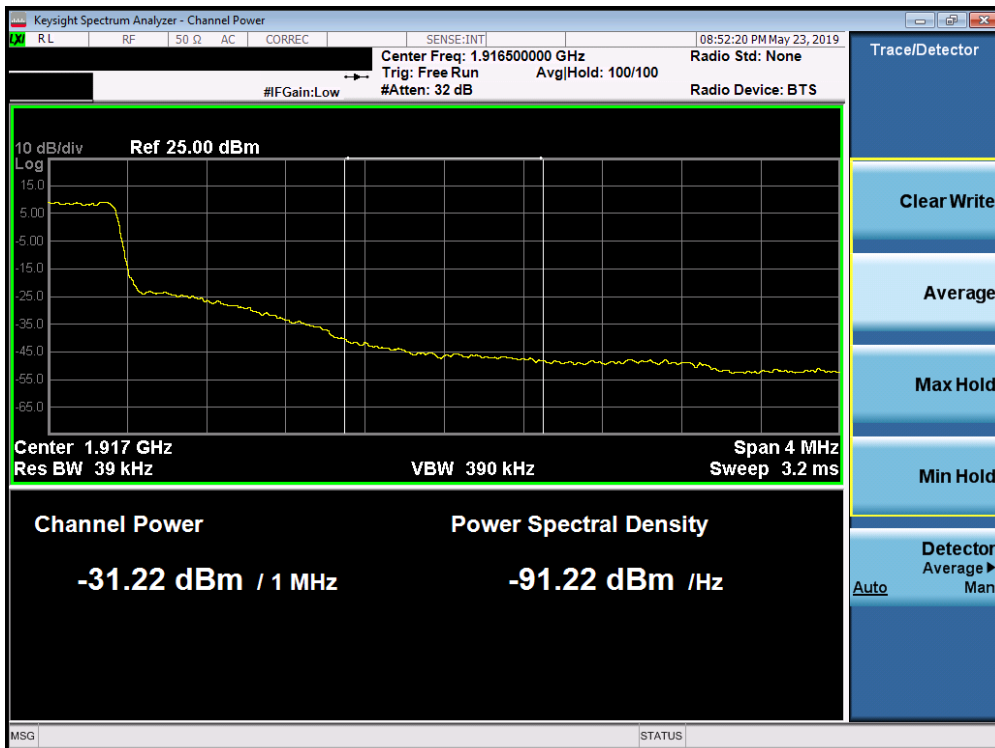
Plot 7-320. Upper Extended Band Edge Plot (Band 25 - 1.4MHz QPSK - Full RB Configuration)
