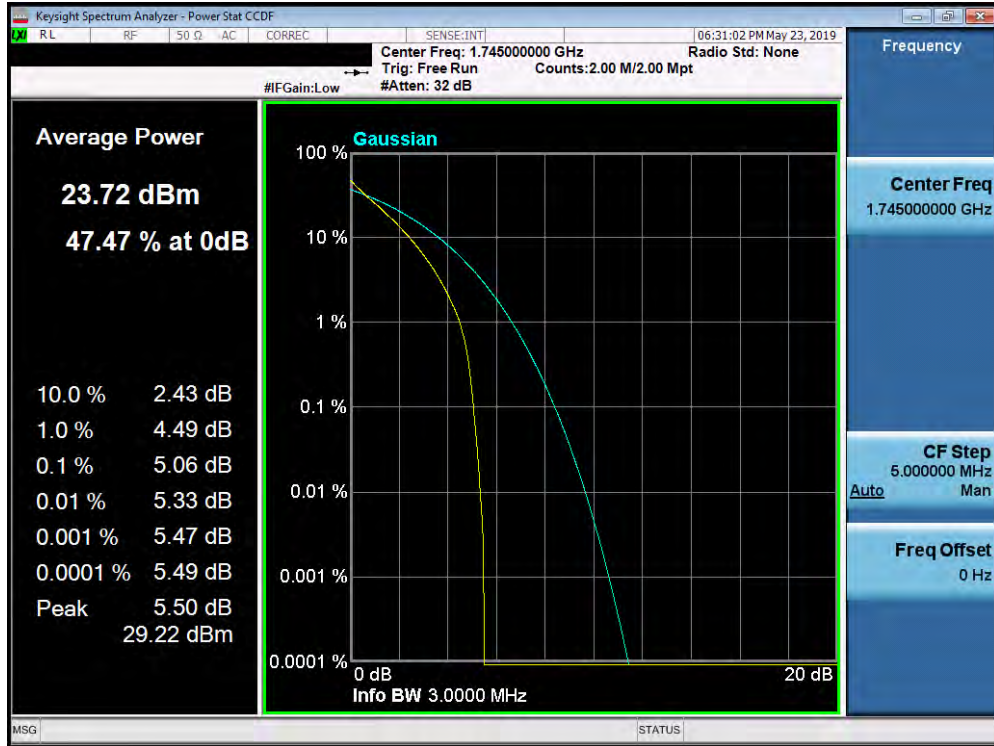
Plot 7-396. PAR Plot (Band 66/4 - 3.0MHz QPSK - Full RB Configuration)
