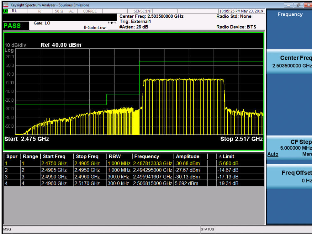
Plot 7-372. Lower ACP Plot (Band 41/38 (PC3)- 15.0MHz QPSK - Full RB Configuration)
