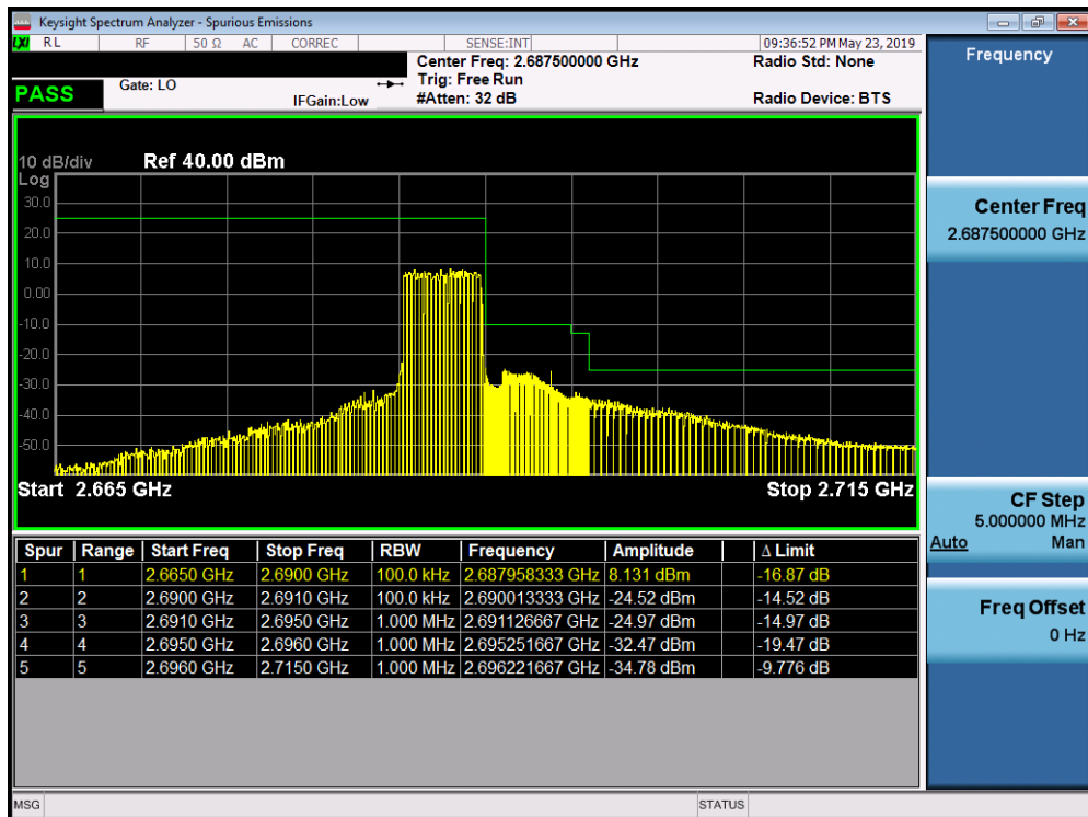
Plot 7-385. Upper ACP Plot (Band 41 (PC2)- 5.0MHz QPSK - Full RB Configuration)
