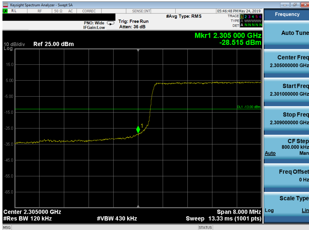
Plot 7-356. Lower Band Edge Plot (Band 30 - 10.0MHz QPSK - Full RB Configuration)
