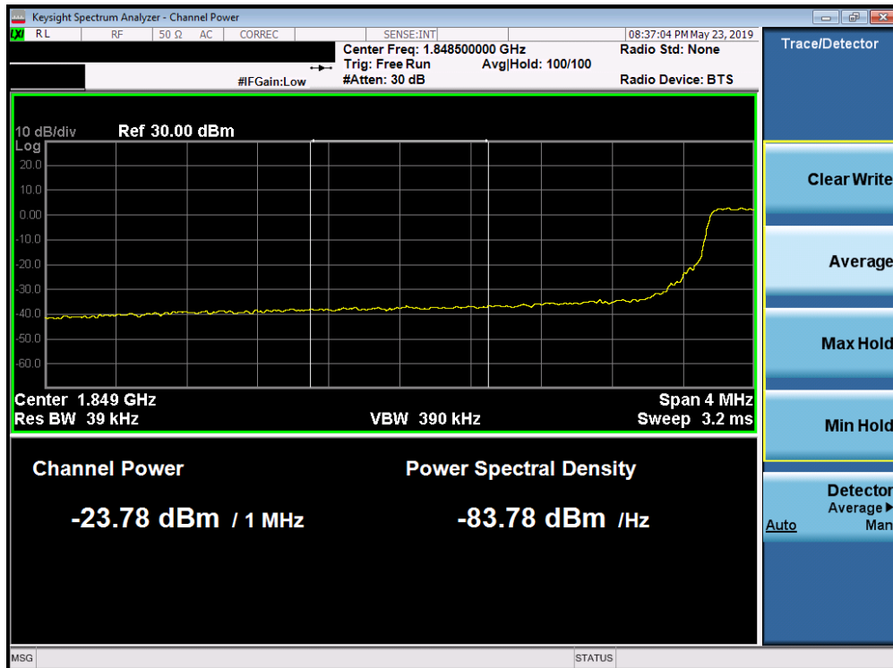
Plot 7-328. Lower Extended Band Edge Plot (Band 25/2 - 5.0MHz QPSK - Full RB Configuration)
