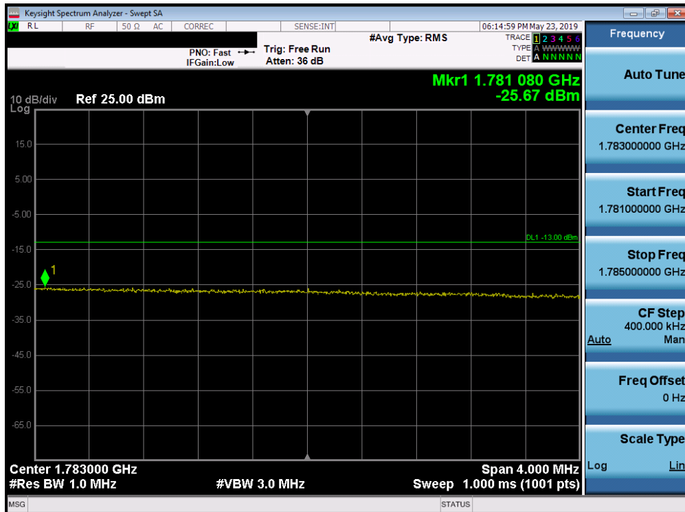
Plot 7-314. Upper Extended Band Edge Plot (Band 66 - 20.0MHz QPSK - Full RB Configuration)
