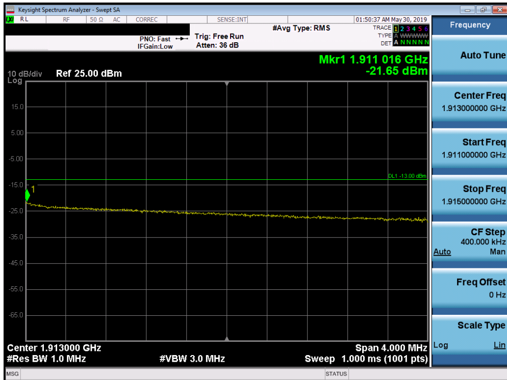
Plot 7-336. Upper Extended Band Edge Plot (Band 2 - 10.0MHz QPSK - Full RB Configuration)
