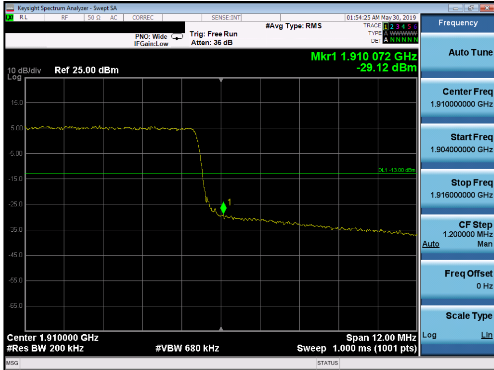
Plot 7-341. Upper Band Edge Plot (Band 2 - 15.0MHz QPSK - Full RB Configuration)
