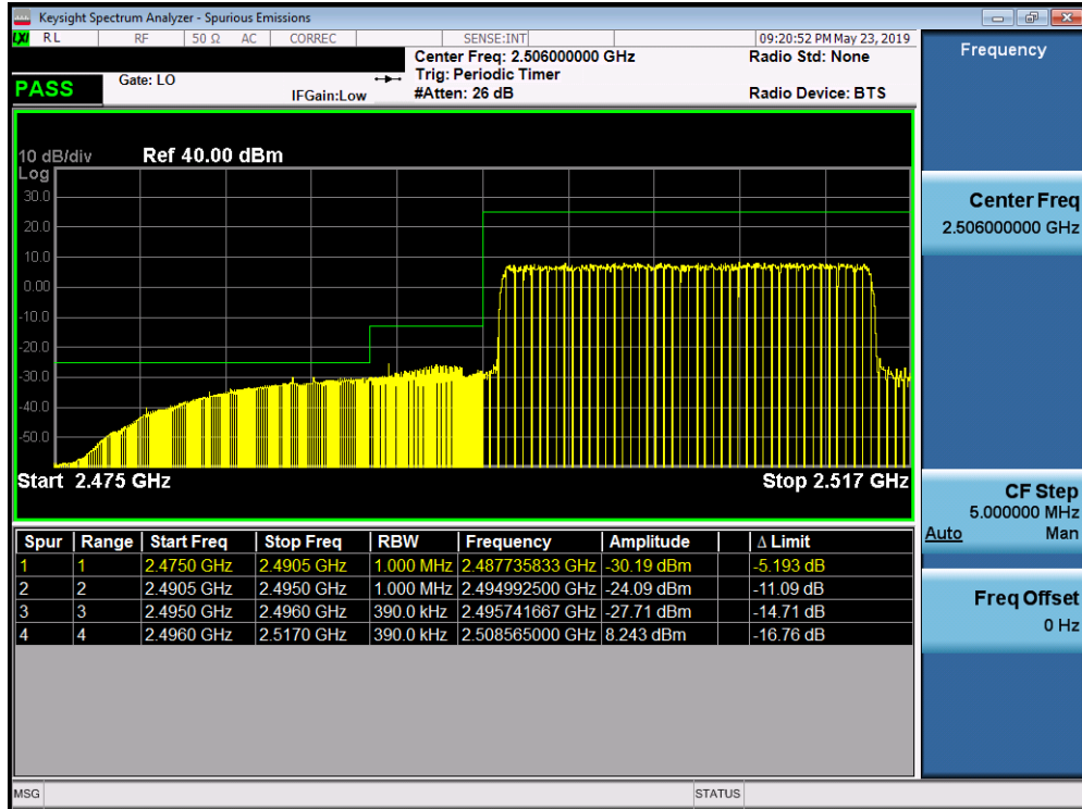
Plot 7-390. Lower ACP Plot (Band 41 (PC2)- 20.0MHz QPSK - Full RB Configuration)
