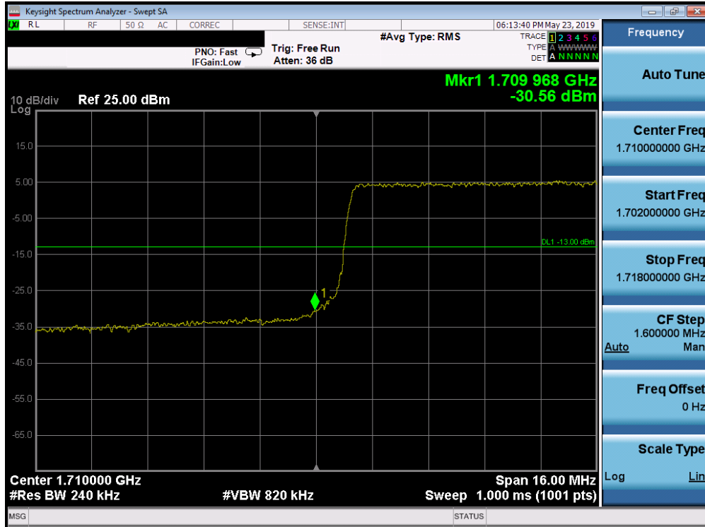
Plot 7-309. Lower Band Edge Plot (Band 66/4 - 20.0MHz QPSK - Full RB Configuration)
