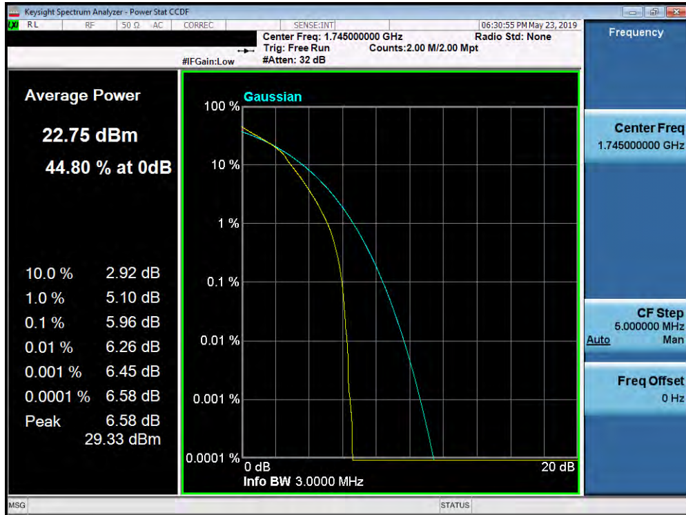
Plot 7-397. PAR Plot (Band 66/4 - 3.0MHz 16-QAM - Full RB Configuration)
