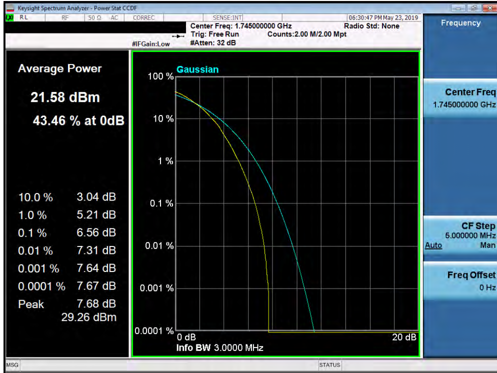
Plot 7-398. PAR Plot (Band 66/4 - 3.0MHz 64-QAM - Full RB Configuration)
