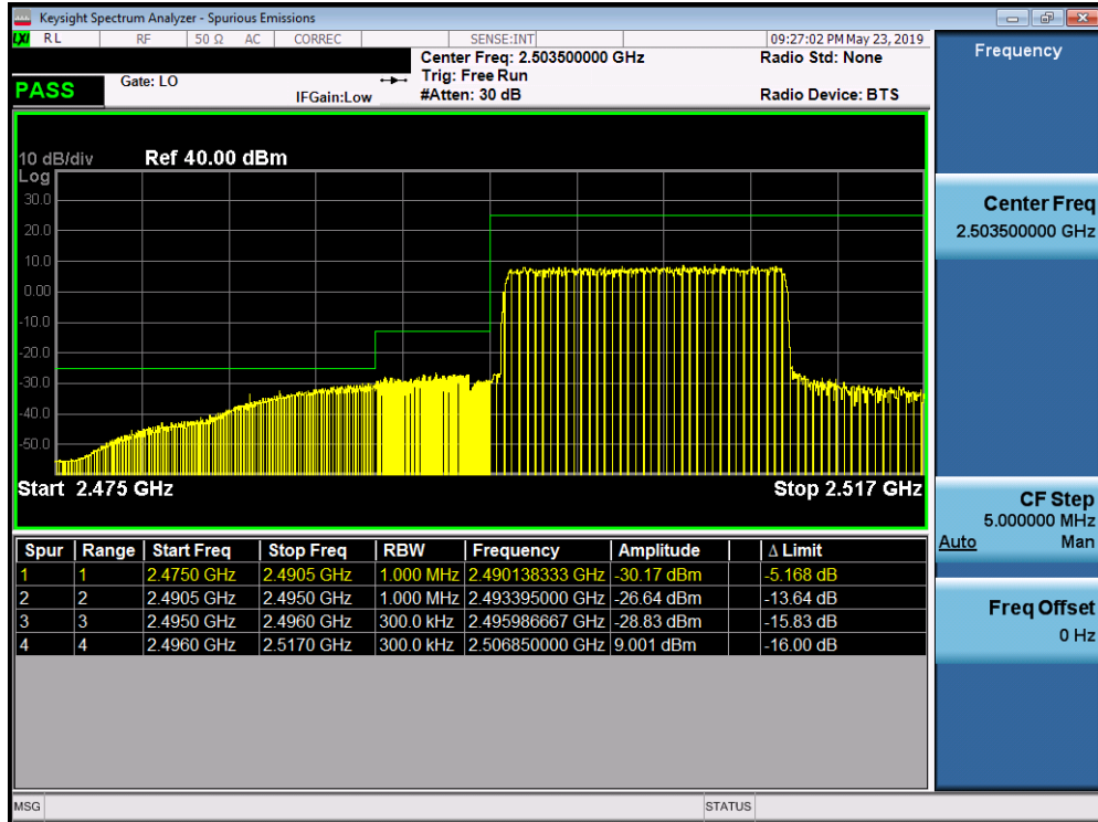
Plot 7-388. Lower ACP Plot (Band 41 (PC2)- 15.0MHz QPSK - Full RB Configuration)
