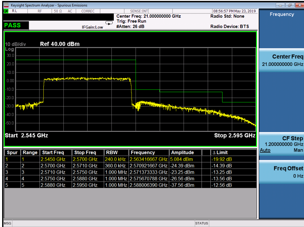
Plot 7-367. Upper ACP Plot (Band 7 - 20.0MHz QPSK - Full RB Configuration)
