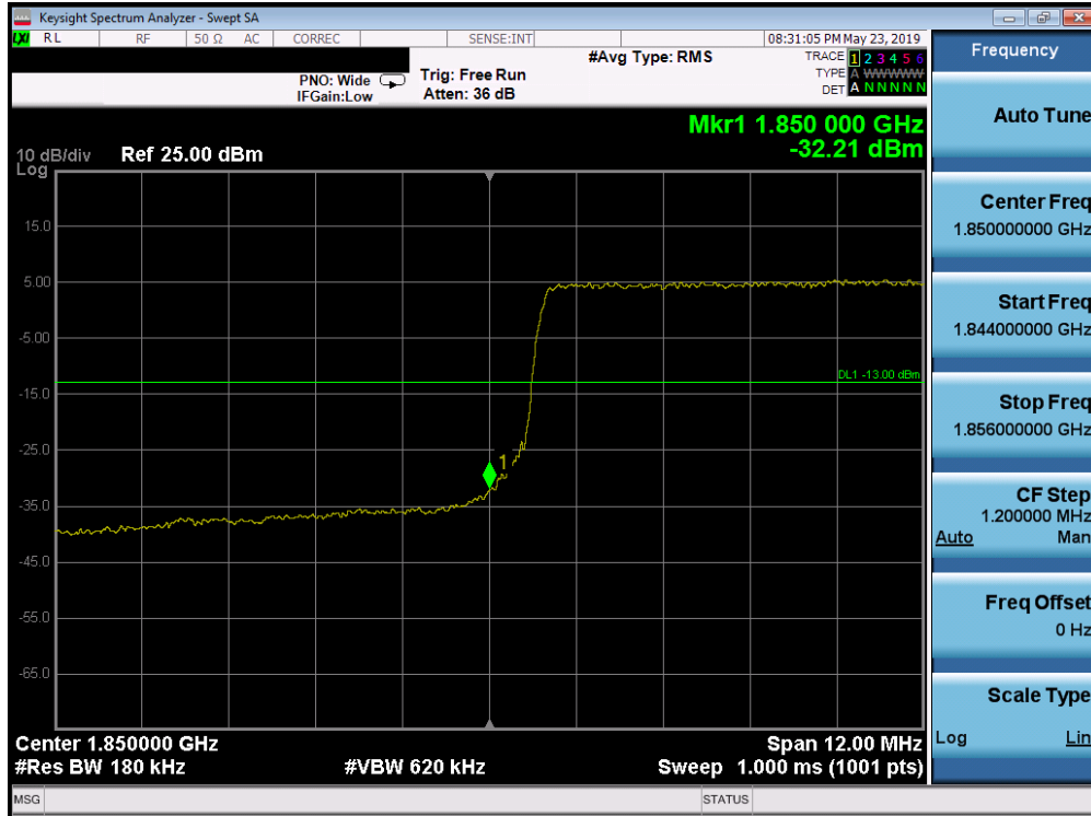
Plot 7-339. Lower Band Edge Plot (Band 25/2 - 15.0MHz QPSK - Full RB Configuration)
