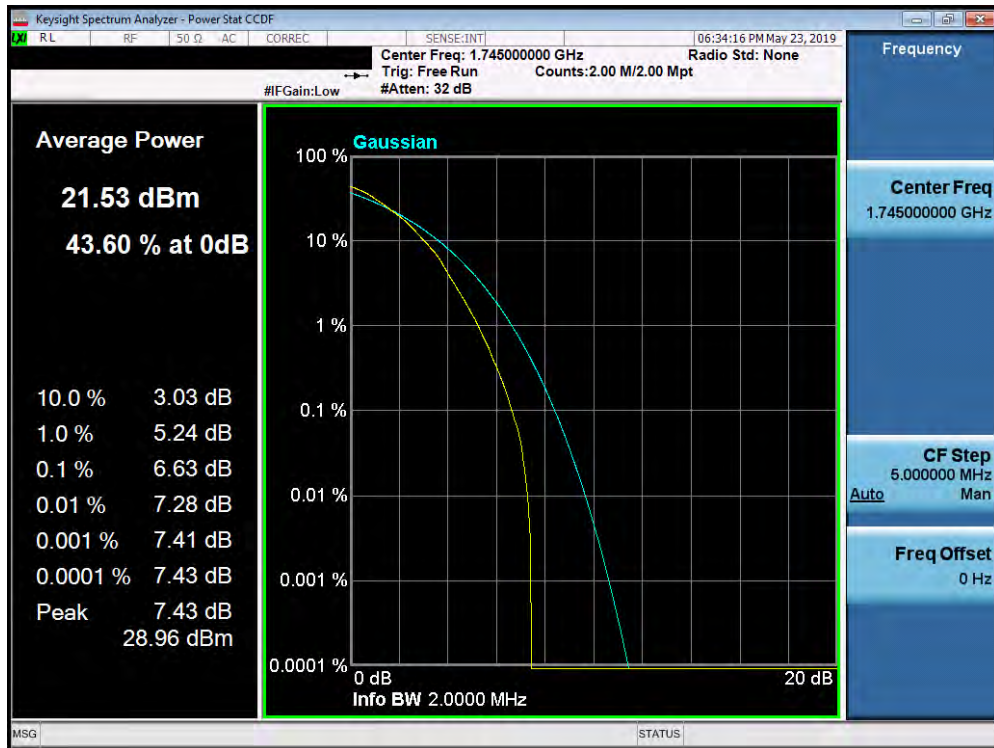
Plot 7-394. PAR Plot (Band 66/4 - 1.4MHz 64-QAM - Full RB Configuration)
