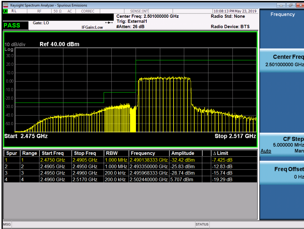
Plot 7-370. Lower ACP Plot (Band 41/38 (PC3)- 10.0MHz QPSK - Full RB Configuration)
