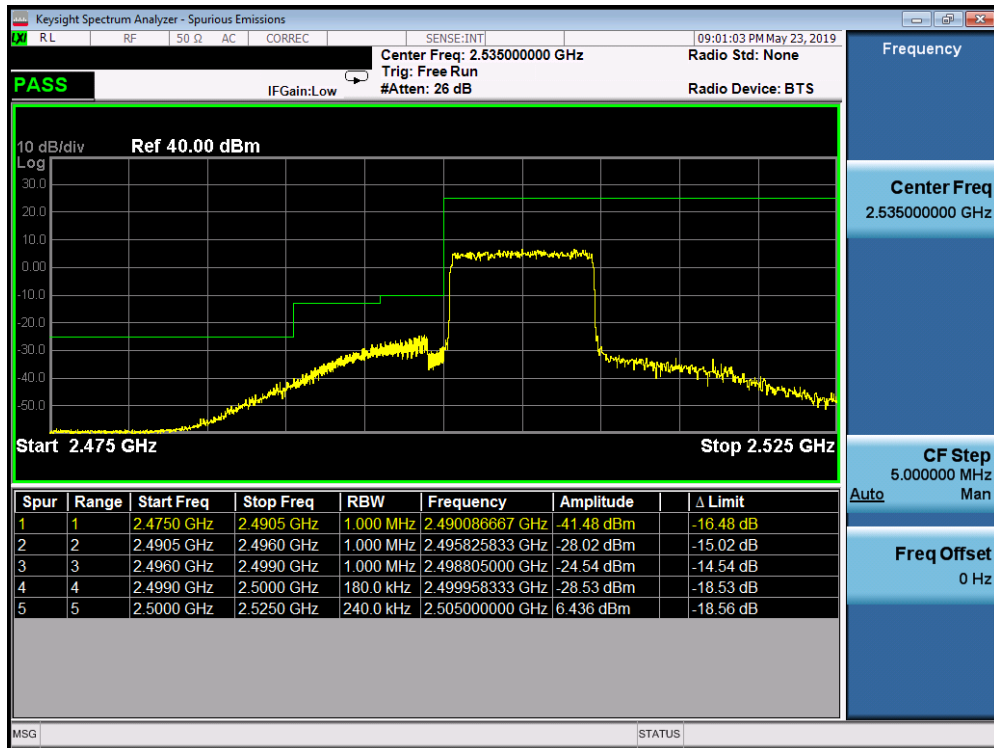
Plot 7-362. Lower ACP Plot (Band 7 - 10.0MHz QPSK - Full RB Configuration)
