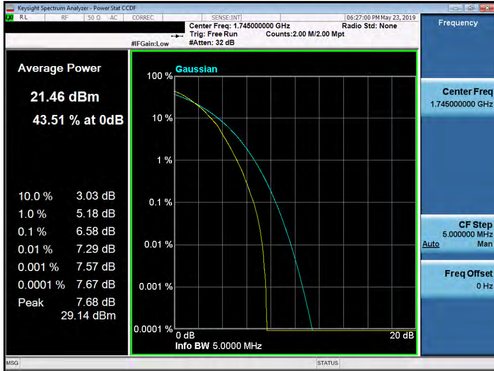
Plot 7-402. PAR Plot (Band 66/4 - 5.0MHz 64-QAM - Full RB Configuration)
