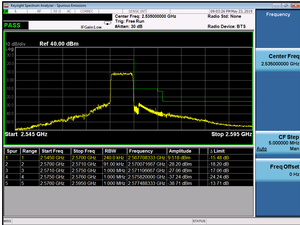
Plot 7-361. Upper ACP Plot (Band 7 - 5.0MHz QPSK - Full RB Configuration)
