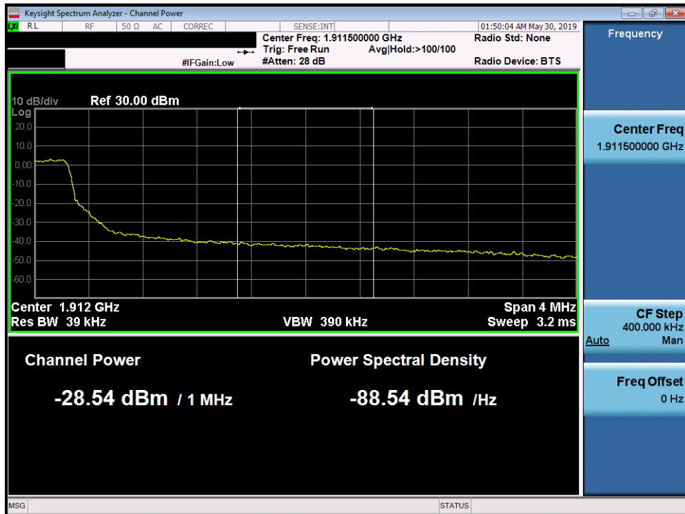
Plot 7-330. Upper Extended Band Edge Plot (Band 2 - 5.0MHz QPSK - Full RB Configuration)
