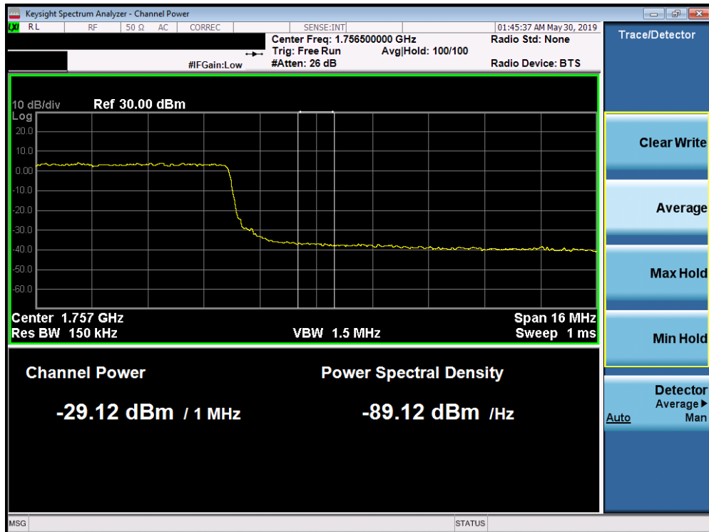
Plot 7-312. Upper Extended Band Edge Plot (Band 4 - 20.0MHz QPSK - Full RB Configuration)
