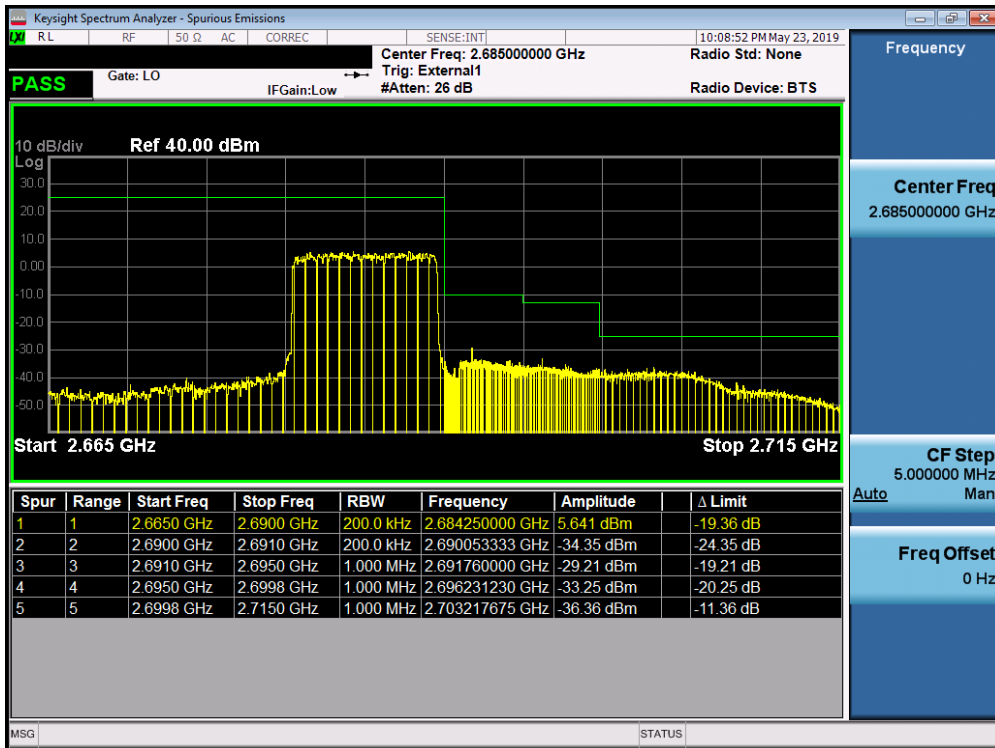
Plot 7-371. Upper ACP Plot (Band 41/38 (PC3)- 10.0MHz QPSK - Full RB Configuration)
