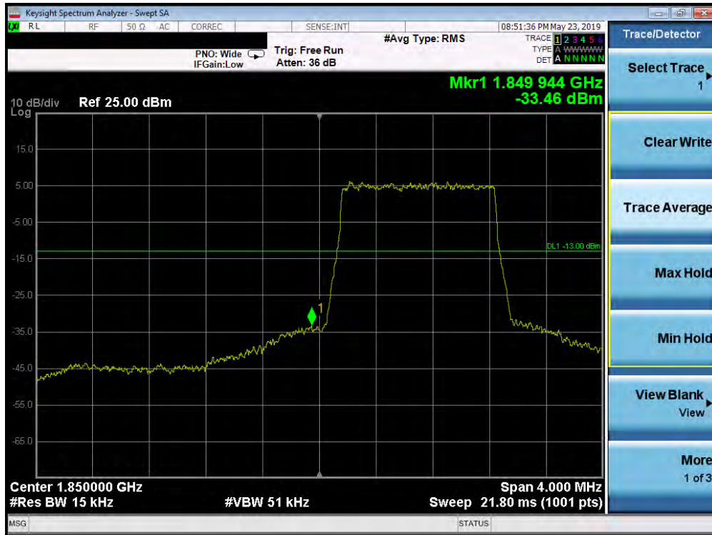
Plot 7-315. Lower Band Edge Plot (Band 25/2 - 1.4MHz QPSK - Full RB Configuration)
