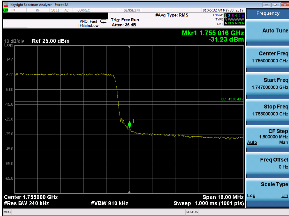
Plot 7-311. Upper Band Edge Plot (Band 4 - 20.0MHz QPSK - Full RB Configuration)
