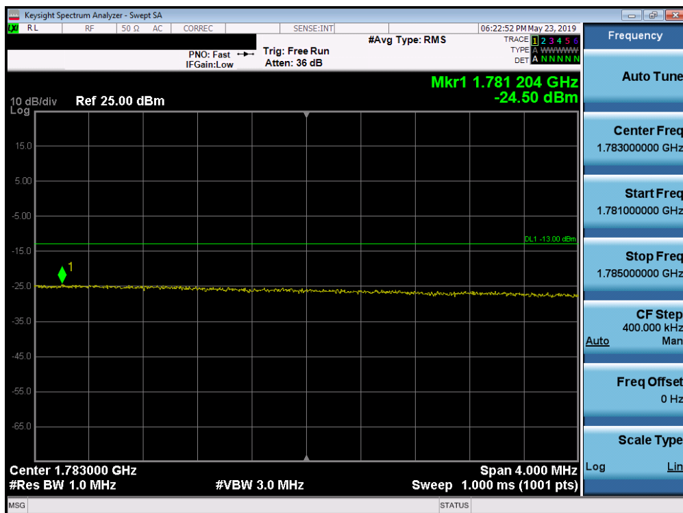
Plot 7-308. Upper Extended Band Edge Plot (Band 66 - 15.0MHz QPSK - Full RB Configuration)
