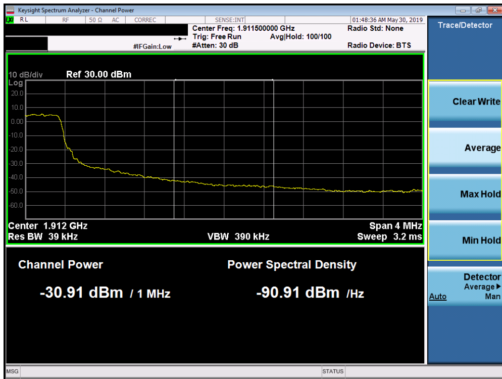
Plot 7-324. Upper Extended Band Edge Plot (Band 2 - 3.0MHz QPSK - Full RB Configuration)
