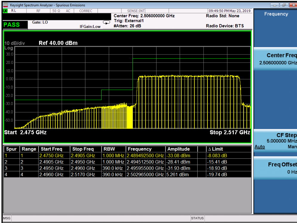
Plot 7-374. Lower ACP Plot (Band 41/38 (PC3)- 20.0MHz QPSK - Full RB Configuration)
