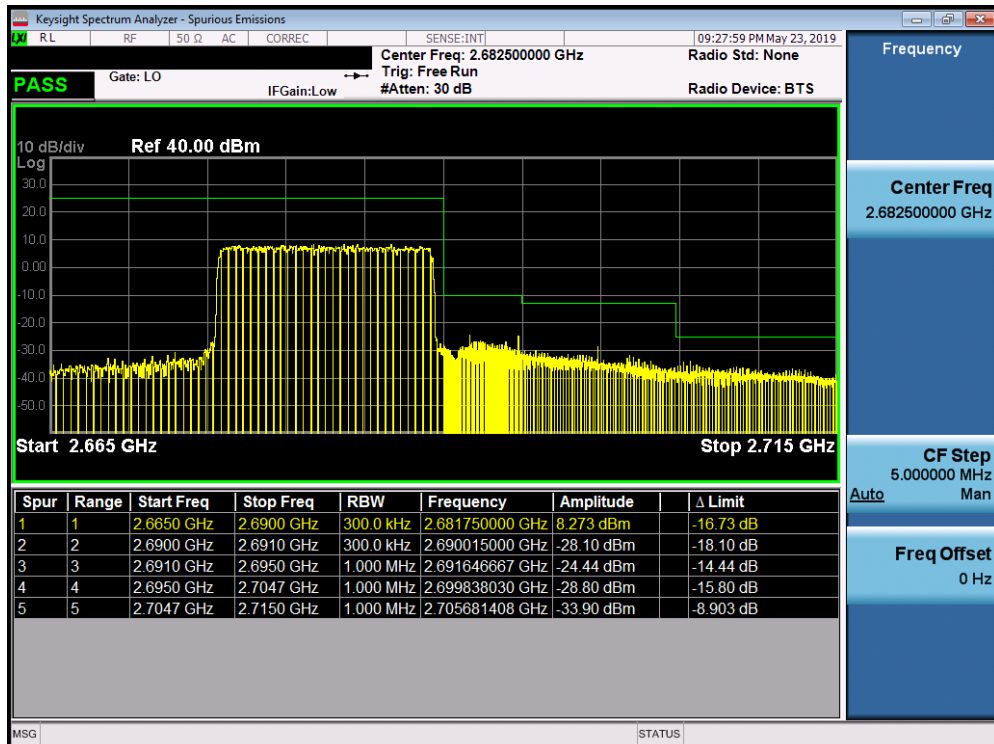
Plot 7-389. Upper ACP Plot (Band 41 (PC2)- 15.0MHz QPSK - Full RB Configuration)
