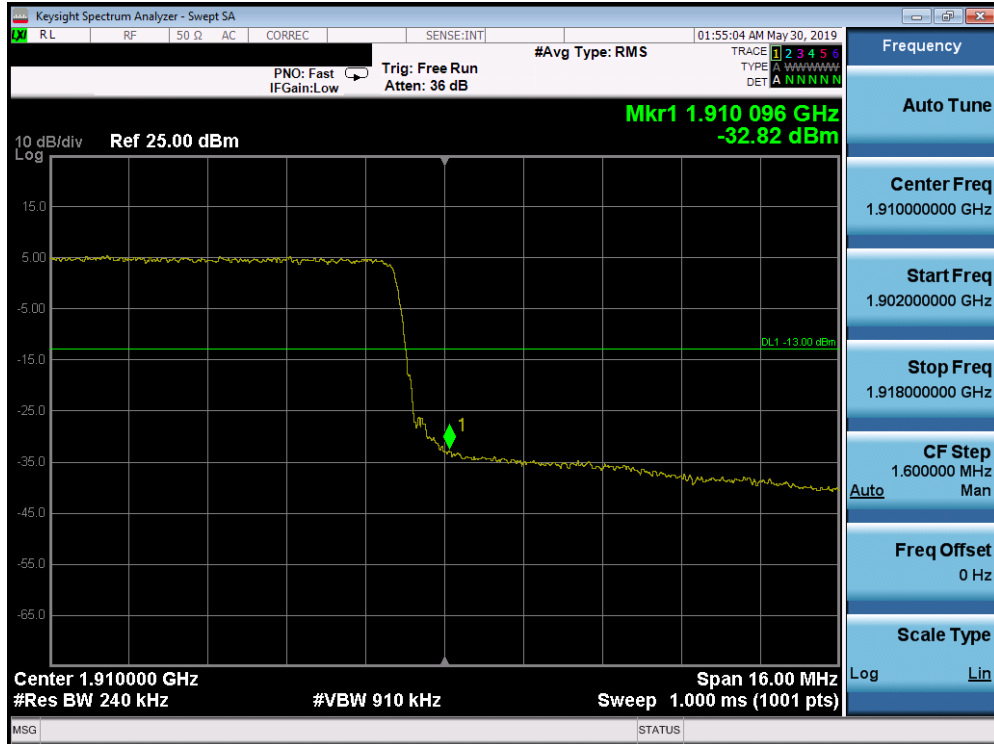
Plot 7-347. Upper Band Edge Plot (Band 2 - 20.0MHz QPSK - Full RB Configuration)
