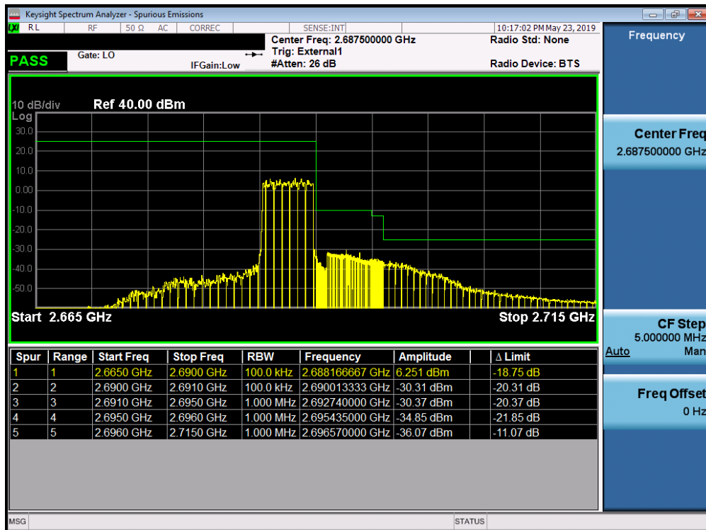
Plot 7-369. Upper ACP Plot (Band 41/38 (PC3)- 5.0MHz QPSK - Full RB Configuration)
