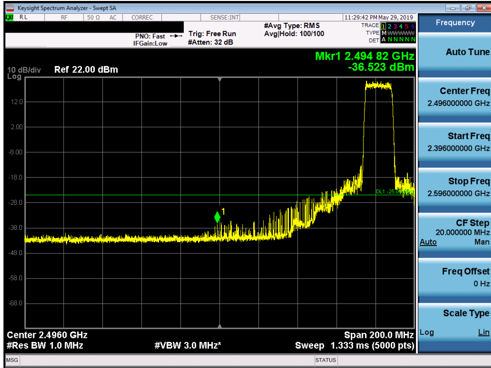
Plot 7-380. Lower ACP Plot (Band 38 - 15.0MHz QPSK - Full RB Configuration)
