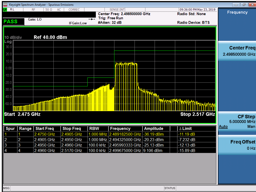
Plot 7-384. Lower ACP Plot (Band 41 (PC2)- 5.0MHz QPSK - Full RB Configuration)
