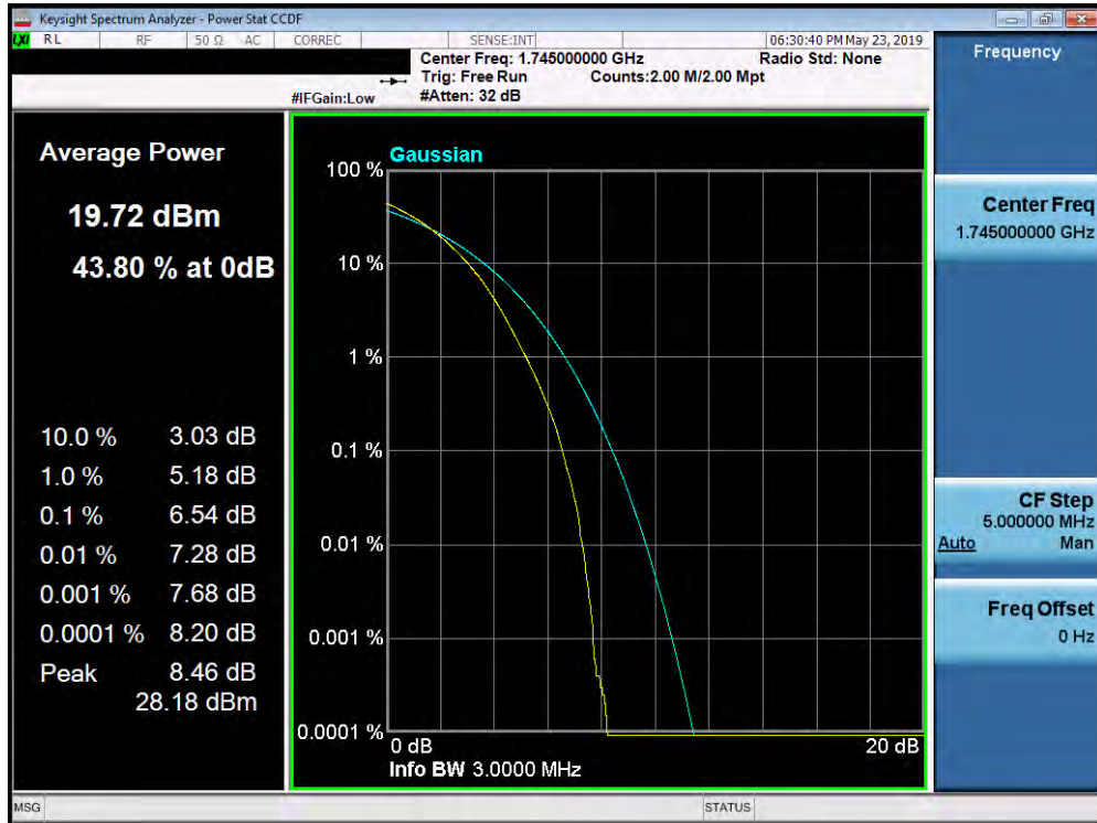
Plot 7-399. PAR Plot (Band 66/4 - 3.0MHz 256-QAM - Full RB Configuration)
