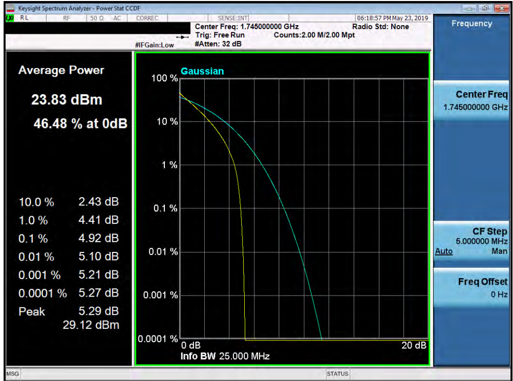
Plot 7-408. PAR Plot (Band 66/4 - 15.0MHz QPSK - Full RB Configuration)
