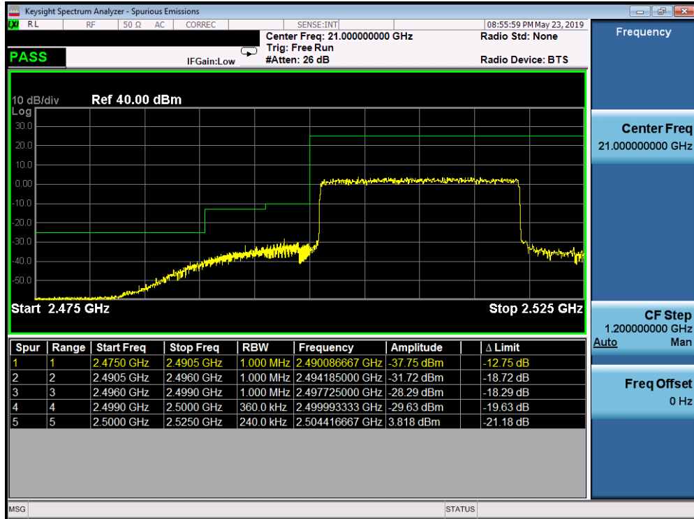
Plot 7-366. Lower ACP Plot (Band 7 - 20.0MHz QPSK - Full RB Configuration)
