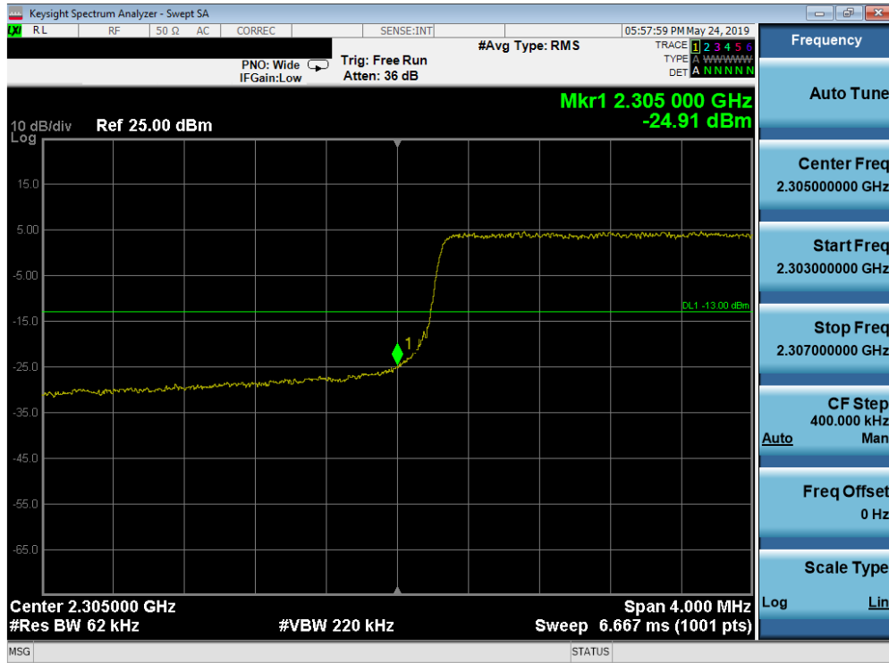
Plot 7-351. Lower Band Edge Plot (Band 30 - 5.0MHz QPSK - Full RB Configuration)
