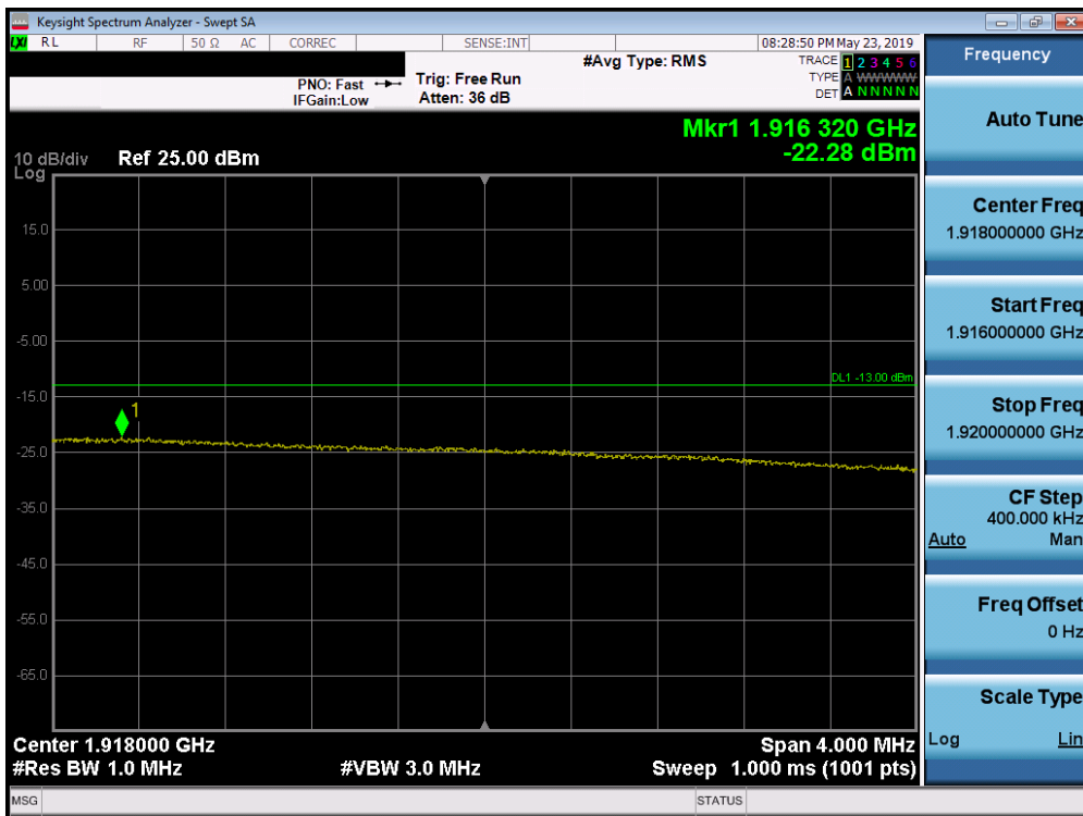
Plot 7-350. Upper Extended Band Edge Plot (Band 25 - 20.0MHz QPSK - Full RB Configuration)
