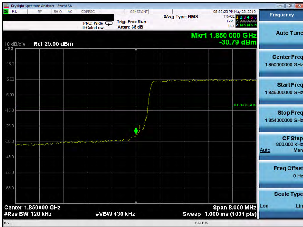
Plot 7-333. Lower Band Edge Plot (Band 25/2 - 10.0MHz QPSK - Full RB Configuration)
