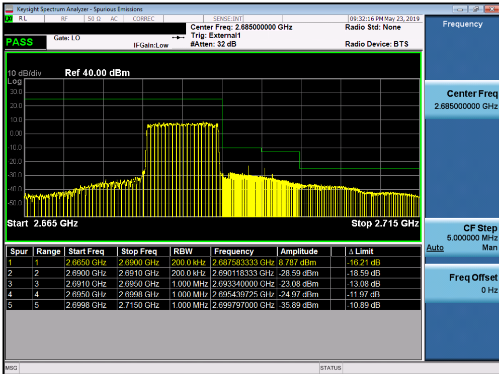
Plot 7-387. Upper ACP Plot (Band 41 (PC2)- 10.0MHz QPSK - Full RB Configuration)
