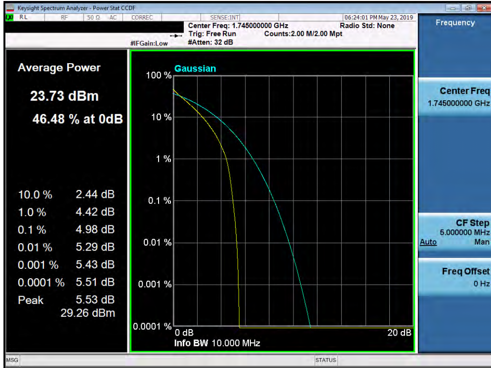
Plot 7-404. PAR Plot (Band 66/4 - 10.0MHz QPSK - Full RB Configuration)
