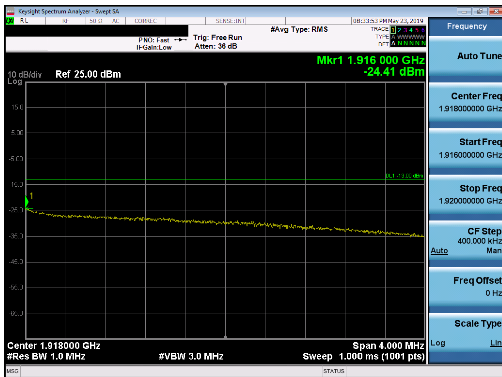
Plot 7-338. Upper Extended Band Edge Plot (Band 25 - 10.0MHz QPSK - Full RB Configuration)
