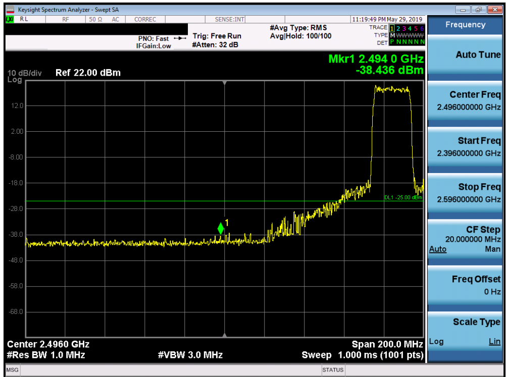
Plot 7-382. Lower ACP Plot (Band 38 - 20.0MHz QPSK - Full RB Configuration)
