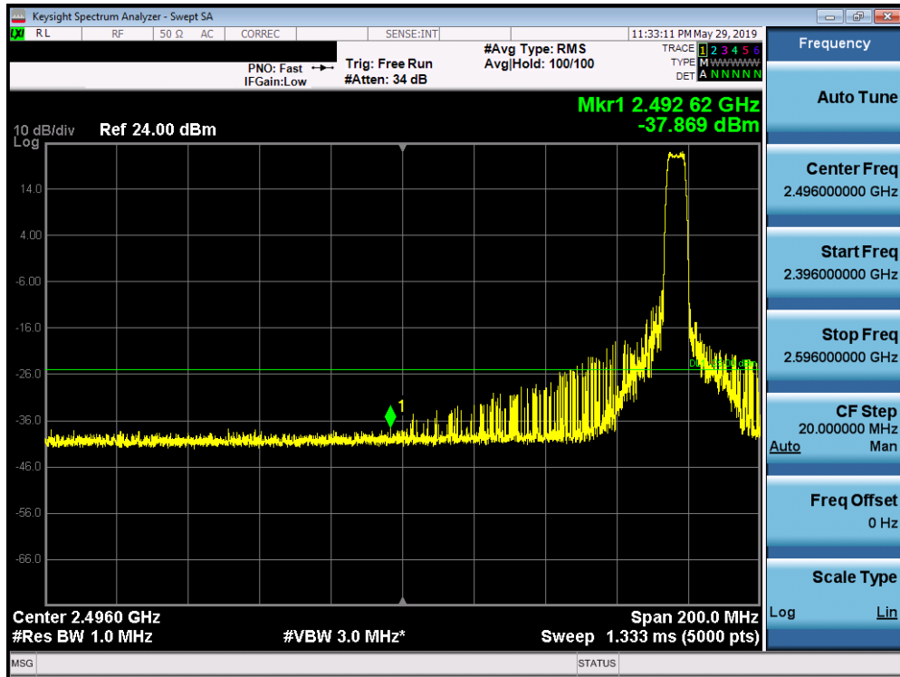
Plot 7-376. Lower ACP Plot (Band 38 - 5.0MHz QPSK - Full RB Configuration)
