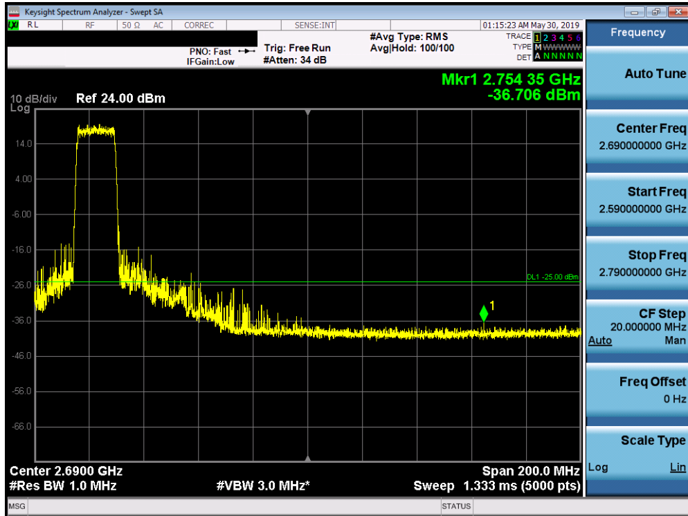
Plot 7-381. Upper ACP Plot (Band 38 - 15.0MHz QPSK - Full RB Configuration)
