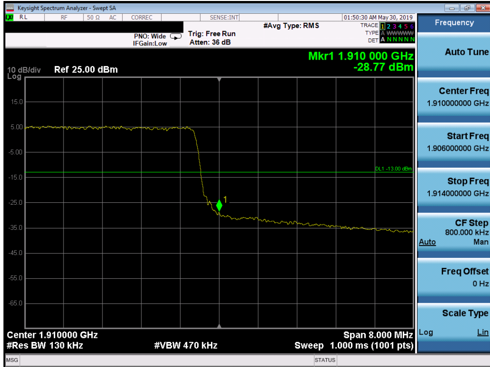
Plot 7-335. Upper Band Edge Plot (Band 2 - 10.0MHz QPSK - Full RB Configuration)
