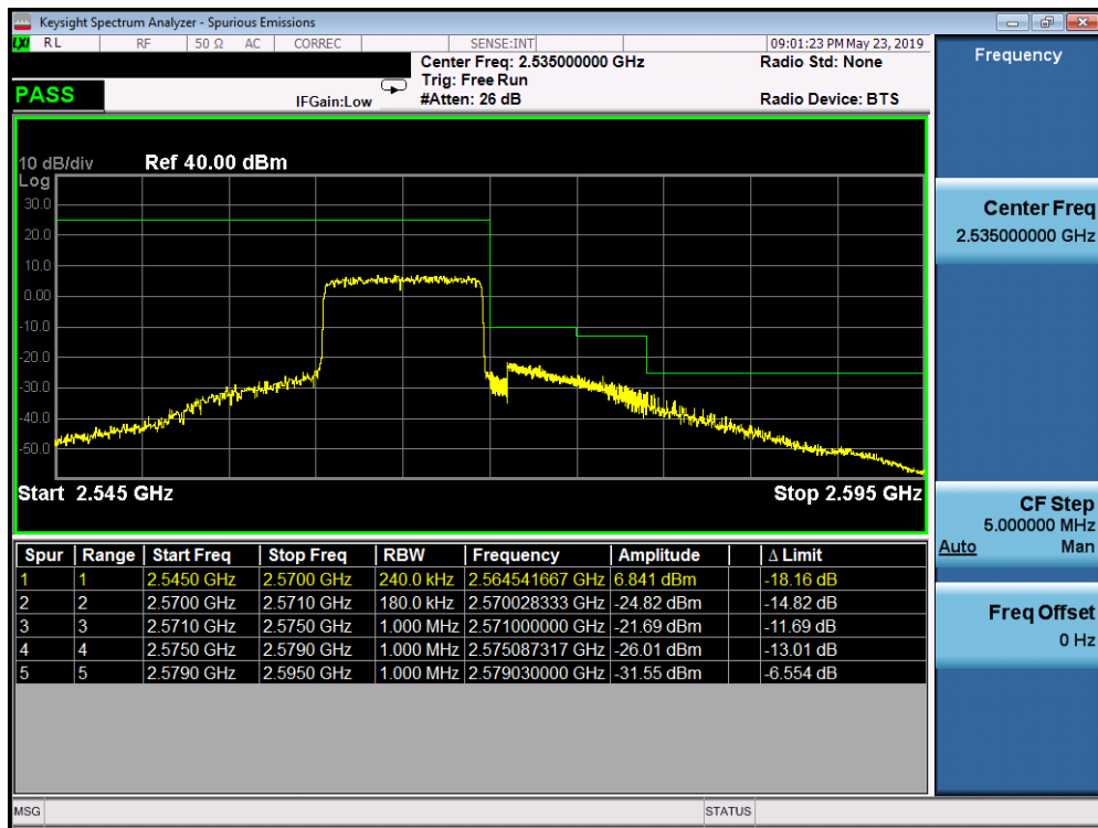
Plot 7-363. Upper ACP Plot (Band 7 - 10.0MHz QPSK - Full RB Configuration)
