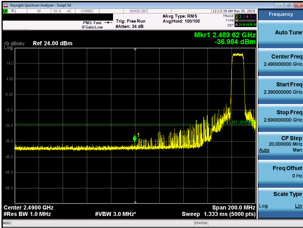
Plot 7-378. Lower ACP Plot (Band 38 - 10.0MHz QPSK - Full RB Configuration)
