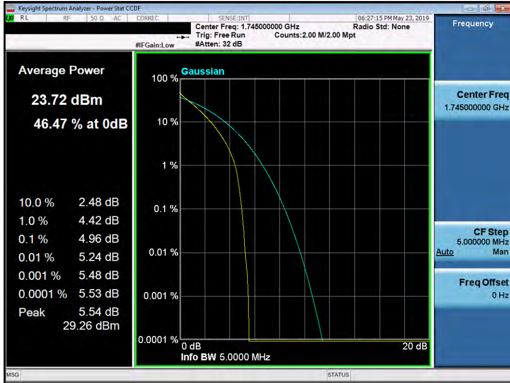
Plot 7-400. PAR Plot (Band 66/4 - 5.0MHz QPSK - Full RB Configuration)
