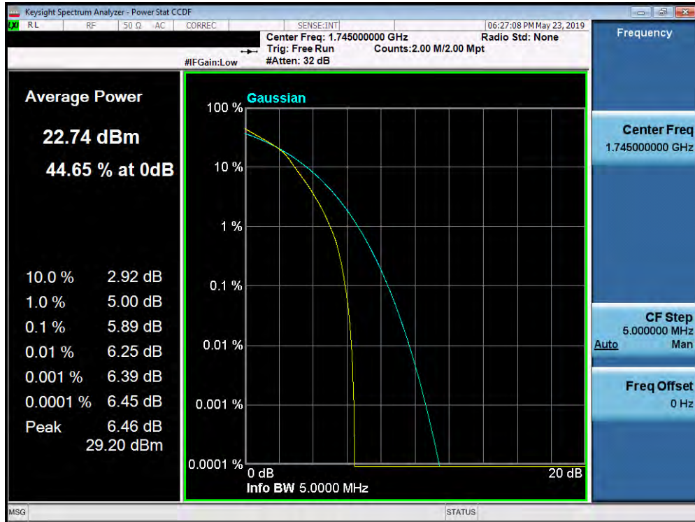
Plot 7-401. PAR Plot (Band 66/4 - 5.0MHz 16-QAM - Full RB Configuration)
