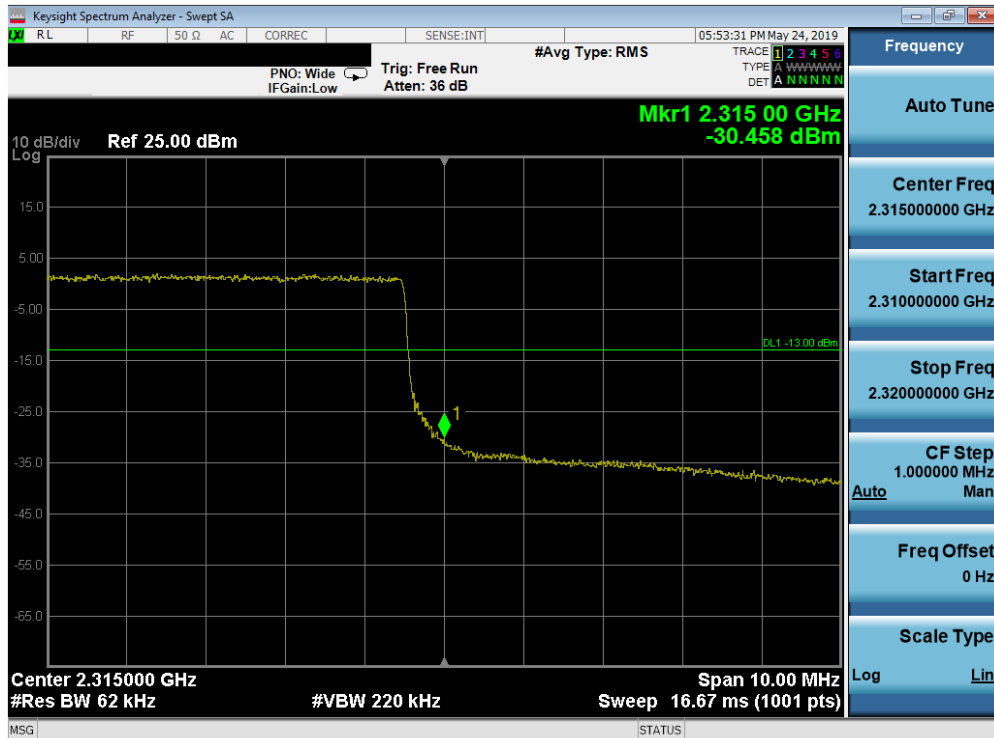
Plot 7-358. Upper Band Edge Plot (Band 30 - 10.0MHz QPSK - Full RB Configuration)
