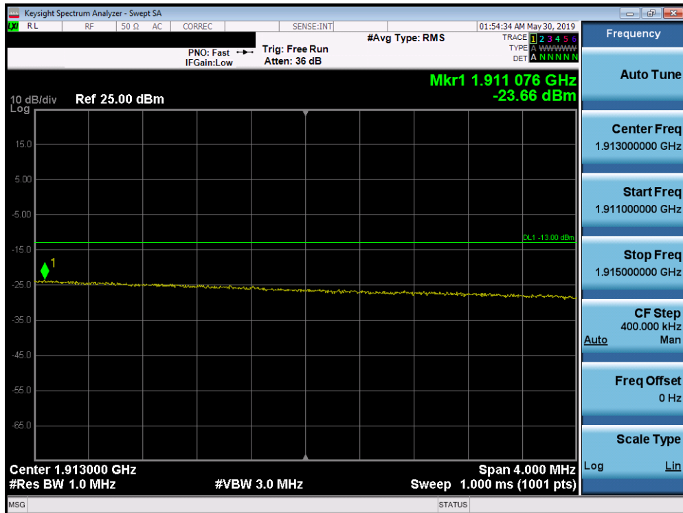
Plot 7-342. Upper Extended Band Edge Plot (Band 2 - 15.0MHz QPSK - Full RB Configuration)
