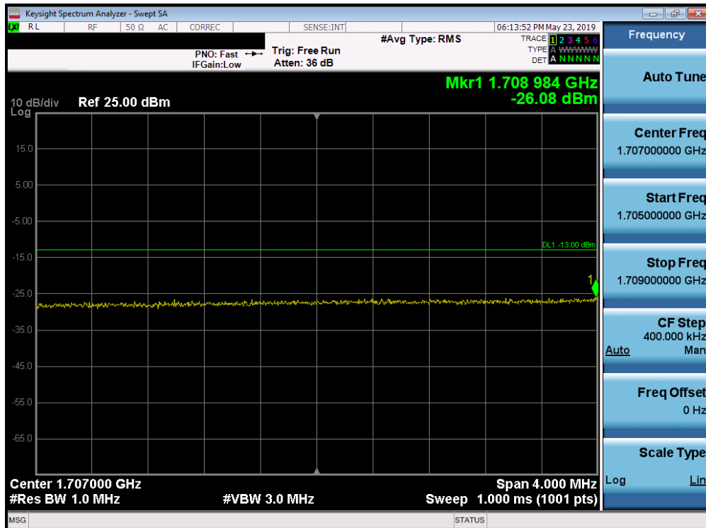
Plot 7-310. Lower Extended Band Edge Plot (Band 66/4 - 20.0MHz QPSK - Full RB Configuration)
