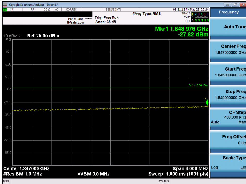
Plot 7-340. Lower Extended Band Edge Plot (Band 25/2 - 15.0MHz QPSK - Full RB Configuration)
