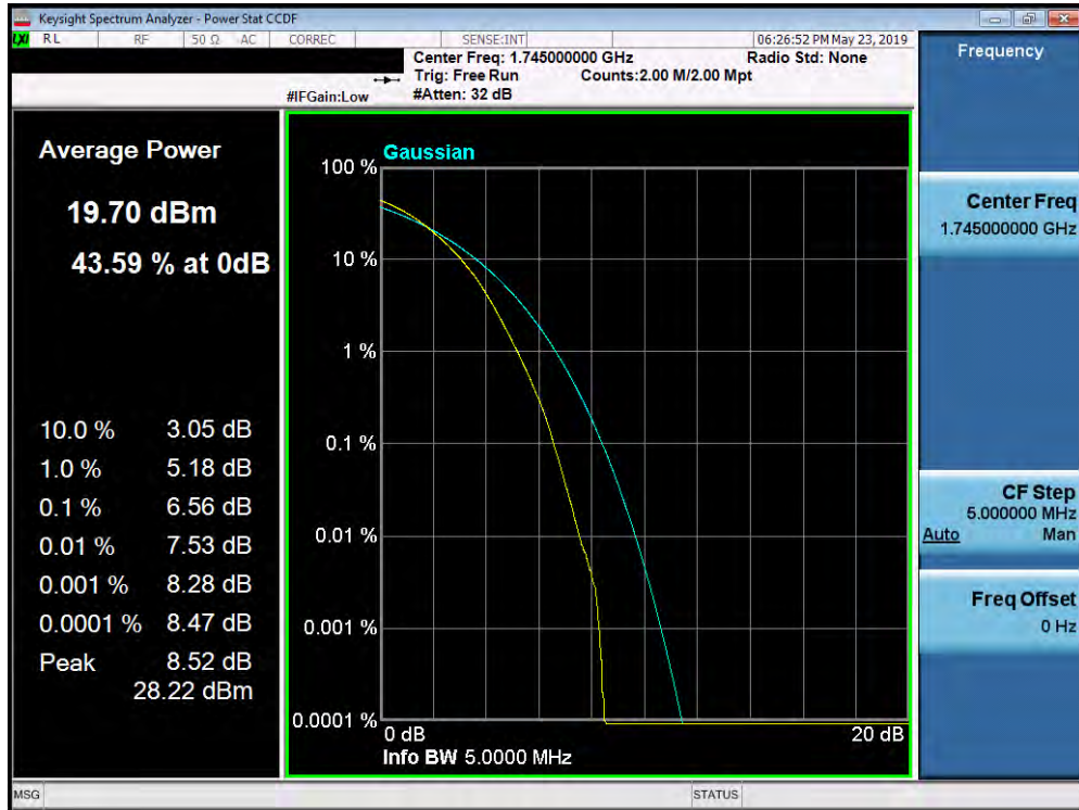
Plot 7-403. PAR Plot (Band 66/4 - 5.0MHz 256-QAM - Full RB Configuration)
