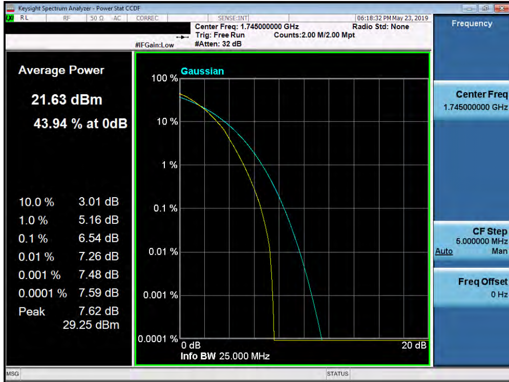
Plot 7-410. PAR Plot (Band 66/4 - 15.0MHz 64-QAM - Full RB Configuration)
