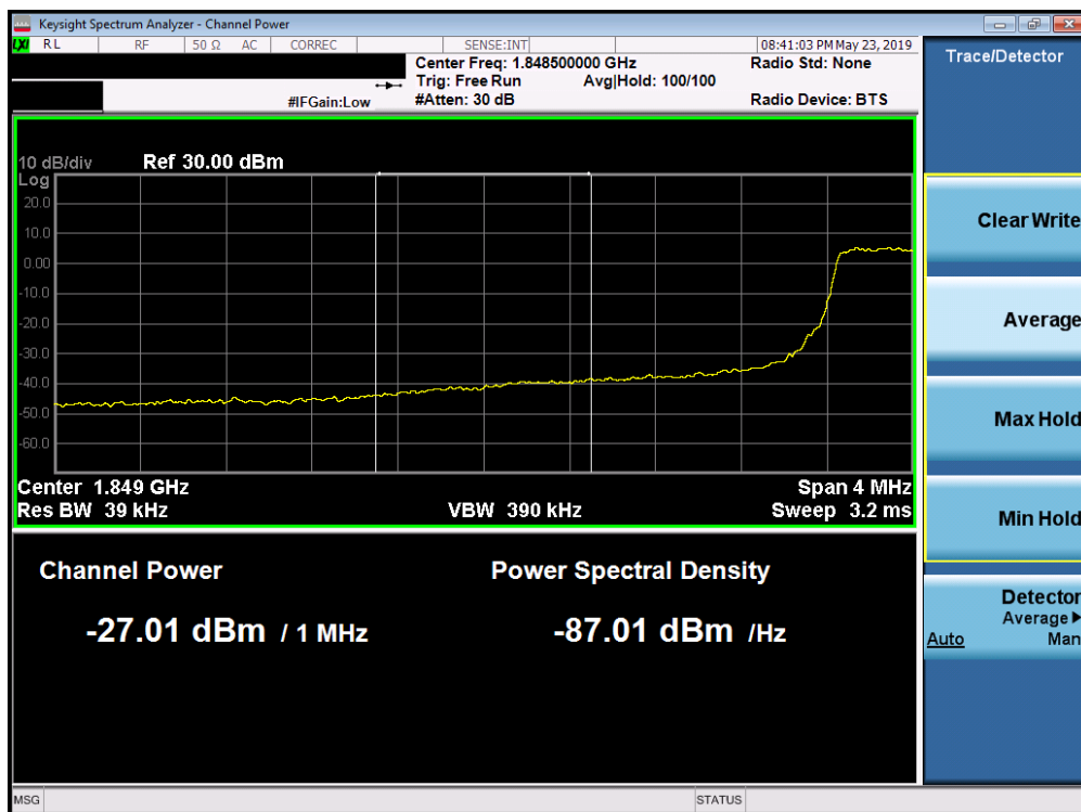
Plot 7-322. Lower Extended Band Edge Plot (Band 25/2 - 3.0MHz QPSK - Full RB Configuration)
