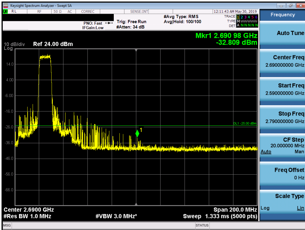
Plot 7-379. Upper ACP Plot (Band 38 - 10.0MHz QPSK - Full RB Configuration)
