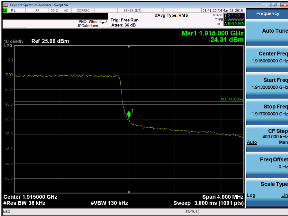
Plot 7-325. Upper Band Edge Plot (Band 25 - 3.0MHz QPSK - Full RB Configuration)
