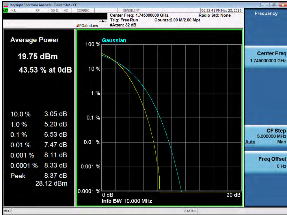
Plot 7-407. PAR Plot (Band 66/4 - 10.0MHz 256-QAM - Full RB Configuration)
