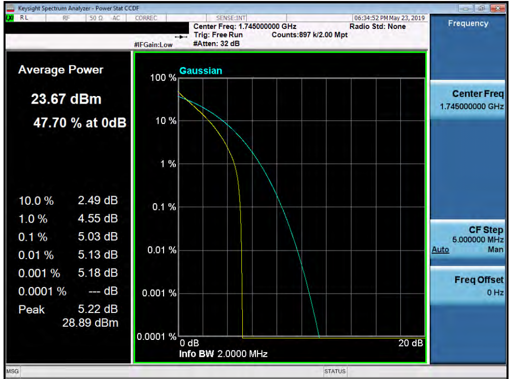
Plot 7-392. PAR Plot (Band 66/4 - 1.4MHz QPSK - Full RB Configuration)
