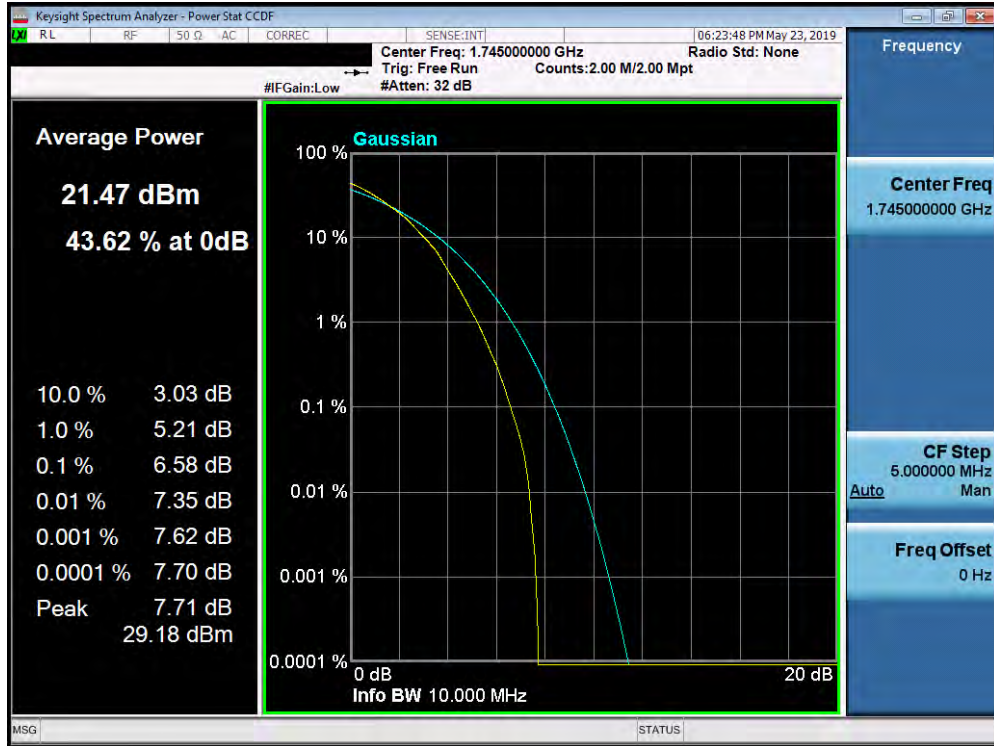
Plot 7-406. PAR Plot (Band 66/4 - 10.0MHz 64-QAM - Full RB Configuration)
