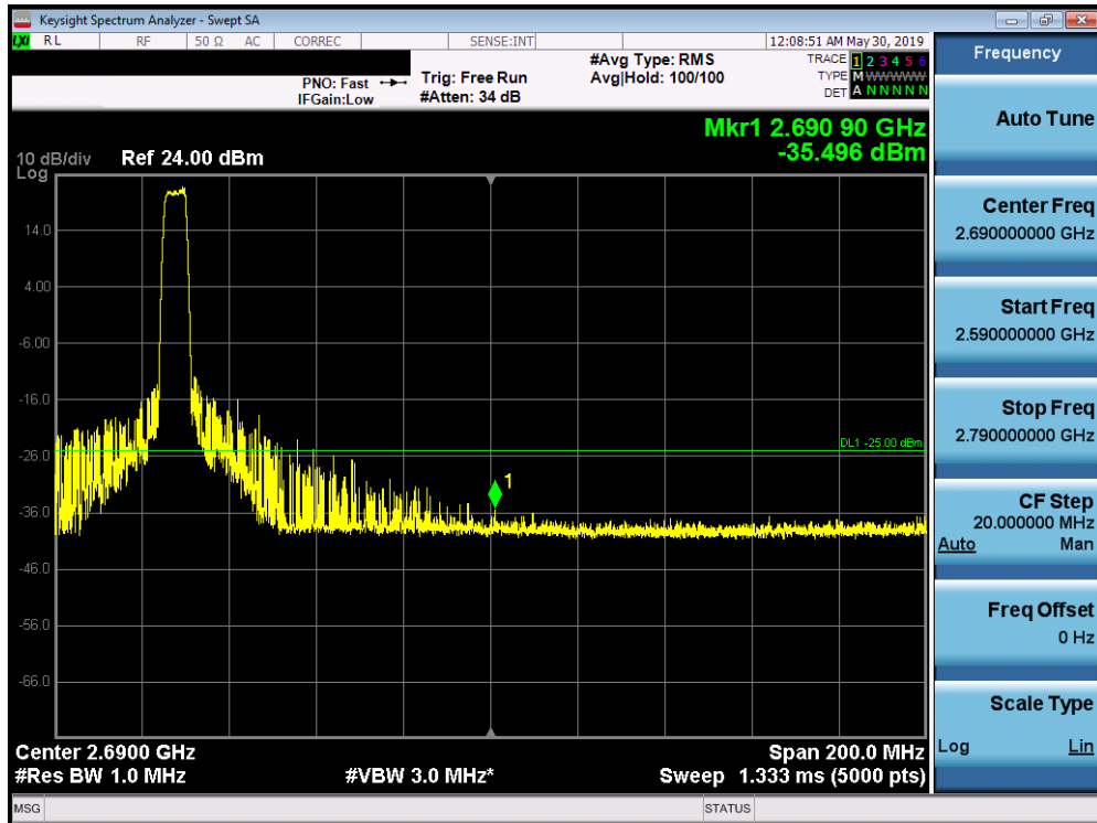
Plot 7-377. Upper ACP Plot (Band 38 - 5.0MHz QPSK - Full RB Configuration)
