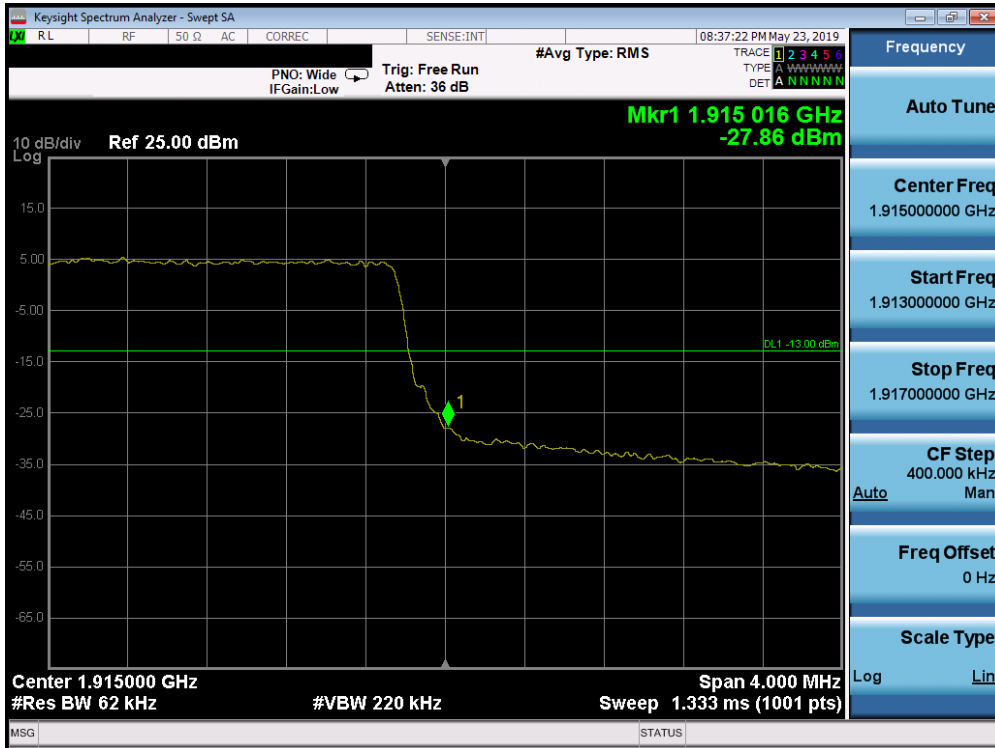
Plot 7-331. Upper Band Edge Plot (Band 25 - 5.0MHz QPSK - Full RB Configuration)
