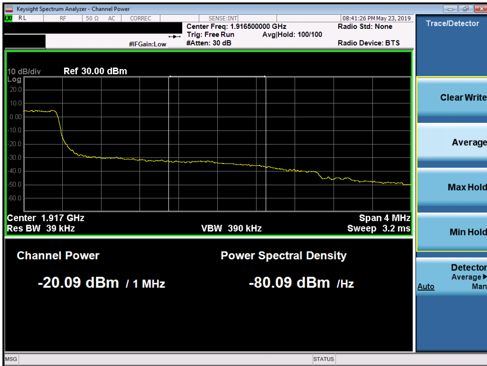
Plot 7-326. Upper Extended Band Edge Plot (Band 25 - 3.0MHz QPSK - Full RB Configuration)
