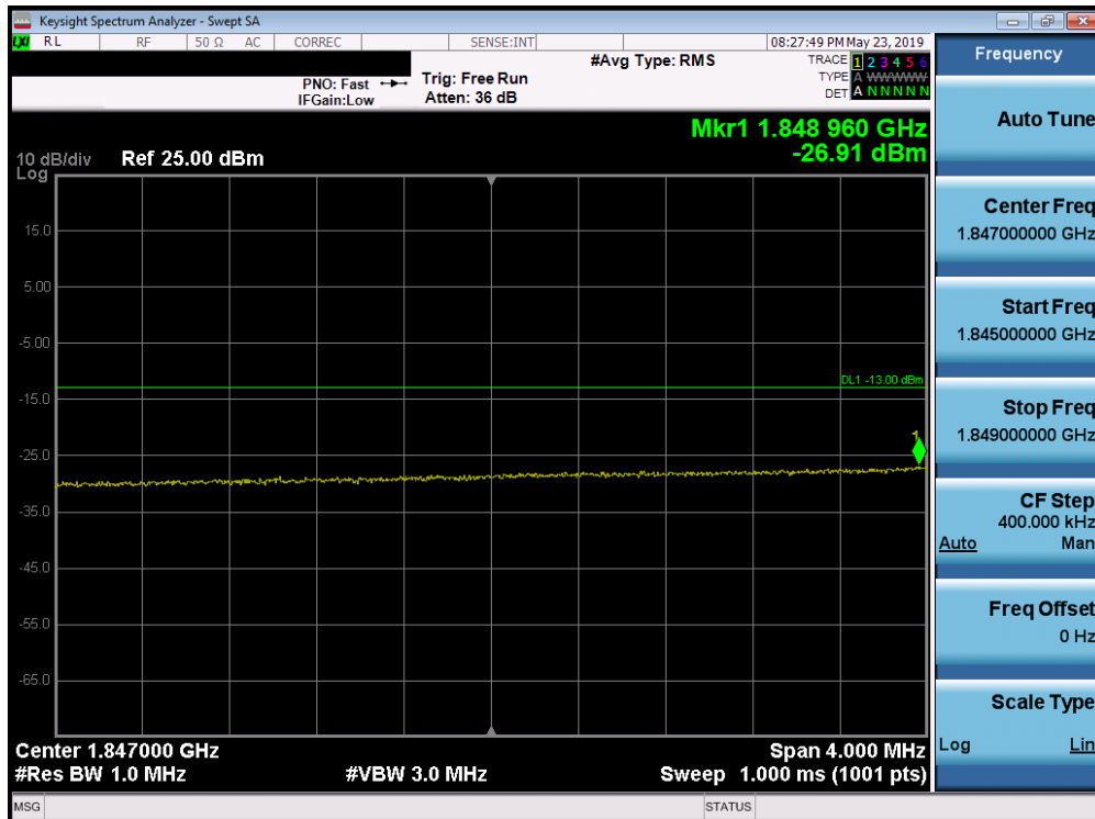
Plot 7-346. Lower Extended Band Edge Plot (Band 25/2 - 20.0MHz QPSK - Full RB Configuration)
