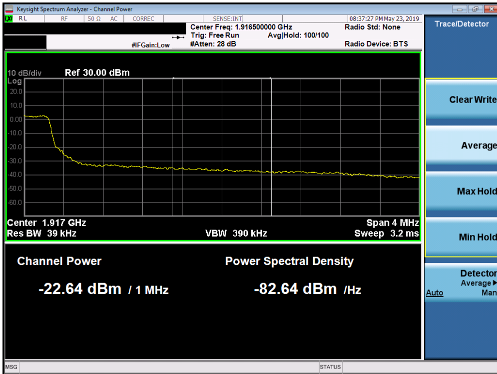
Plot 7-332. Upper Extended Band Edge Plot (Band 25 - 5.0MHz QPSK - Full RB Configuration)
