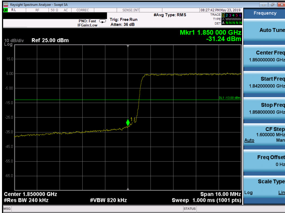
Plot 7-345. Lower Band Edge Plot (Band 25/2 - 20.0MHz QPSK - Full RB Configuration)
