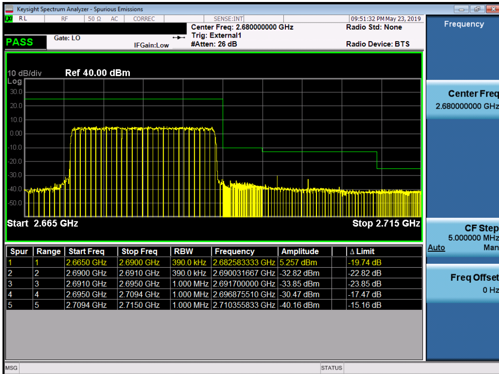
Plot 7-375. Upper ACP Plot (Band 41/38 (PC3)- 20.0MHz QPSK - Full RB Configuration)
