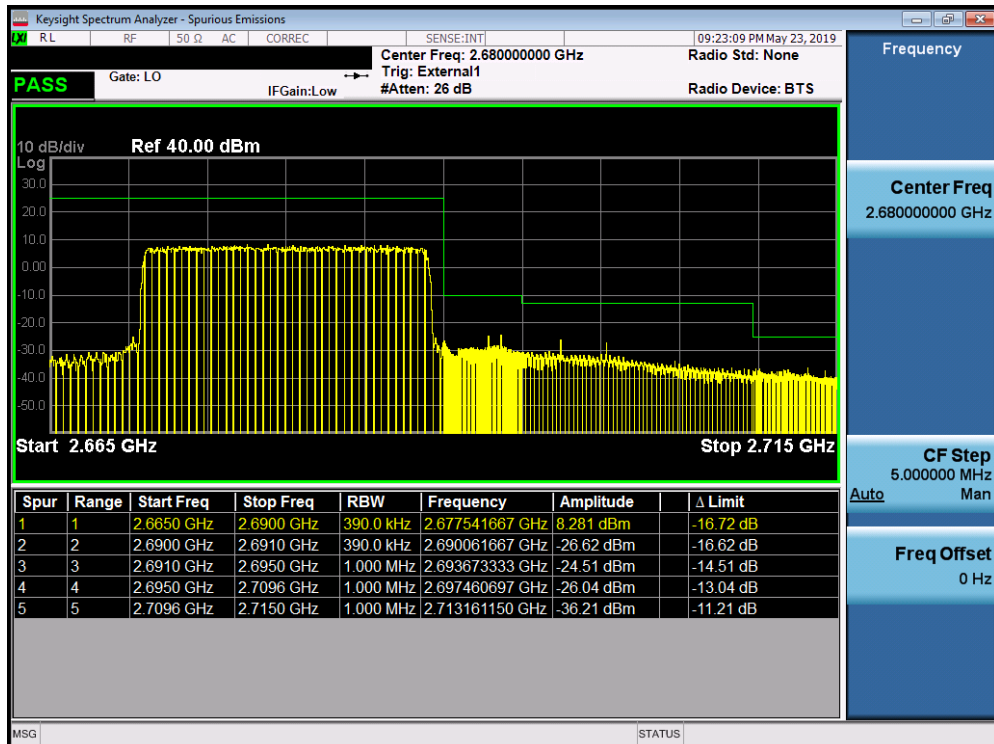
Plot 7-391. Upper ACP Plot (Band 41 (PC2)- 20.0MHz QPSK - Full RB Configuration)
