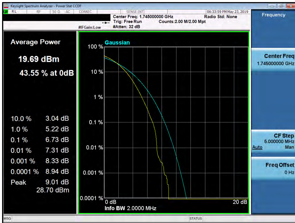
Plot 7-395. PAR Plot (Band 66/4 - 1.4MHz 256-QAM - Full RB Configuration)
