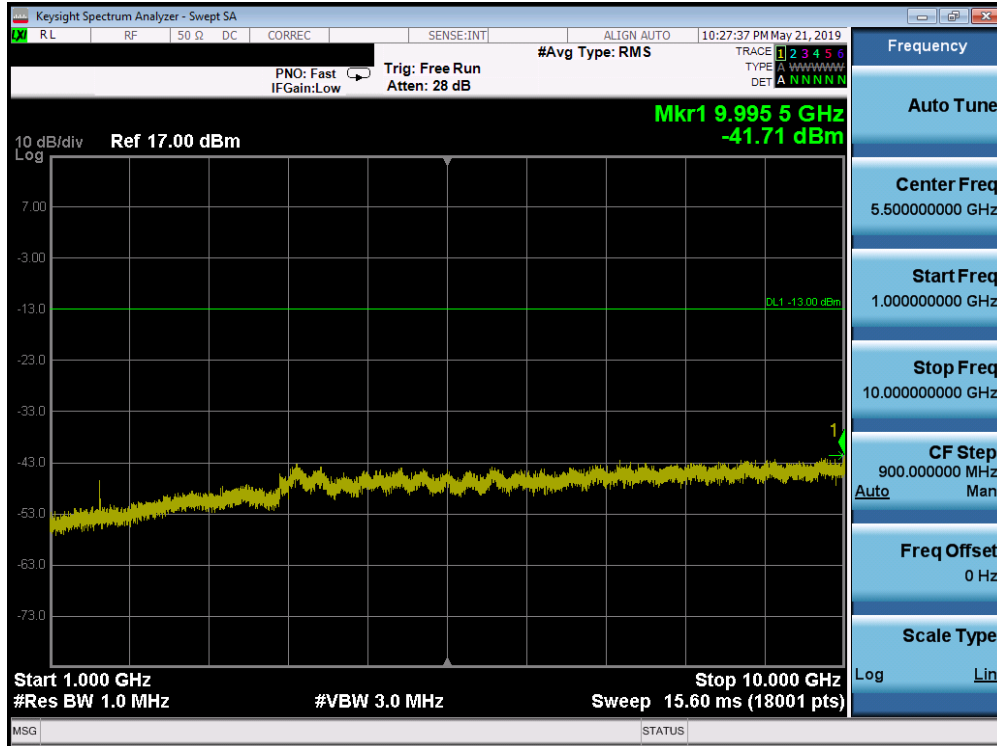
Plot 7-191. Conducted Spurious Plot (Band 13 - 5.0MHz QPSK - RB Size 1, RB Offset 0 - High Channel)
