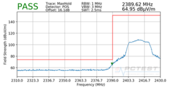
Plot 7-92. Radiated Restricted Band Edge Measurement MIMO with WCP (Peak)
