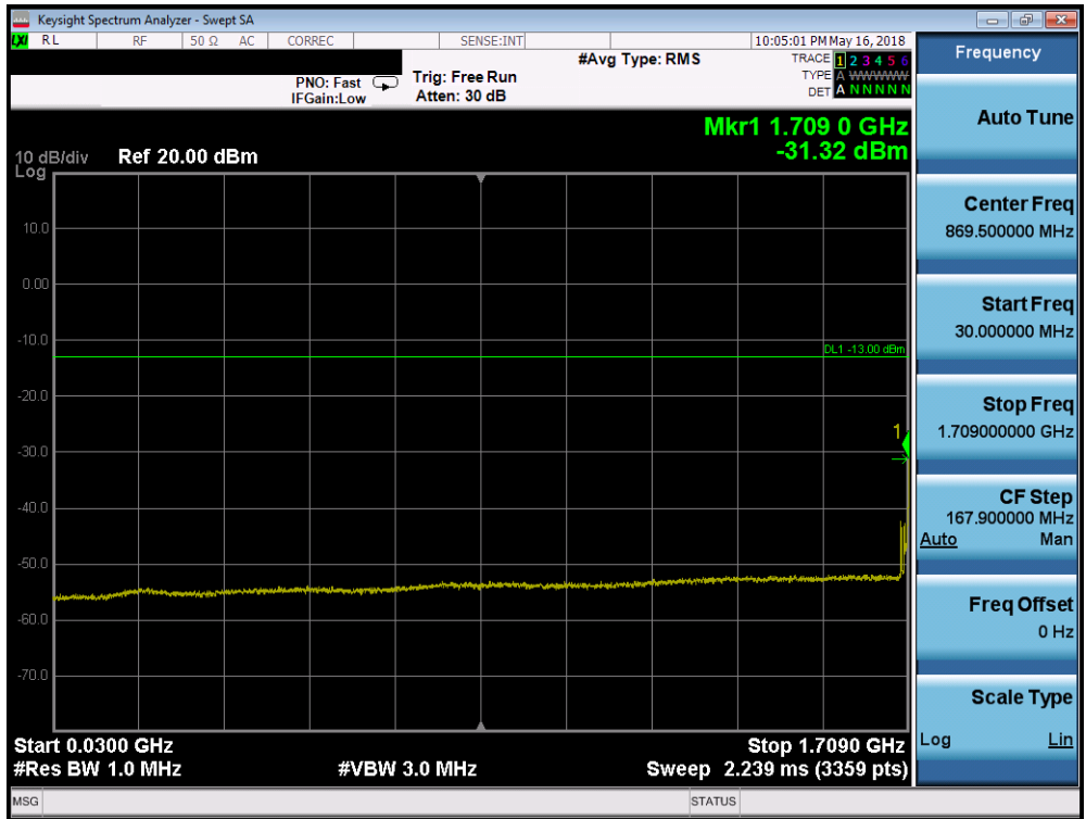
Plot 7-172. Conducted Spurious Plot (Band 66/4 - 20.0MHz QPSK - RB Size 1, RB Offset 0 - Low Channel)
