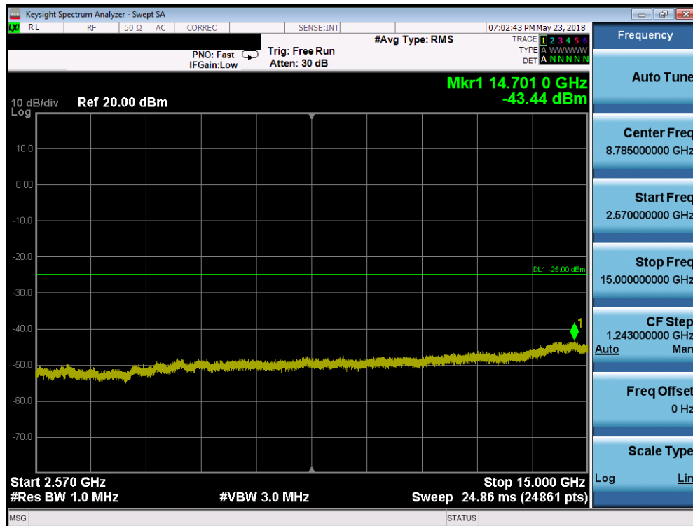
Plot 7-212. Conducted Spurious Plot (Band 7 - 15.0MHz QPSK - RB Size 1, RB Offset 0 - Low Channel)
