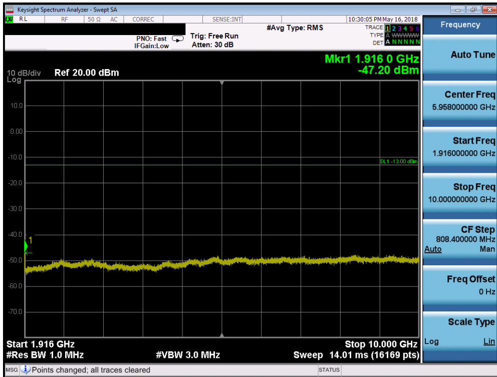
Plot 7-188. Conducted Spurious Plot (Band 25/2 - 20.0MHz QPSK - RB Size 1, RB Offset 0 - High Channel)
