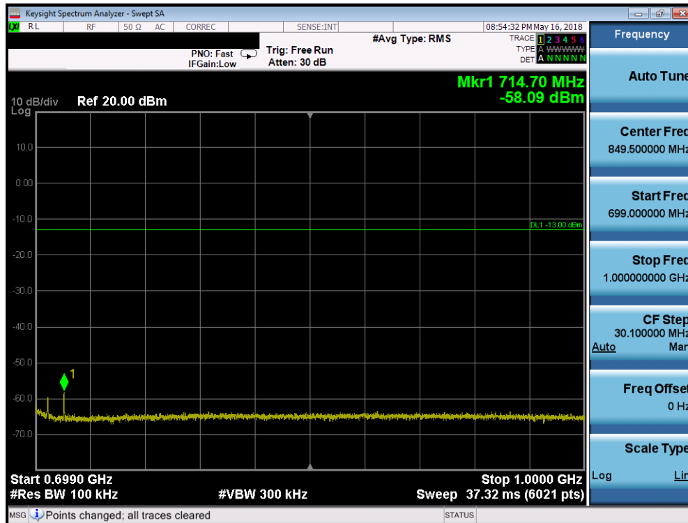
Plot 7-149. Conducted Spurious Plot (Band 71 - 20.0MHz QPSK - RB Size 1, RB Offset 0 - High Channel)
