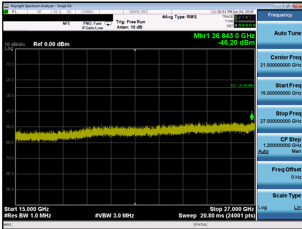
Plot 7-222. Conducted Spurious Plot (Band 41/38 - 20.0MHz QPSK - RB Size 1, RB Offset 0 - Low Channel)
