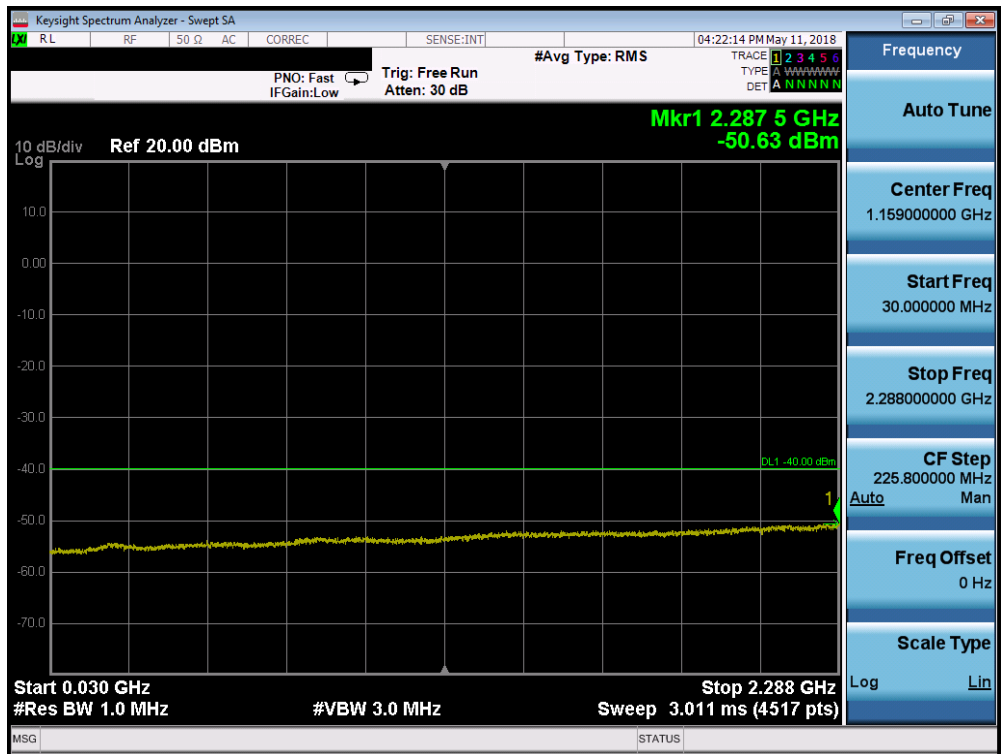
Plot 7-196. Conducted Spurious Plot (Band 30 - 5.0MHz QPSK - RB Size 1, RB Offset 0 - Mid Channel)
