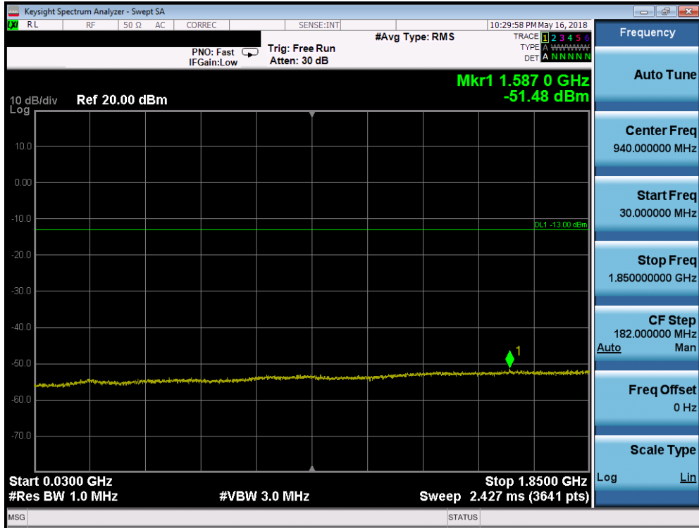
Plot 7-187. Conducted Spurious Plot (Band 25/2 - 20.0MHz QPSK - RB Size 1, RB Offset 0 - High Channel)
