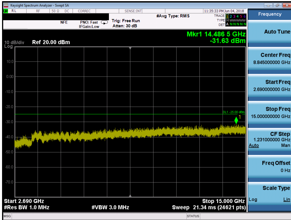
Plot 7-224. Conducted Spurious Plot (Band 41/38 - 20.0MHz QPSK - RB Size 1, RB Offset 0 - Mid Channel)
