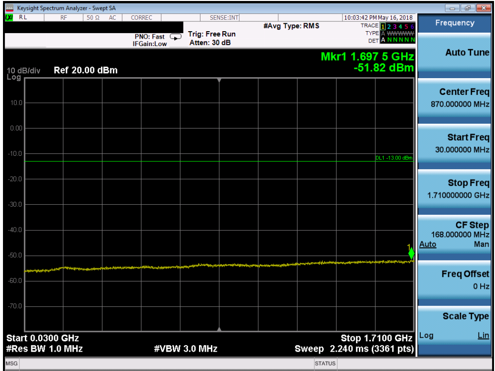
Plot 7-178. Conducted Spurious Plot (Band 66/4 - 20.0MHz QPSK - RB Size 1, RB Offset 0 - High Channel)
