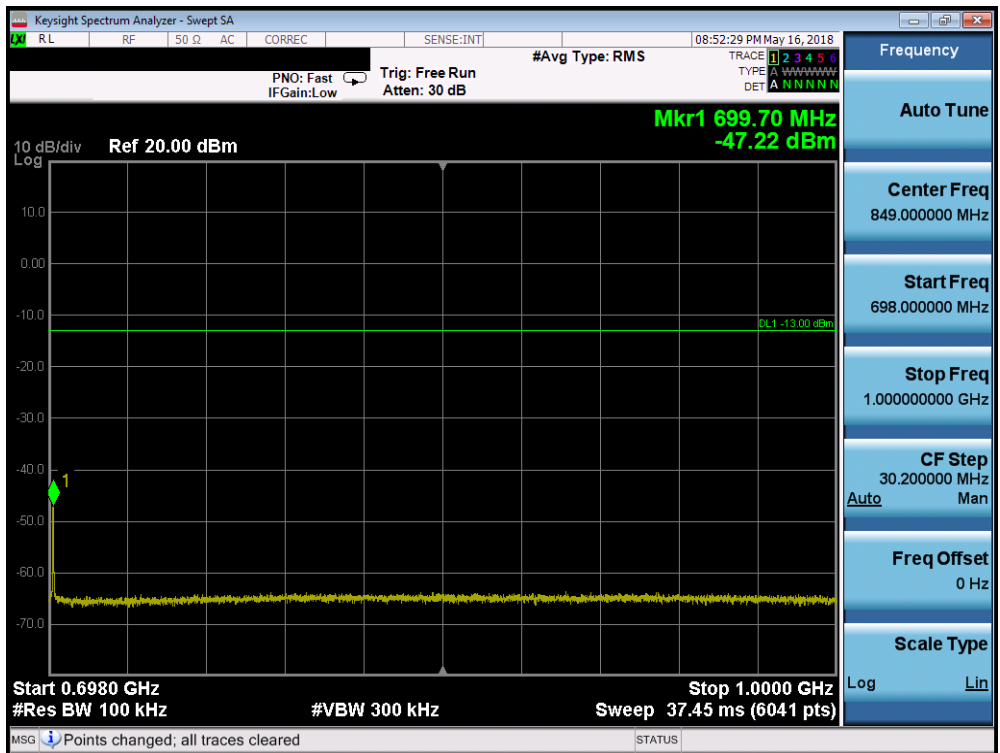
Plot 7-143. Conducted Spurious Plot (Band 71 - 20.0MHz QPSK - RB Size 1, RB Offset 0 - Low Channel)
