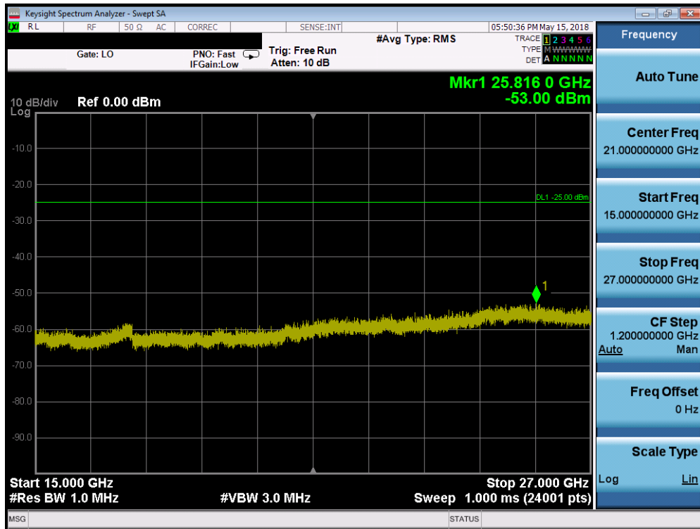
Plot 7-231. Conducted Spurious Plot (Band 41 - 20.0MHz QPSK - RB Size 1, RB Offset 0 - Low Channel)
