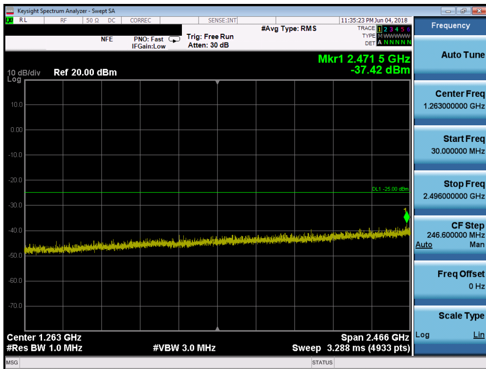
Plot 7-223. Conducted Spurious Plot (Band 41/38 - 20.0MHz QPSK - RB Size 1, RB Offset 0 - Mid Channel)
