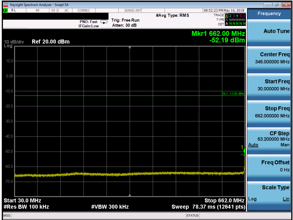
Plot 7-142. Conducted Spurious Plot (Band 71 - 20.0MHz QPSK - RB Size 1, RB Offset 0 - Low Channel)
