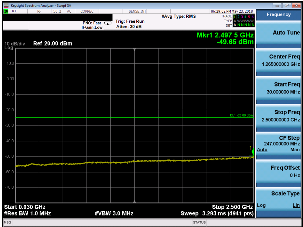
Plot 7-208. Conducted Spurious Plot (Band 7 - 15.0MHz QPSK - RB Size 1, RB Offset 0 - High Channel)
