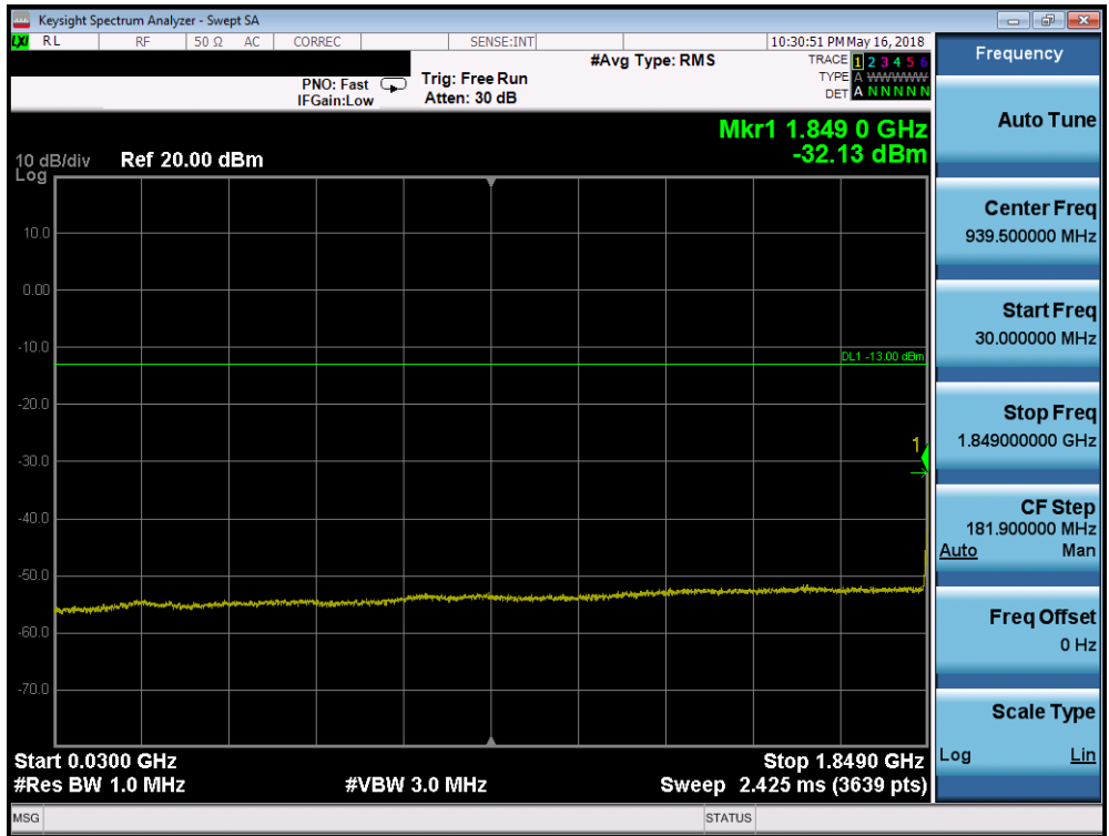
Plot 7-181. Conducted Spurious Plot (Band 25/2 - 20.0MHz QPSK - RB Size 1, RB Offset 0 - Low Channel)
