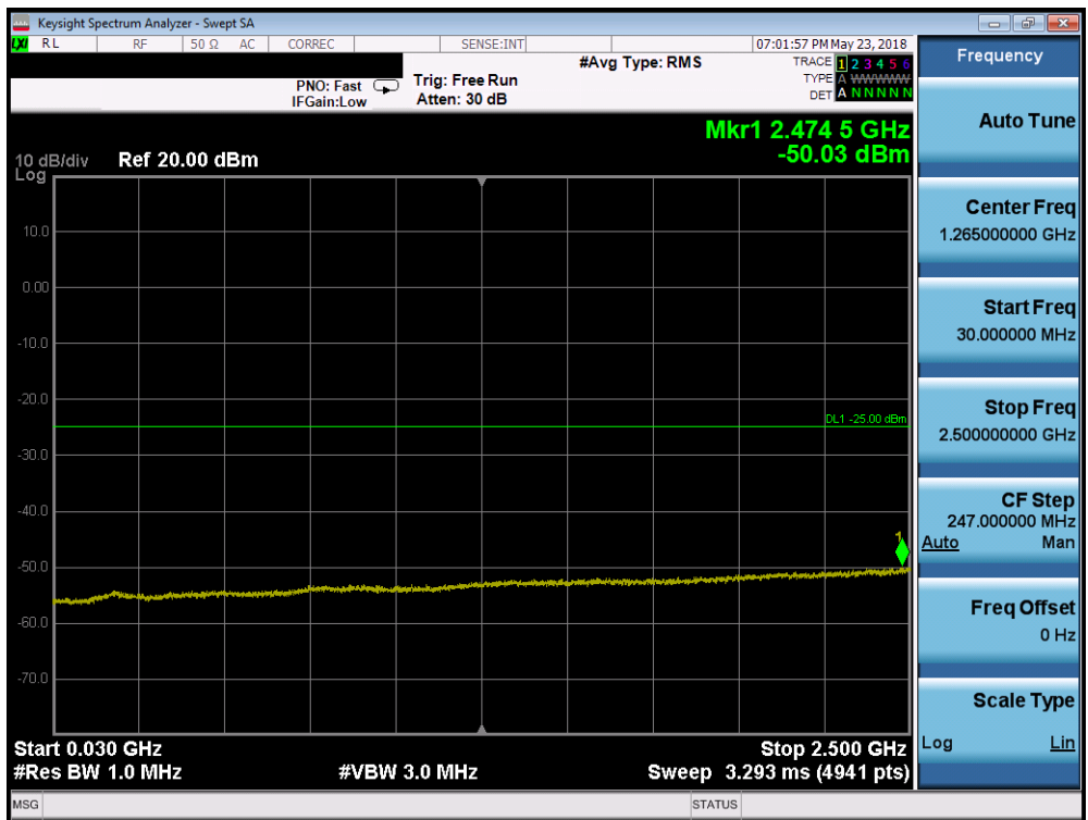
Plot 7-214. Conducted Spurious Plot (Band 7 - 15.0MHz QPSK - RB Size 1, RB Offset 0 - Mid Channel)
