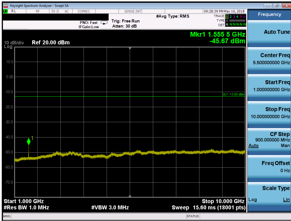
Plot 7-162. Conducted Spurious Plot (Band 13 - 10.0MHz QPSK - RB Size 1, RB Offset 0)
