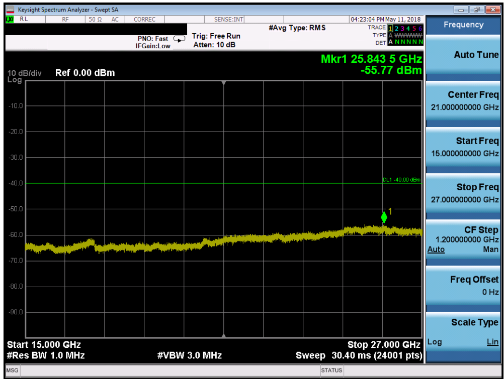
Plot 7-195. Conducted Spurious Plot (Band 30 - 5.0MHz QPSK - RB Size 1, RB Offset 0 - Low Channel)
