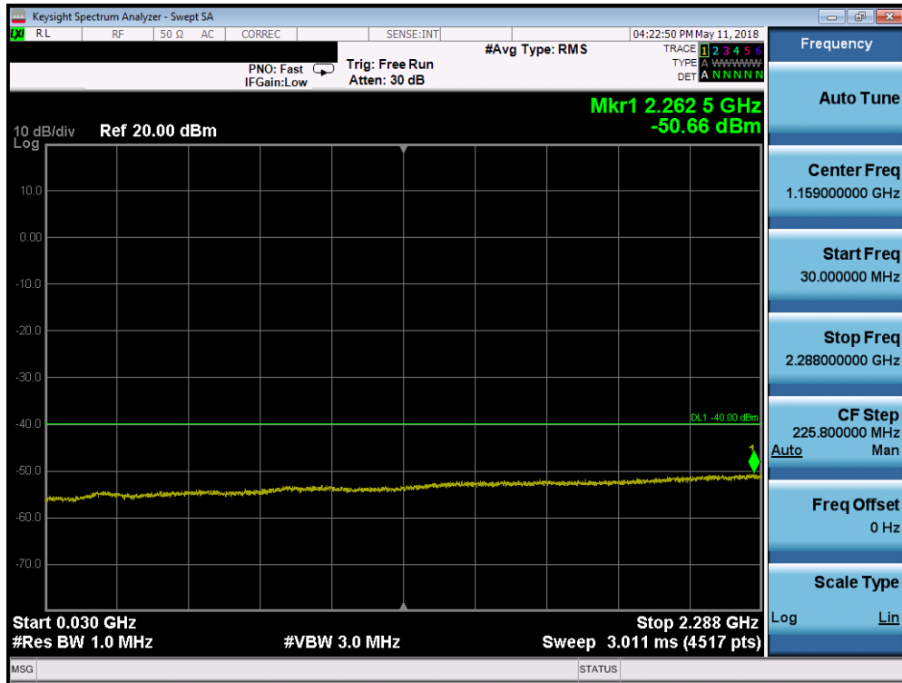
Plot 7-193. Conducted Spurious Plot (Band 30 - 5.0MHz QPSK - RB Size 1, RB Offset 0 - Low Channel)
