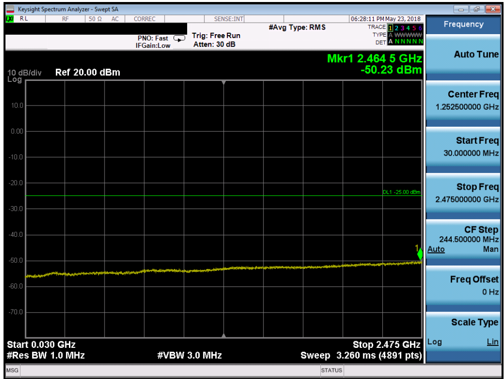
Plot 7-202. Conducted Spurious Plot (Band 7 - 15.0MHz QPSK - RB Size 1, RB Offset 0 - Low Channel)
