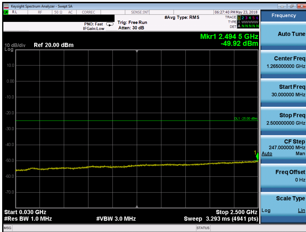
Plot 7-205. Conducted Spurious Plot (Band 7 - 15.0MHz QPSK - RB Size 1, RB Offset 0 - Mid Channel)
