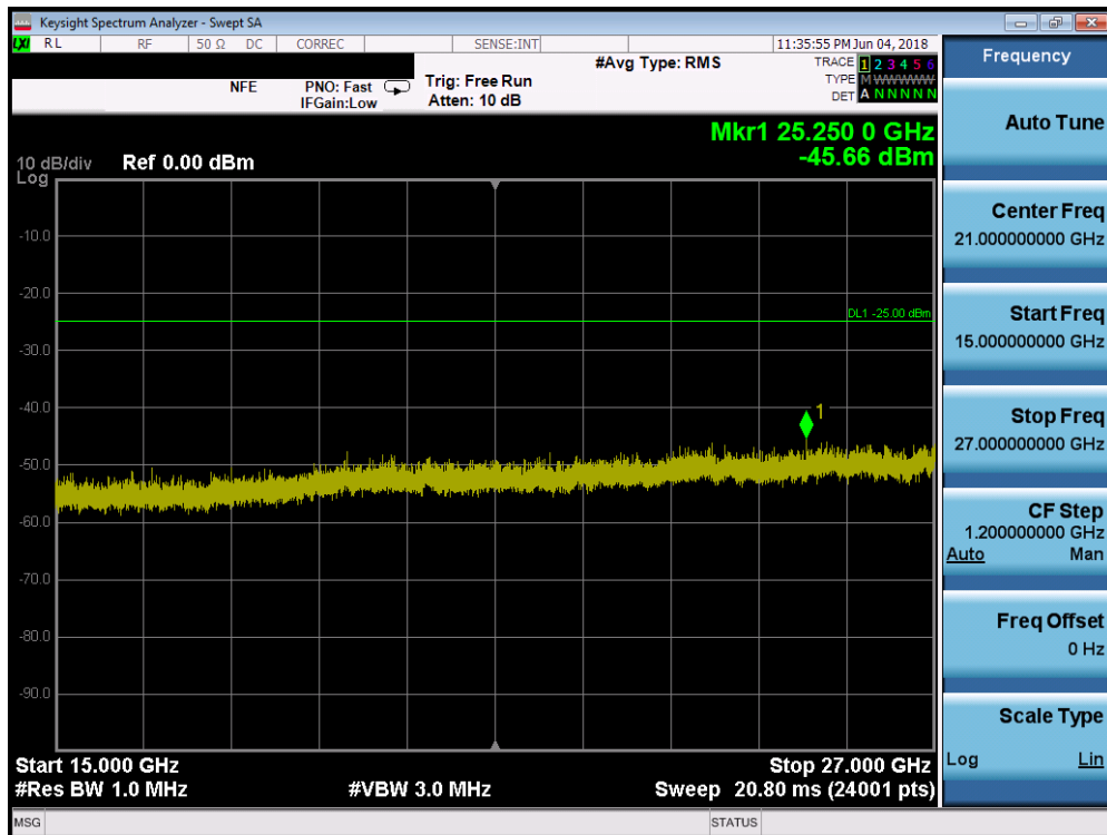
Plot 7-225. Conducted Spurious Plot (Band 41/38 - 20.0MHz QPSK - RB Size 1, RB Offset 0 - Mid Channel)
