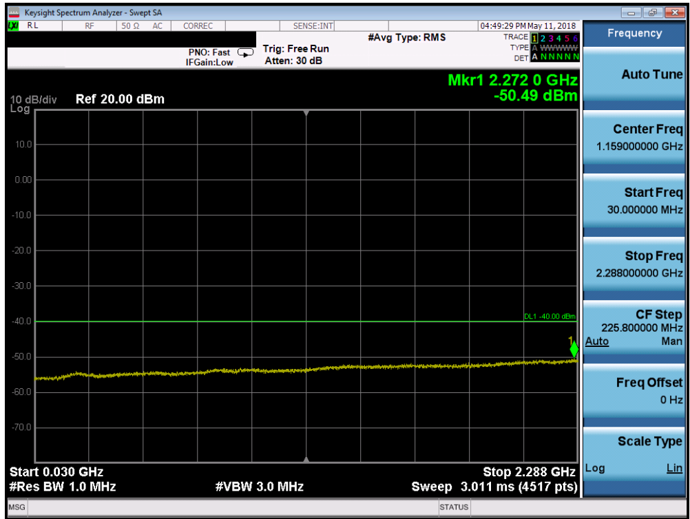
Plot 7-190. Conducted Spurious Plot (Band 30 - 10.0MHz QPSK - RB Size 1, RB Offset 0 - Mid Channel)
