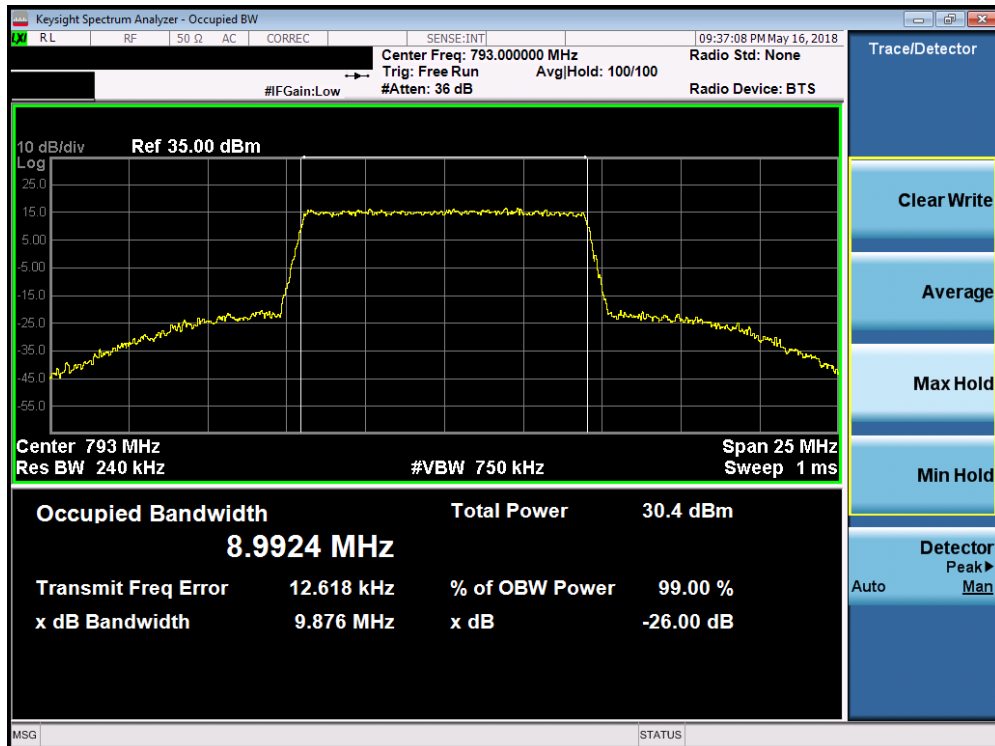
Plot 7-8. Occupied Bandwidth Plot (LTE Band 14 – 10MHz 64QAM – Full RB Configuration)
