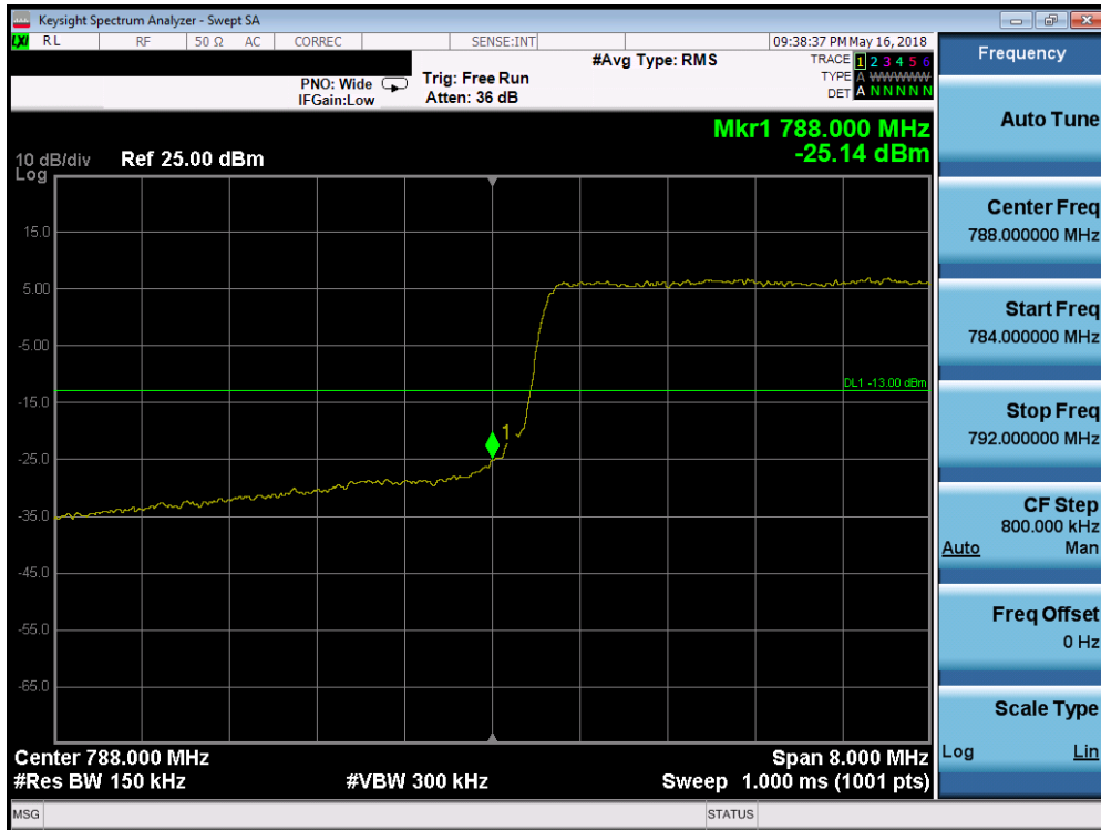
Plot 7-42. Lower Band Edge Plot (LTE Band 14 – 10MHz QPSK – Full RB Configuration)
