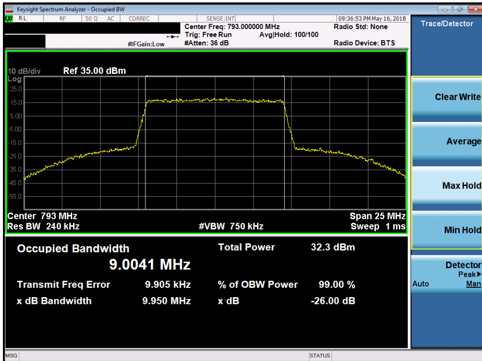
Plot 7-6. Occupied Bandwidth Plot (LTE Band 14 – 10MHz QPSK – Full RB Configuration)
