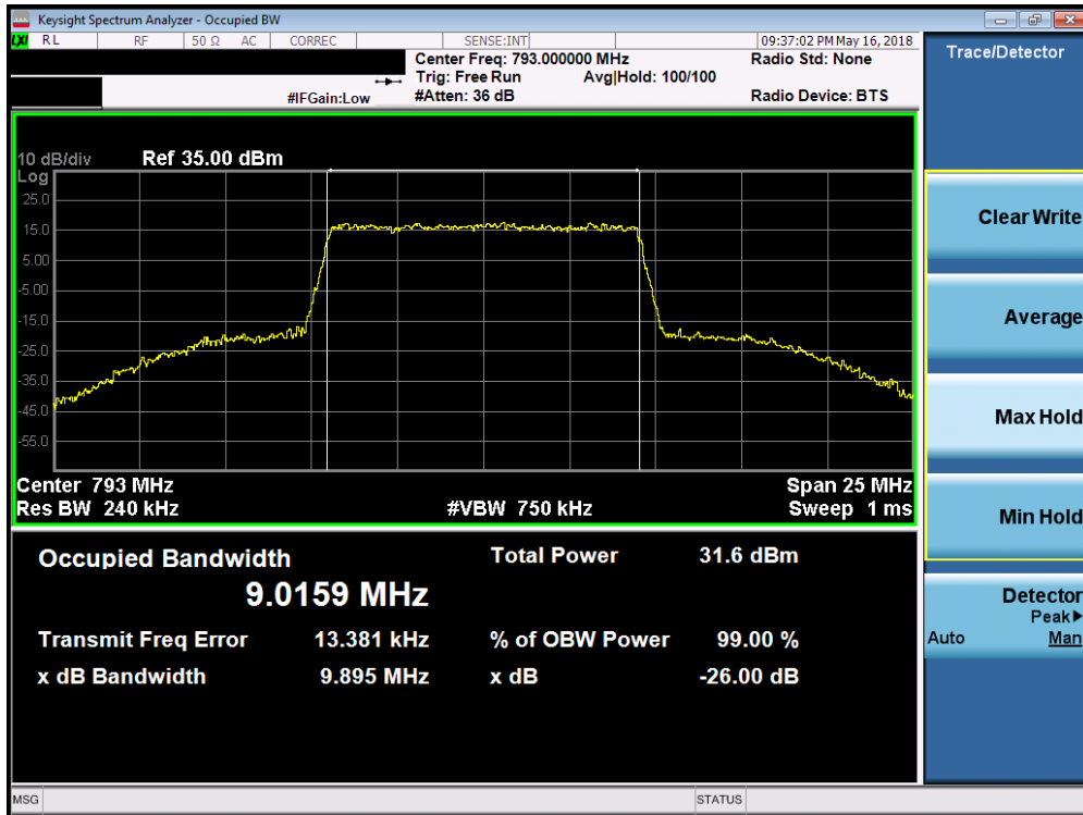
Plot 7-7. Occupied Bandwidth Plot (LTE Band 14 – 10MHz 16QAM – Full RB Configuration)
