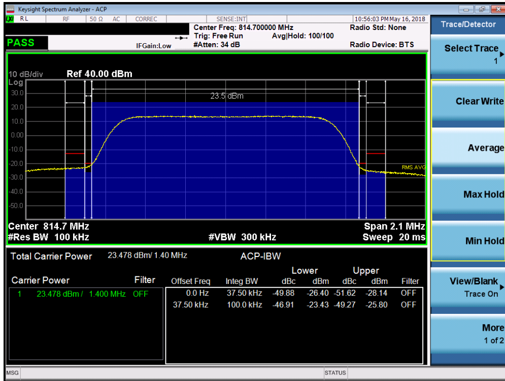
Plot 7-46. Channel Edge Plot (LTE Band 26 – 1.4MHz QPSK – RB Size 6– Low Channel)
