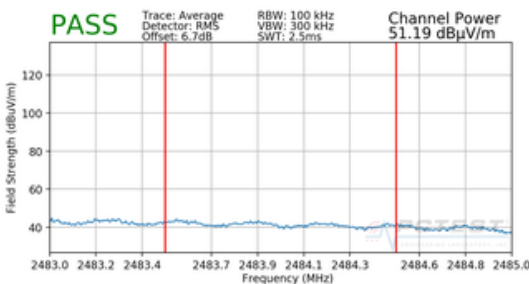
Plot 7-83. Radiated Restricted Upper Band Edge Measurement MIMO (Average)
