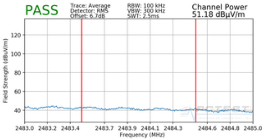
Plot 7-85. Radiated Restricted Band Edge Measurement MIMO with WCP (Average)
