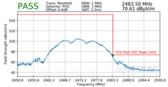
Plot 7-92. Radiated Restricted Band Edge Measurement CDD with WCP (Peak)
