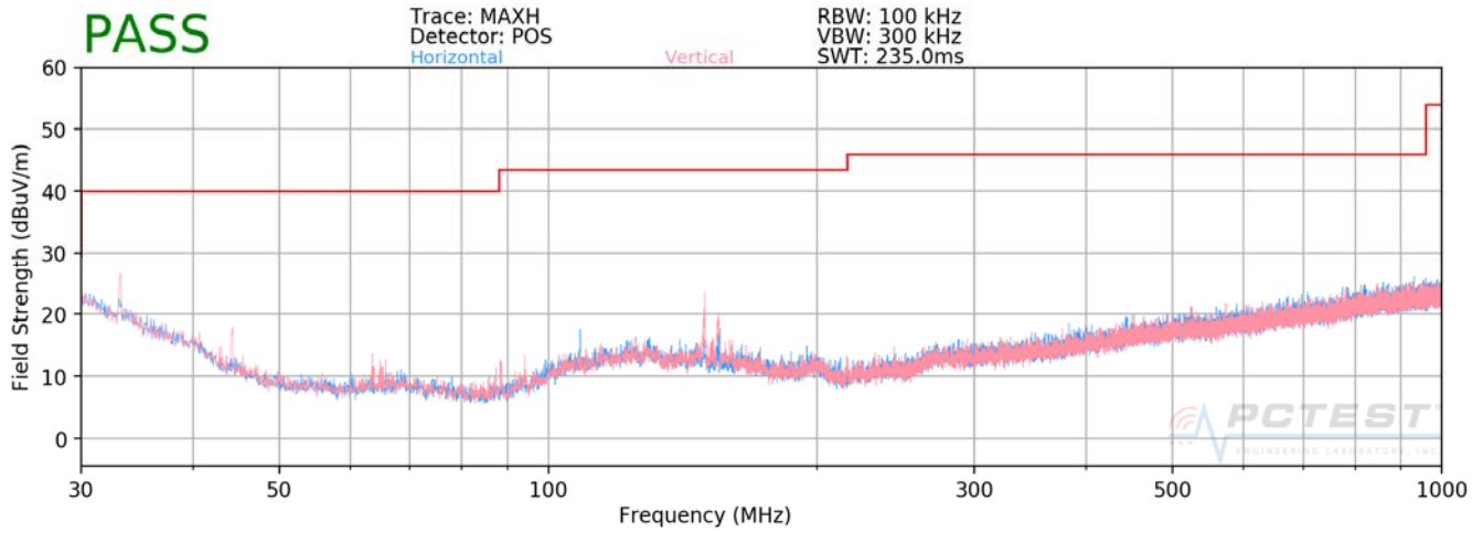
Plot 7-93. Radiated Spurious Plot below 1GHz SISO ANT1
