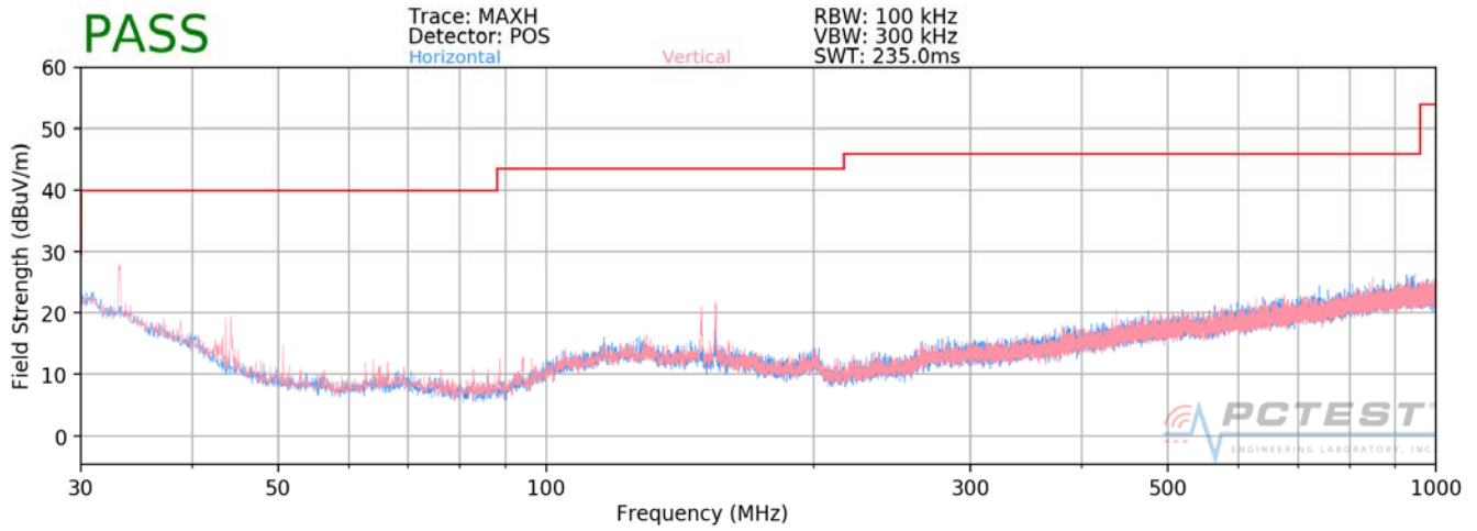
Plot 7-94. Radiated Spurious Plot below 1GHz SISO ANT2
