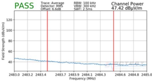
Plot 7-91. Radiated Restricted Band Edge Measurement CDD with WCP (Average)
