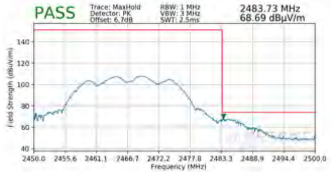
Plot 7-106. Radiated Restricted Upper Band Edge Measurement CDD (Peak)
