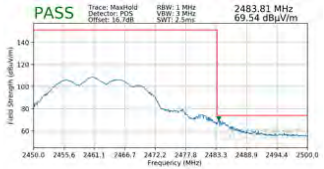
Plot 7-110. Radiated Restricted Band Edge Measurement CDD with WCP (Peak)
