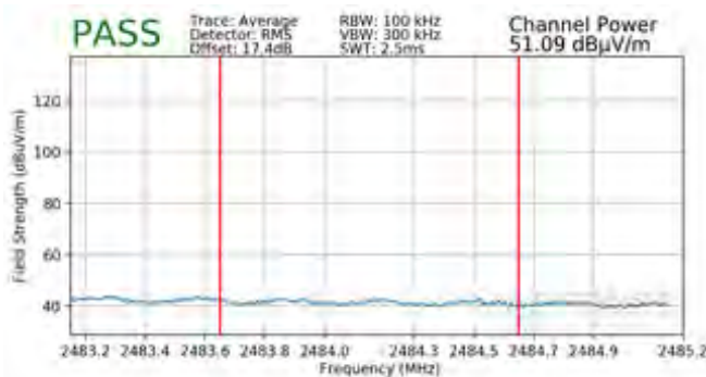
Plot 7-83. Radiated Restricted Upper Band Edge Measurement SISO ANT1 (Average)
