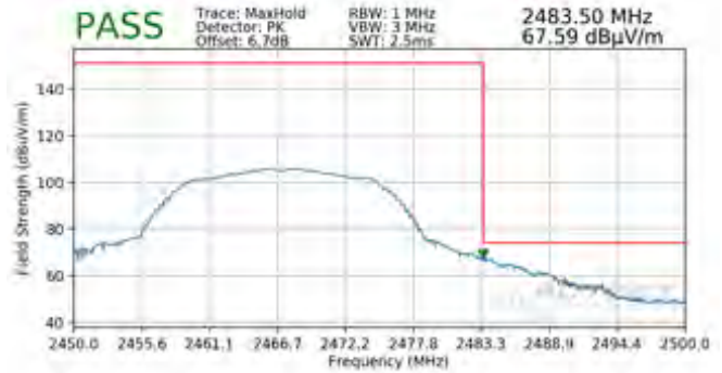
Plot 7-86. Radiated Restricted Band Edge Measurement SISO ANT1 (Peak)
