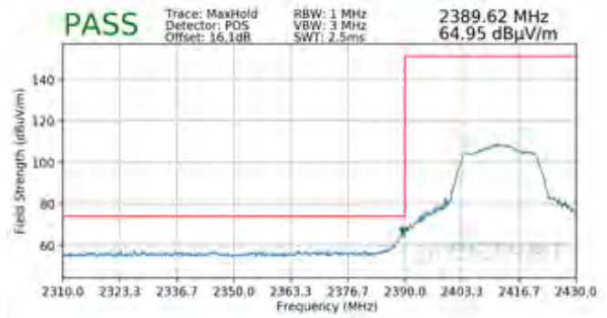
Plot 7-120. Radiated Restricted Band Edge Measurement MIMO with WCP (Peak)
