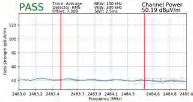
Plot 7-85. Radiated Restricted Band Edge Measurement SISO ANT1 (Average)
