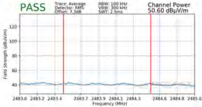
Plot 7-95. Radiated Restricted Upper Band Edge Measurement SISO ANT2 (Average)
