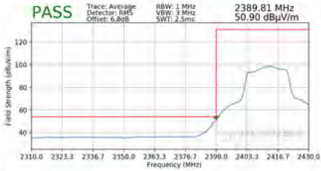
Plot 7-89. Radiated Restricted Band Edge Measurement SISO ANT1 with WCP (Average)
