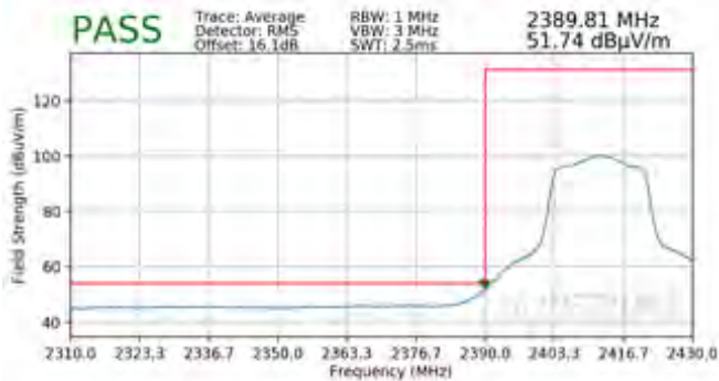
Plot 7-111. Radiated Restricted Lower Band Edge Measurement MIMO (Average)
