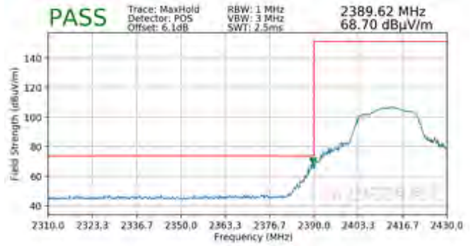
Plot 7-90. Radiated Restricted Band Edge Measurement SISO ANT1 with WCP (Peak)
