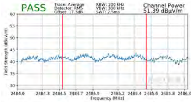
Plot 7-109. Radiated Restricted Band Edge Measurement CDD with WCP (Average)
