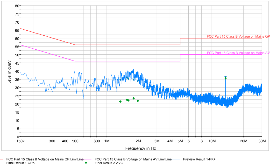
Plot 7-2. Line-Conducted Test Plot (N)
