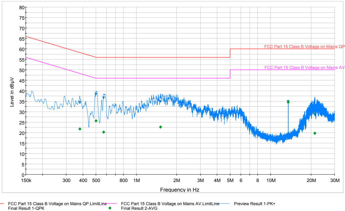
Plot 7-1. Line-Conducted Test Plot (L1)
