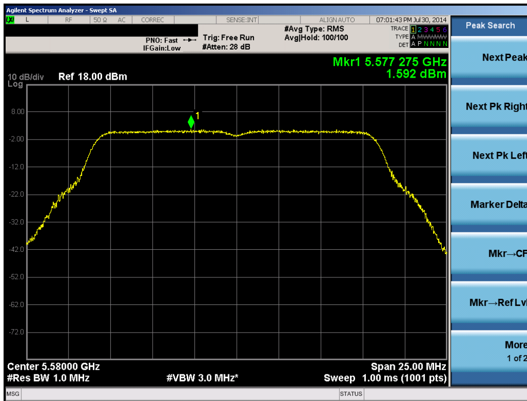
Plot 6-116. Peak Power Spectral Density Plot (802.11a (UNII Band 2C) – Ch. 116)
