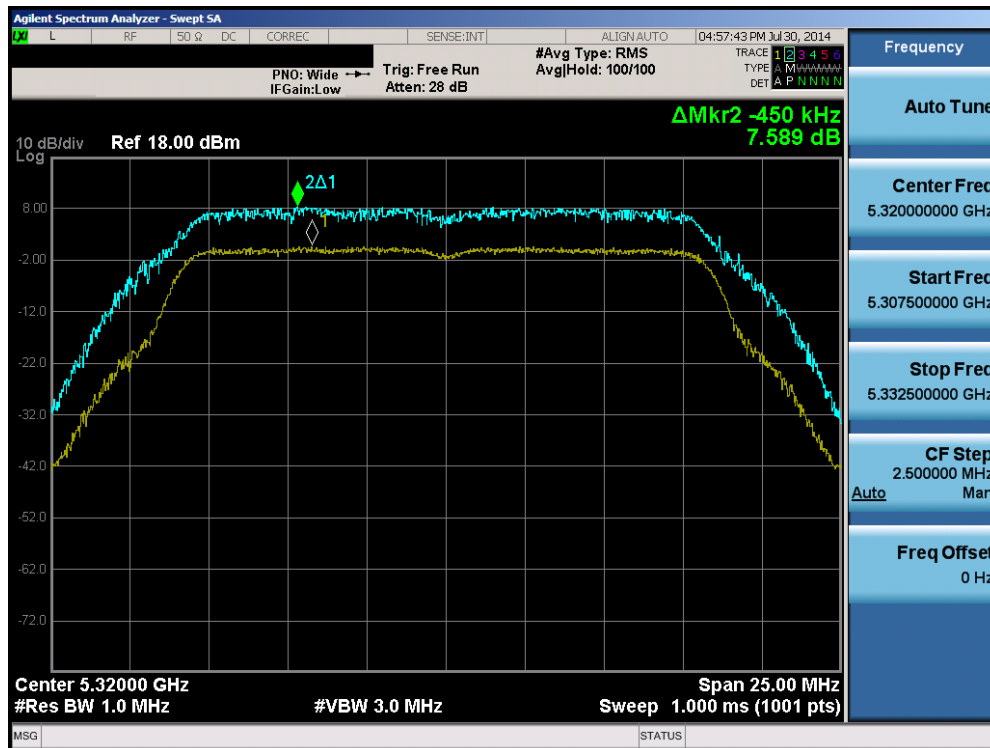
Plot 6-125. Peak Excursion Ratio Plot (802.11a (UNII Band 2A) – Ch. 64)
