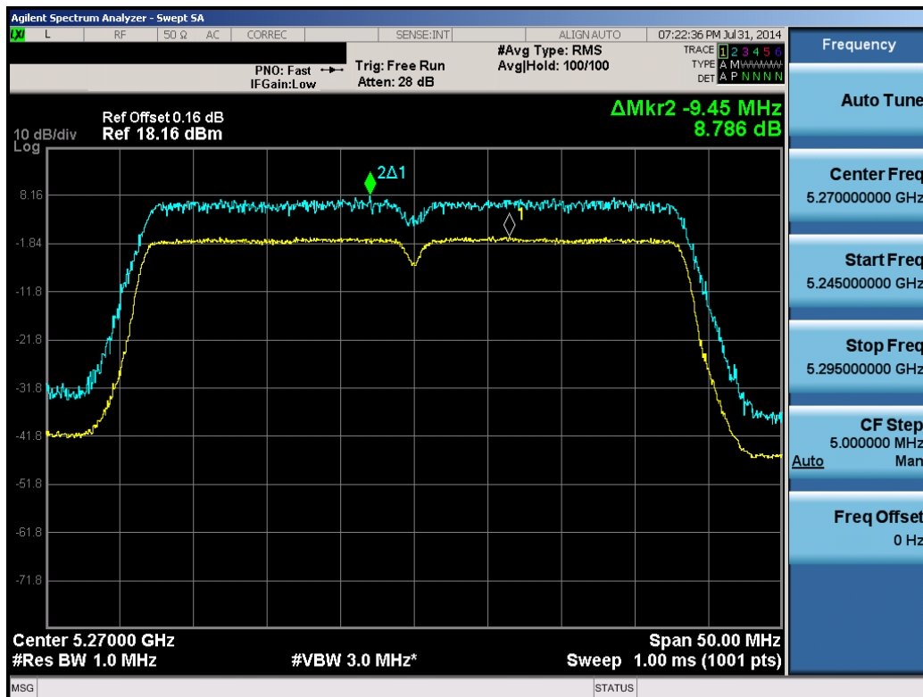
Plot 6-131. Peak Excursion Ratio Plot (40MHz BW 802.11n (UNII Band 2A) – Ch. 54)
