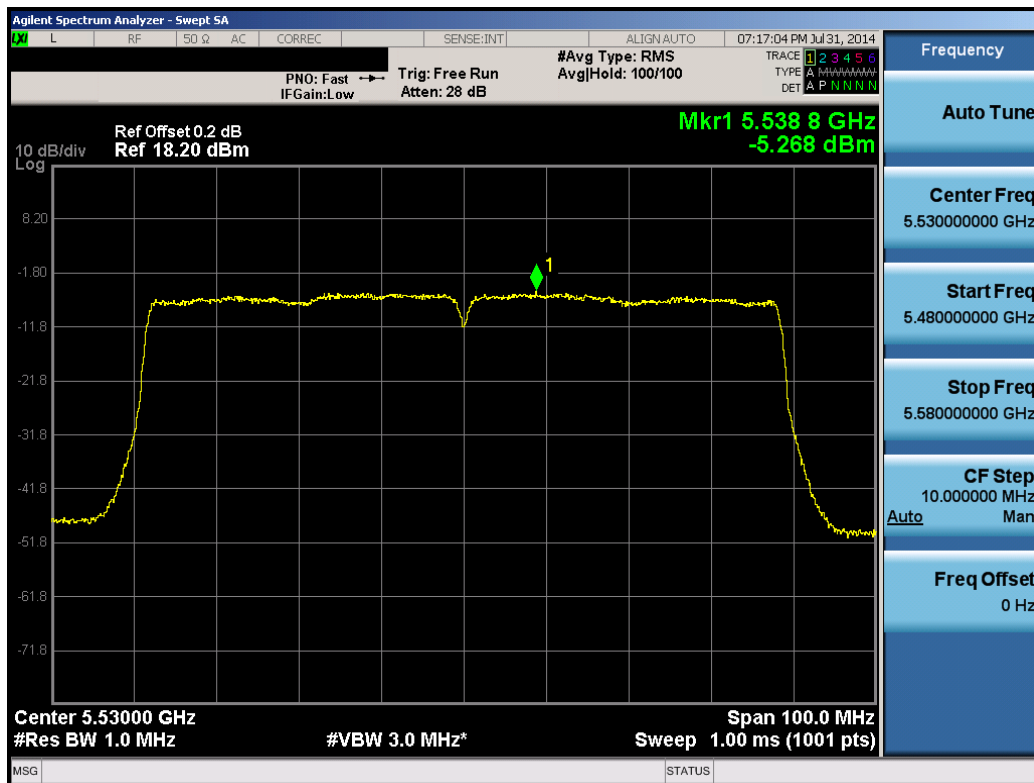
Plot 6-124. Peak Power Spectral Density Plot (80MHz BW 802.11a/n/ac (UNII Band 2C) – Ch. 106)
