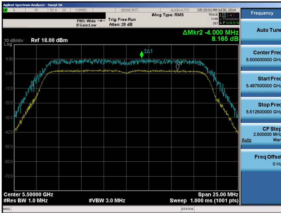
Plot 6-127. Peak Excursion Ratio Plot (20MHz BW 802.11n (UNII Band 2C) – Ch. 100)
