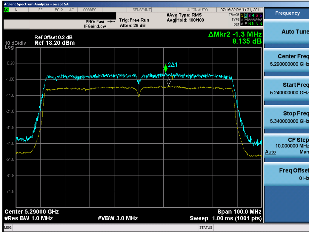
Plot 6-132. Peak Excursion Ratio Plot (80MHz BW 802.11ac (UNII Band 2A) – Ch. 58)
