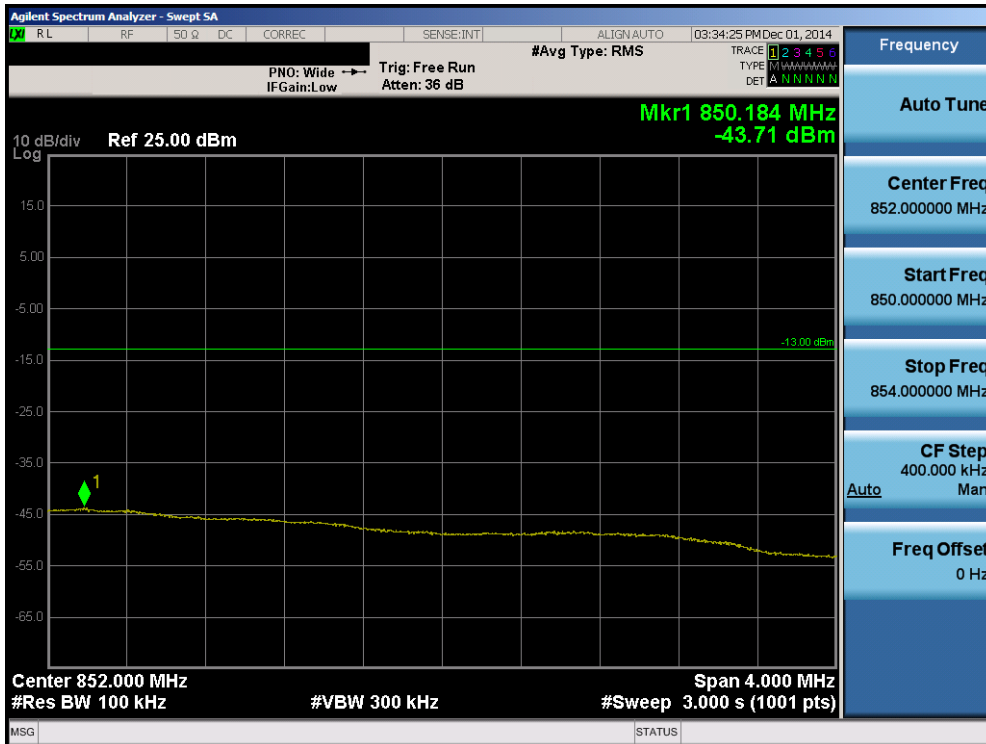
Plot 6-42. Upper Extended Band Edge Plot (Band 5 – 5.0MHz QPSK – RB Size 25)
