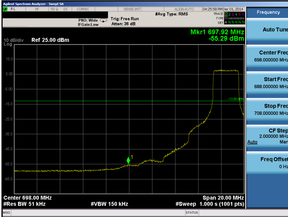
Plot 6-25. Lower Band Edge Plot (Band 17 – 5.0MHz QPSK – RB Size 25)
