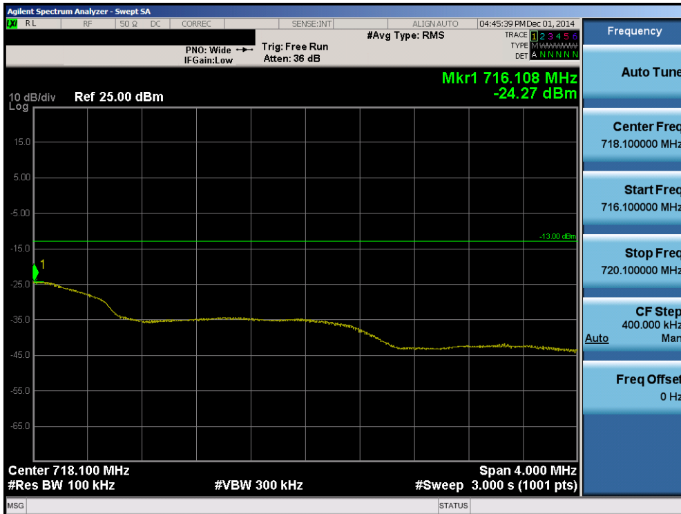
Plot 6-28. Upper Extended Band Edge Plot (Band 17 – 5.0MHz QPSK – RB Size 25)
