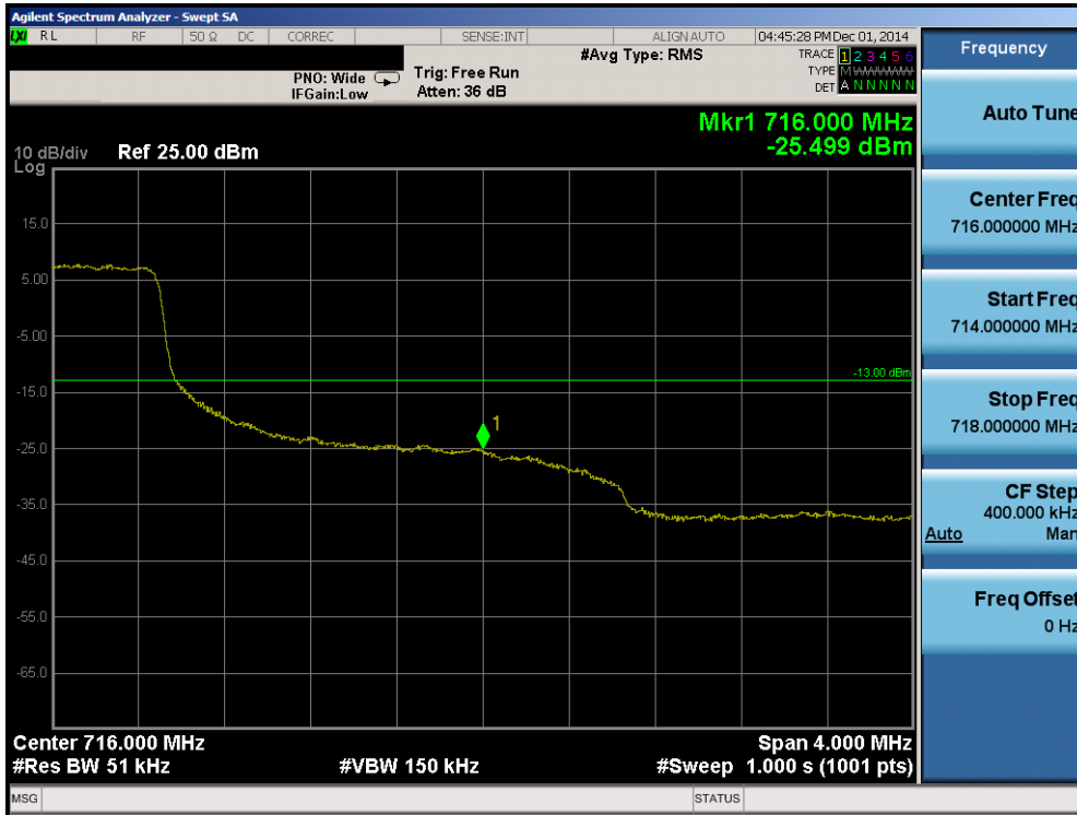
Plot 6-27. Upper Band Edge Plot (Band 17 – 5.0MHz QPSK – RB Size 25)
