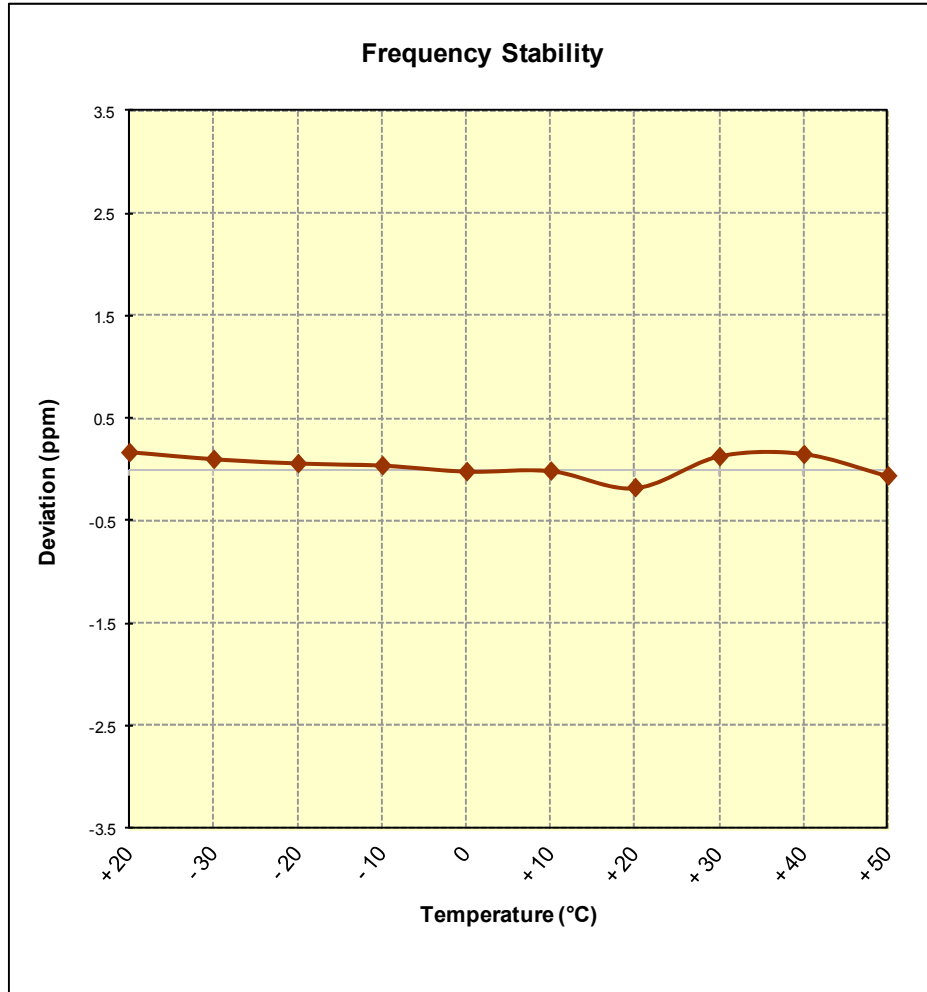
Figure 6-9. Frequency Stability Graph (PCS WCDMA Mode – Ch. 9400)
