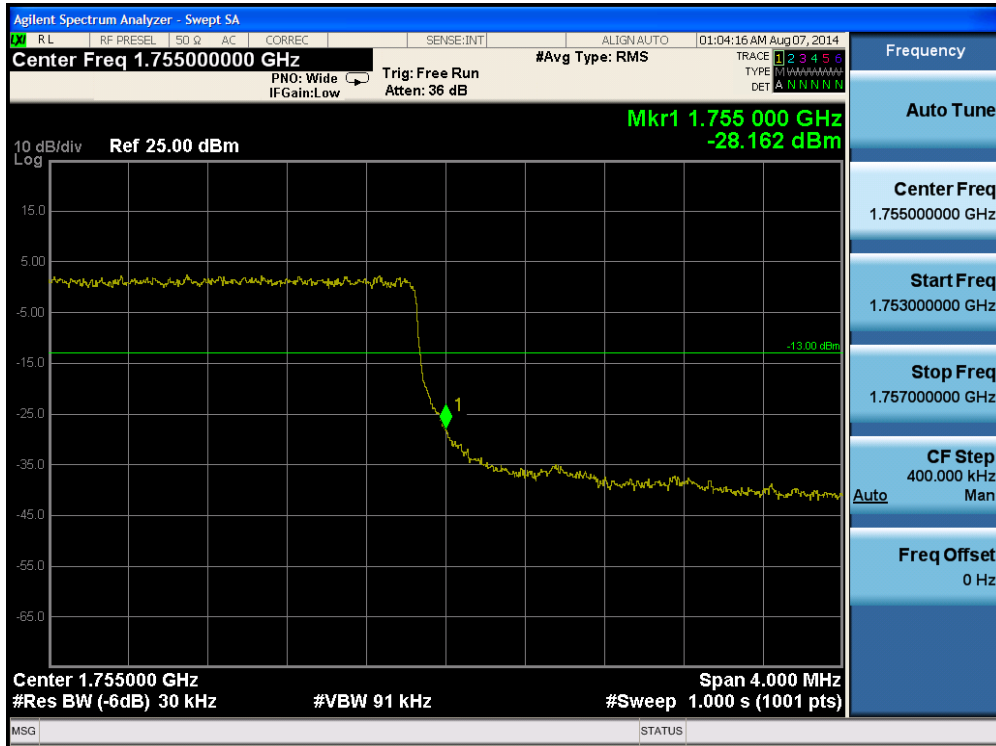
Plot 6-65. Upper Band Edge Plot (Band 4 – 3.0MHz QPSK – RB Size 15)
