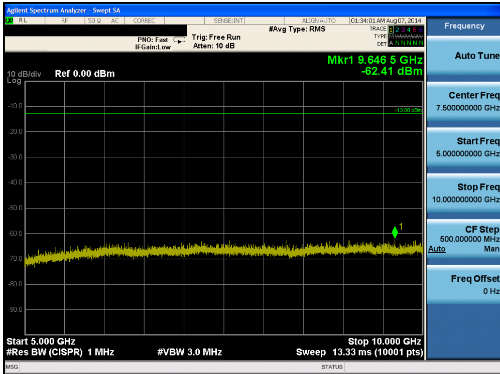
Plot 6-38. Conducted Spurious Plot (Band 5 – 10.0MHz QPSK – RB Size 1, RB Offset 0 – High Channel)
