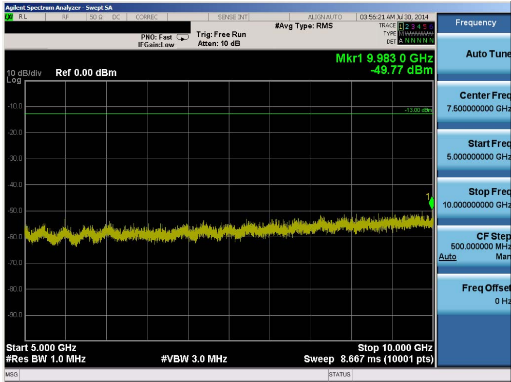
Plot 6-36. Conducted Spurious Plot (Band 5 – 10.0MHz QPSK – RB Size 1, RB Offset 0 – Mid Channel)
