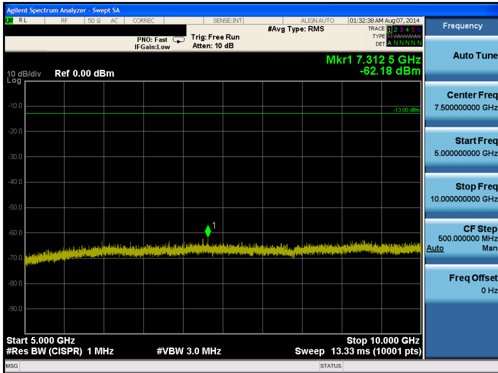
Plot 6-34. Conducted Spurious Plot (Band 5 – 10.0MHz QPSK – RB Size 1, RB Offset 0 – Low Channel)
