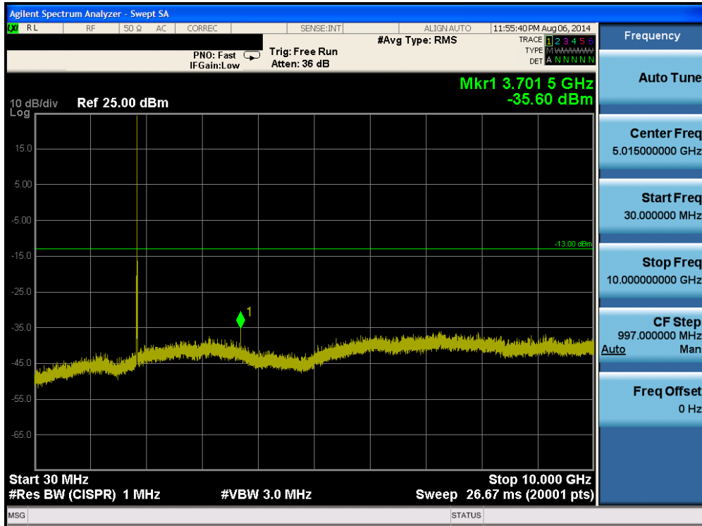
Plot 6-45. Conducted Spurious Plot (Band 2 – 10.0MHz QPSK – RB Size 1, RB Offset 0– Low Channel)
