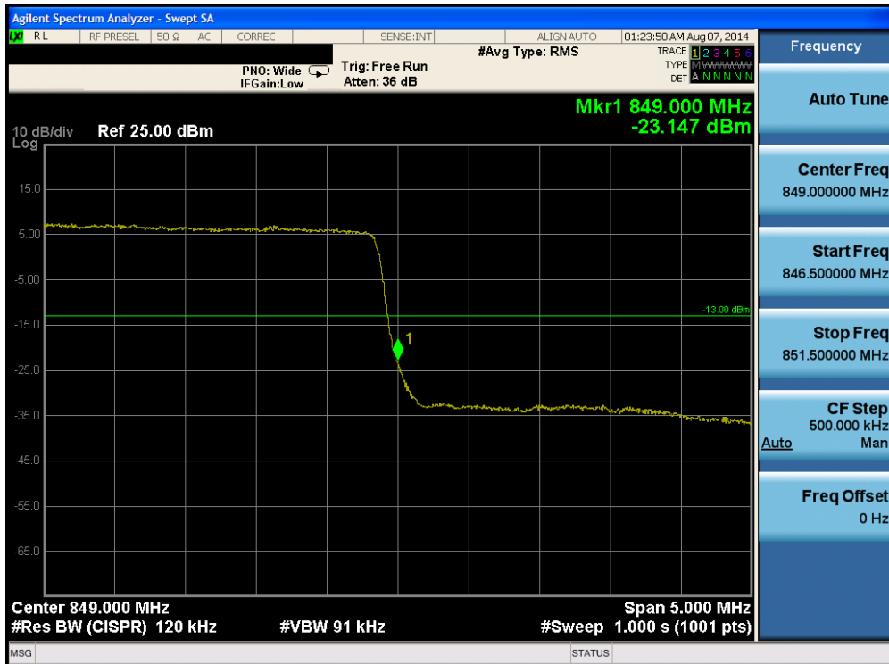
Plot 6-54. Upper Band Edge Plot (Band 5 – 3.0MHz QPSK – RB Size 15)
