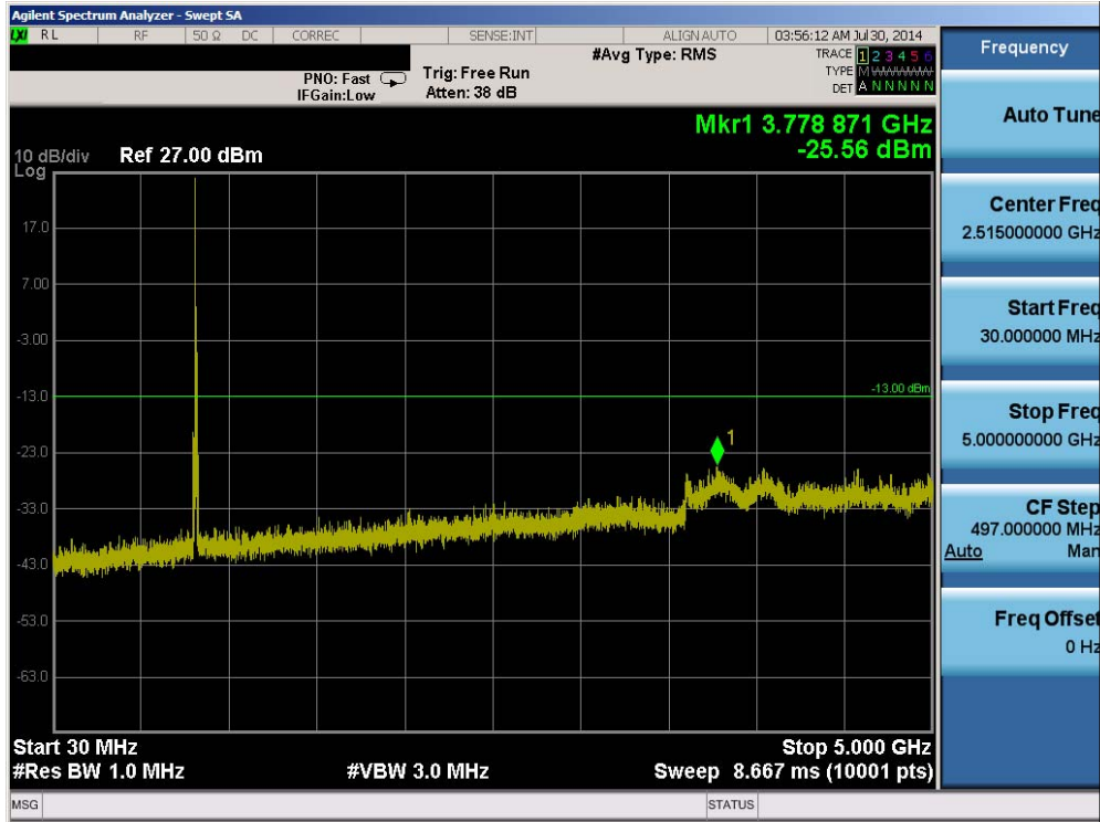
Plot 6-35. Conducted Spurious Plot (Band 5 – 10.0MHz QPSK – RB Size 1, RB Offset 0 – Mid Channel)
