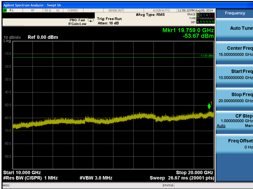
Plot 6-46. Conducted Spurious Plot (Band 2 – 10.0MHz QPSK – RB Size 1, RB Offset 0 – Low Channel)
