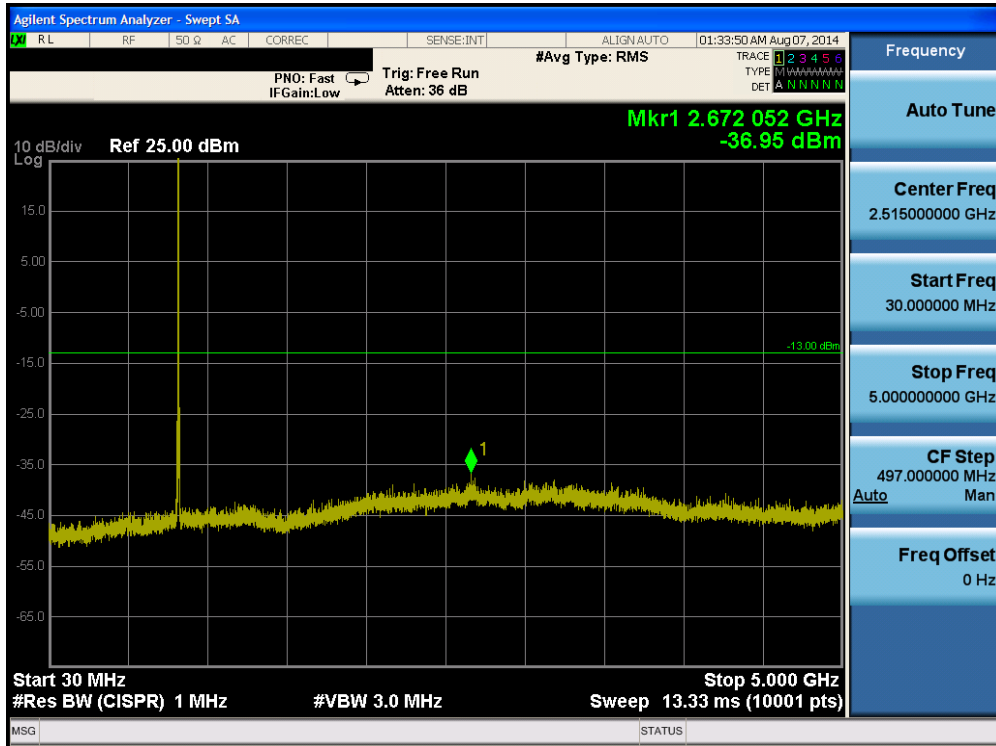
Plot 6-37. Conducted Spurious Plot (Band 5 – 10.0MHz QPSK – RB Size 1, RB Offset 0 – High Channel)
