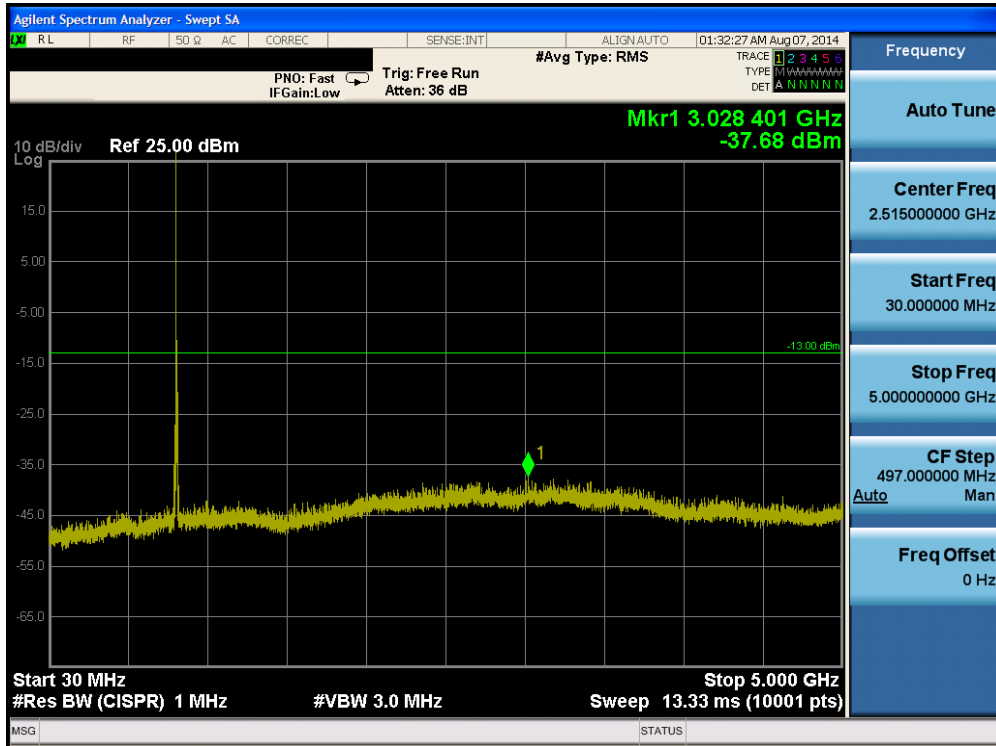
Plot 6-33. Conducted Spurious Plot (Band 5 – 10.0MHz QPSK – RB Size 1, RB Offset 0– Low Channel)
