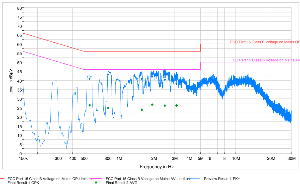
Plot 6-8. Line-Conducted Test Plot (L1)
