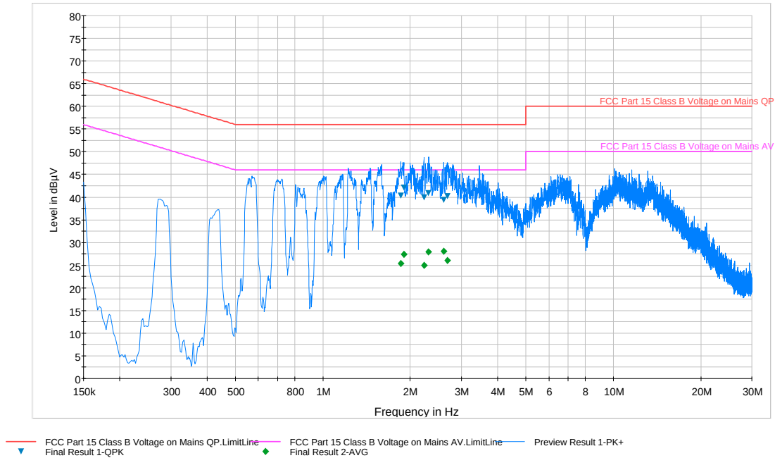
Plot 6-203. Line Conducted Plot with 802.11a UNII Band 2C (N)
