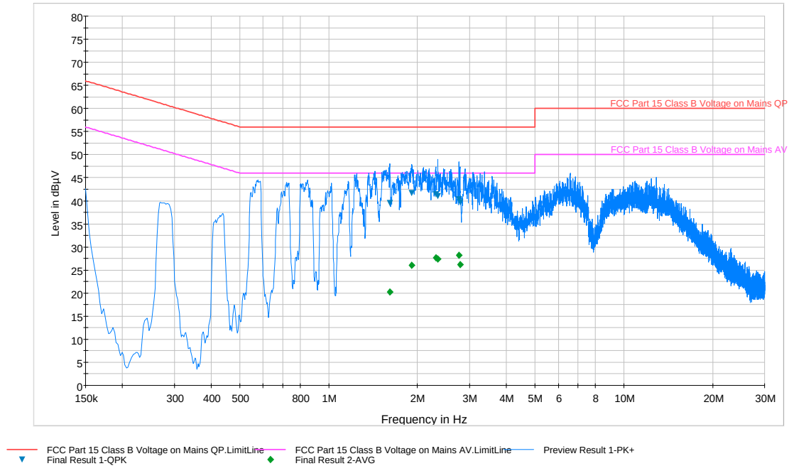
Plot 6-199. Line Conducted Plot with 802.11a UNII Band 1 (N)
