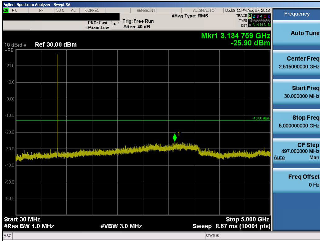
Plot 8-14. Conducted Spurious Plot (10.0MHz QPSK – RB Size 1, RB Offset 0 – High Channel)
