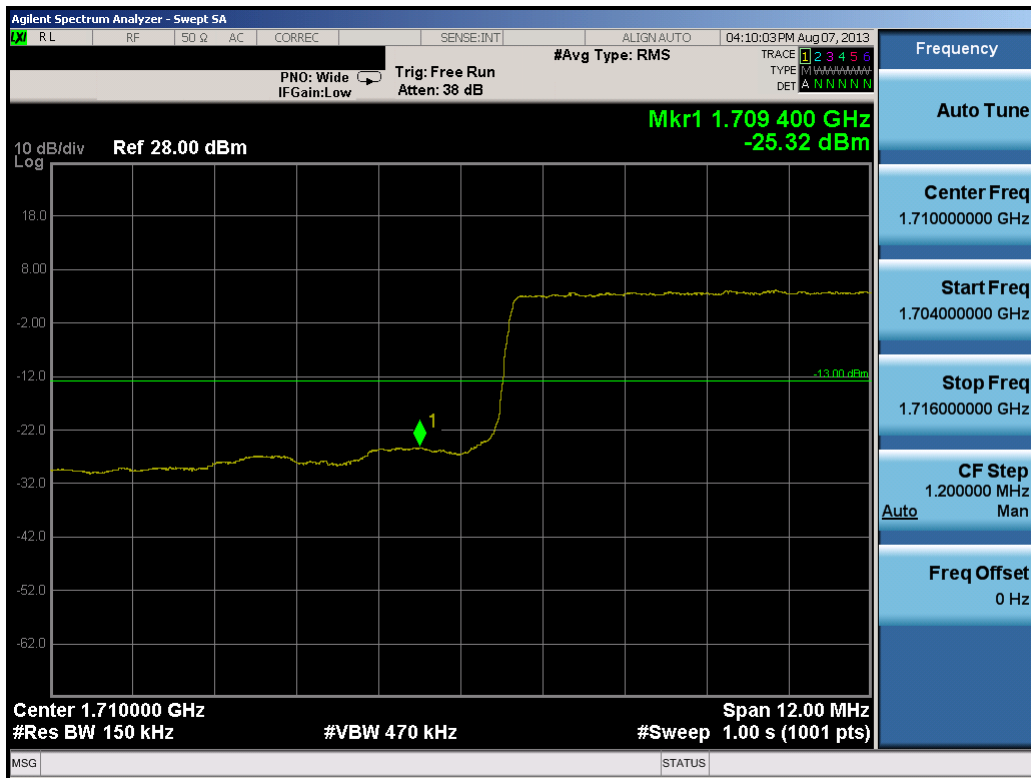
Plot 9-23. Lower Band Edge Plot (15.0MHz QPSK – RB Size 75)
