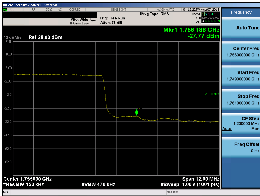
Plot 9-27. Upper Band Edge Plot (15.0MHz QPSK – RB Size 75)
