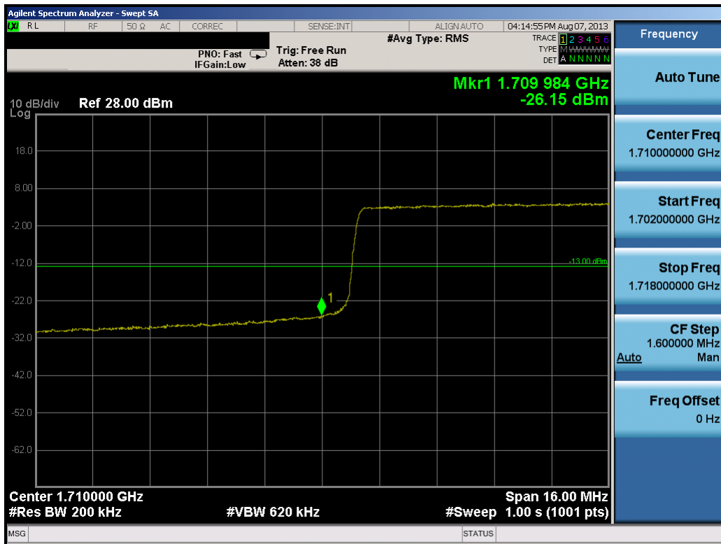
Plot 9-31. Lower Band Edge Plot (20.0MHz QPSK – RB Size 100)
