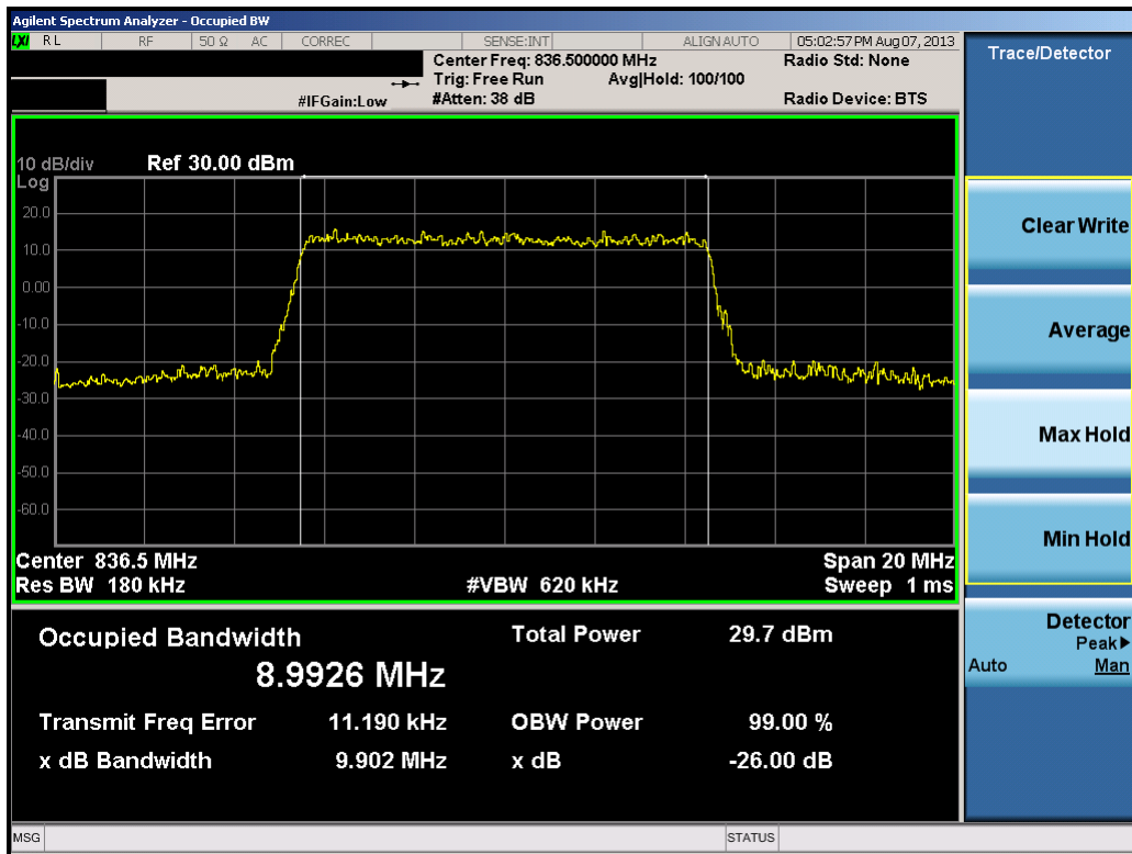
Plot 8-9. Occupied Bandwidth Plot (10.0MHz 16-QAM – RB Size 50)
