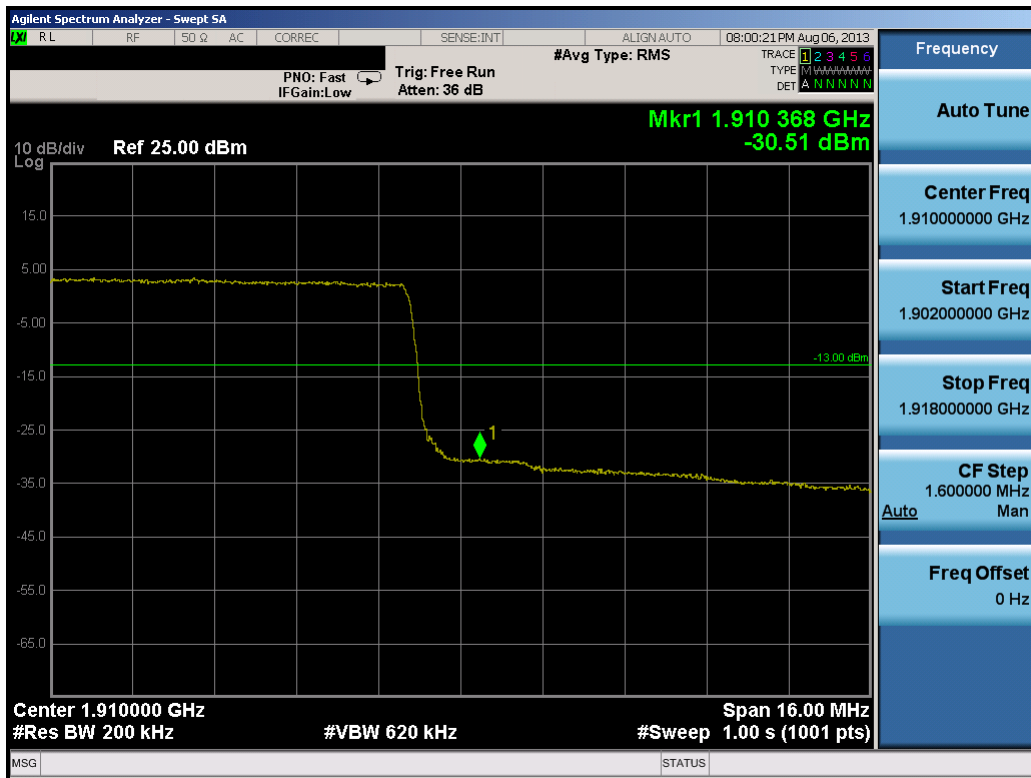
Plot 10-35. Upper Band Edge Plot (20.0MHz QPSK – RB Size 100)
