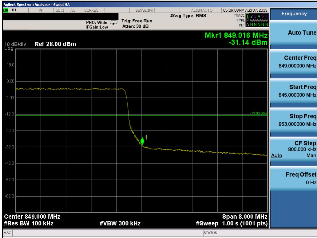
Plot 8-16. Upper Band Edge Plot (10.0MHz QPSK – RB Size 50)
