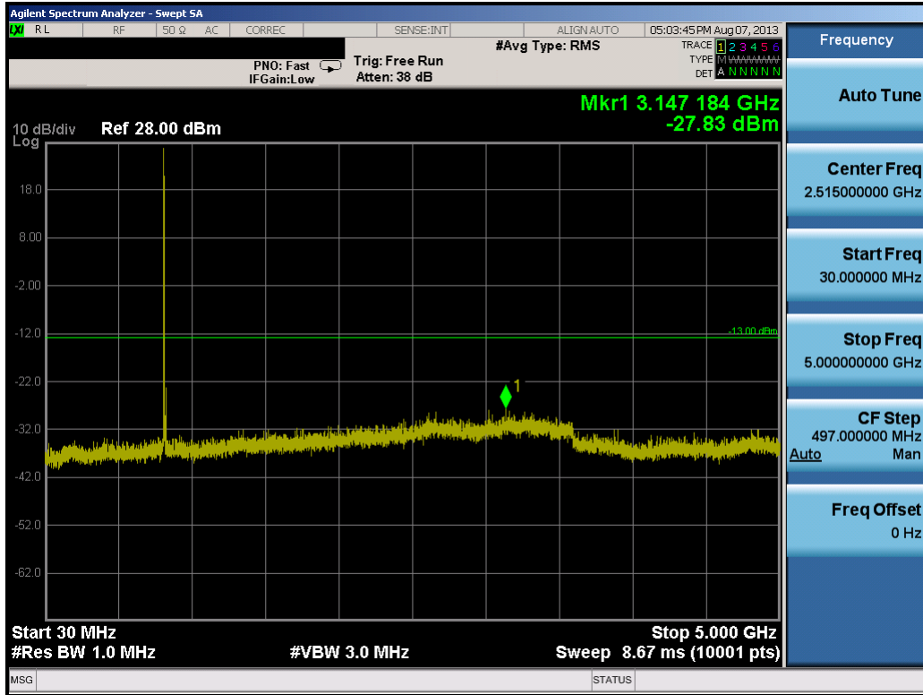
Plot 8-12. Conducted Spurious Plot (10.0MHz QPSK – RB Size 1, RB Offset 0 – Mid Channel)
