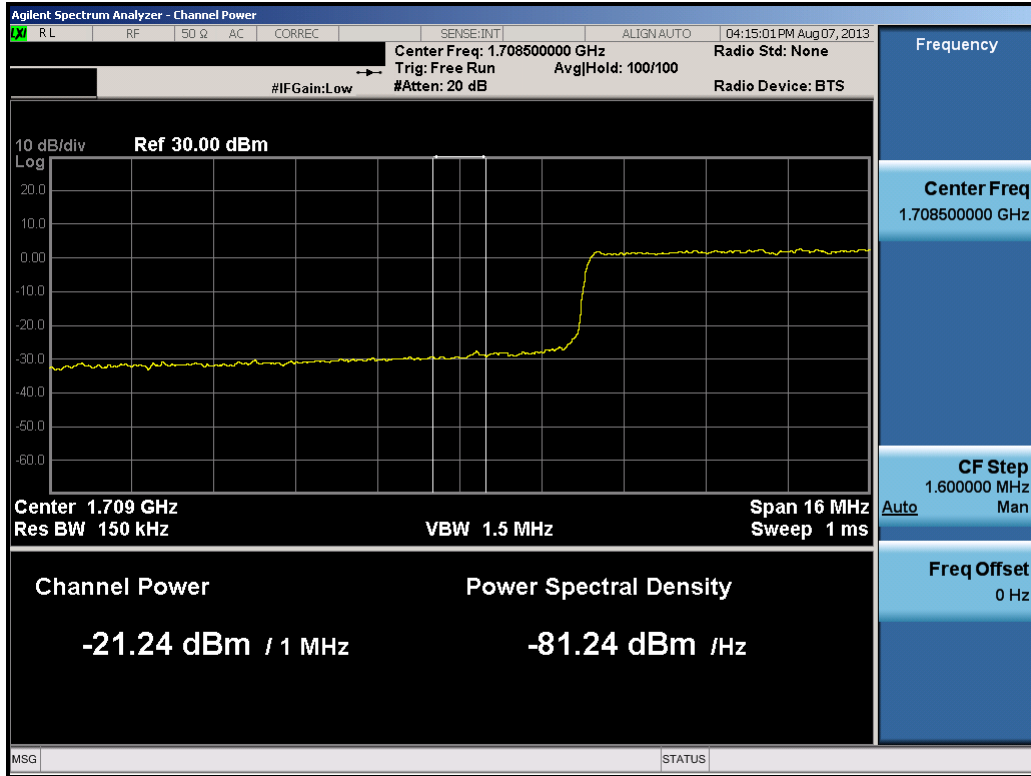
Plot 9-32. Lower Extended Band Edge Plot (20.0MHz QPSK – RB Size 100)
