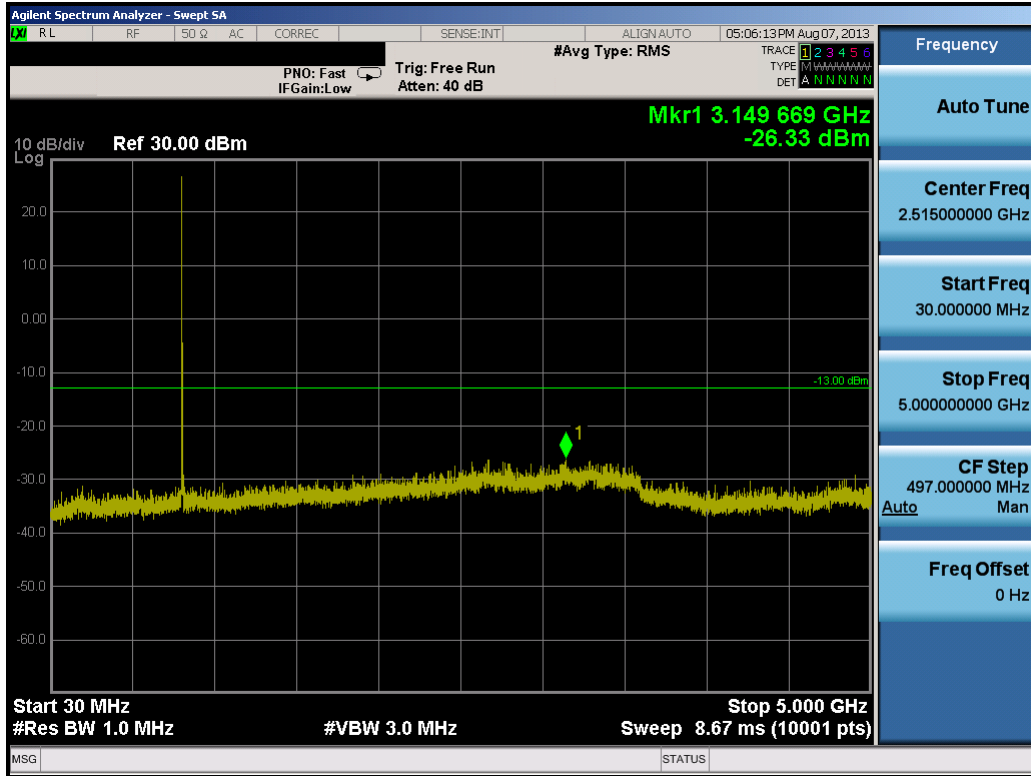
Plot 8-10. Conducted Spurious Plot (10.0MHz QPSK – RB Size 1, RB Offset 0– Low Channel)
