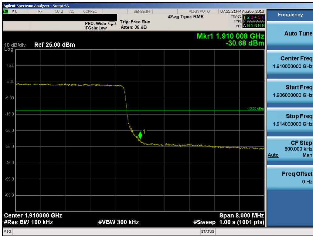
Plot 10-19. Upper Band Edge Plot (10.0MHz QPSK – RB Size 50)
