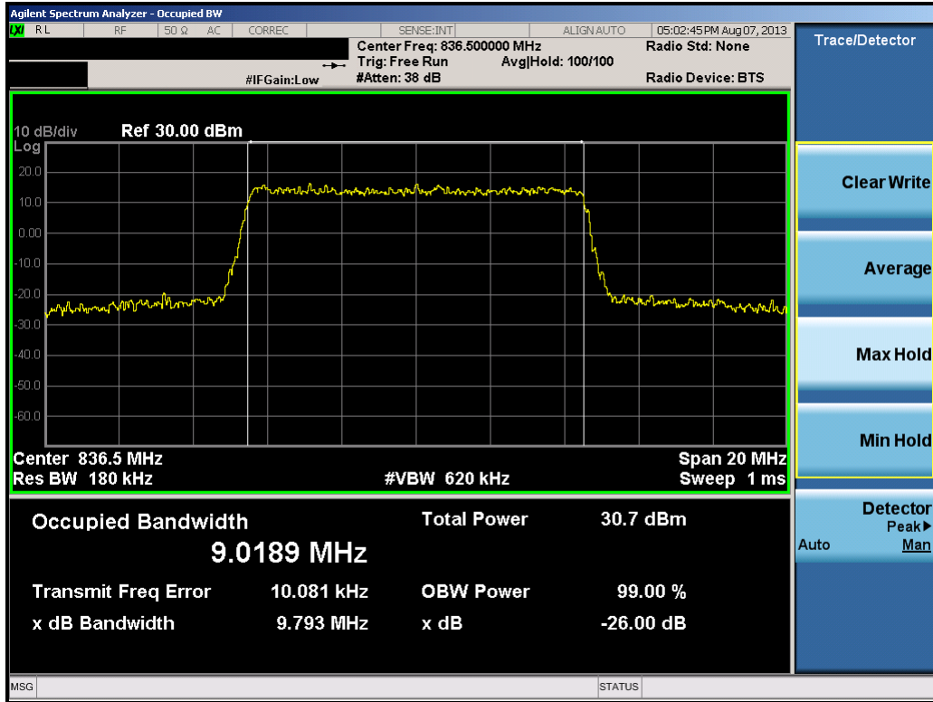
Plot 8-8. Occupied Bandwidth Plot (10.0MHz QPSK – RB Size 50)
