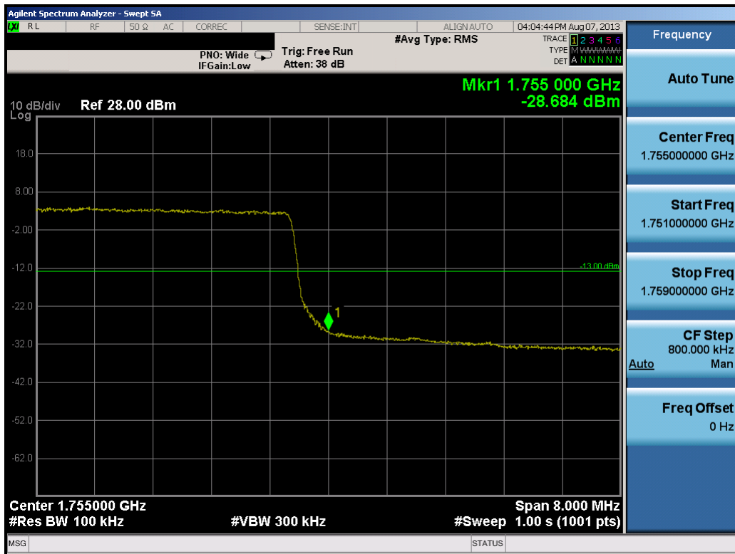
Plot 9-19. Upper Band Edge Plot (10.0MHz QPSK – RB Size 50)
