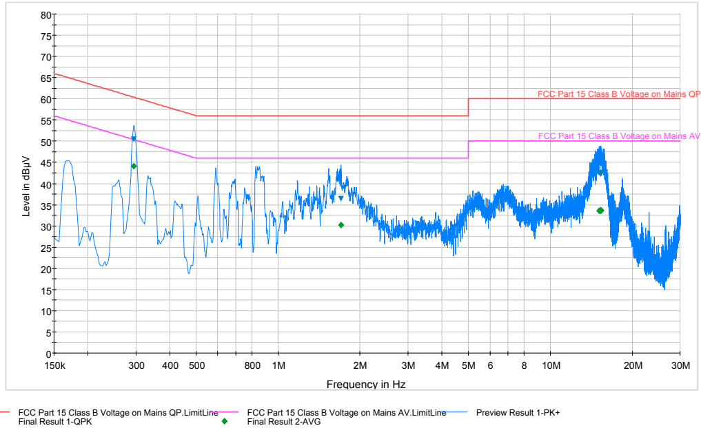
Plot 6-69. Line Conducted Plot with 802.11b (N)
