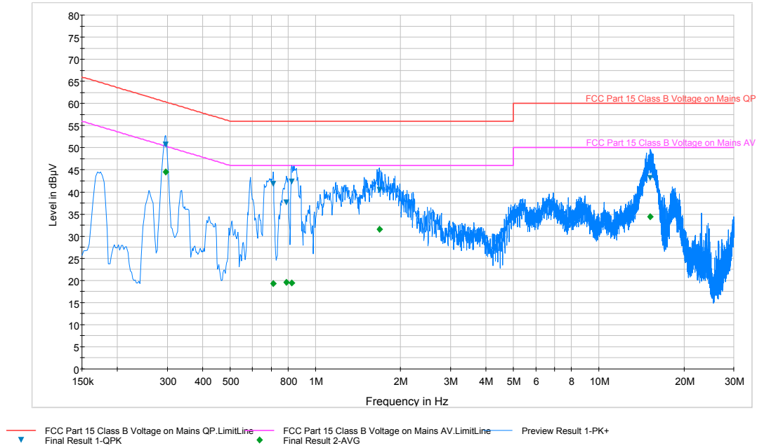
Plot 6-70. Line Conducted Plot with 802.11a (L1)
