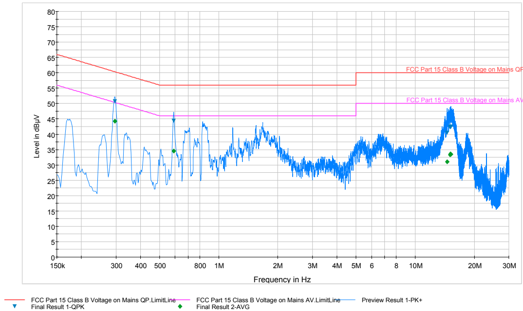
Plot 6-71. Line Conducted Plot with 802.11a (N)
