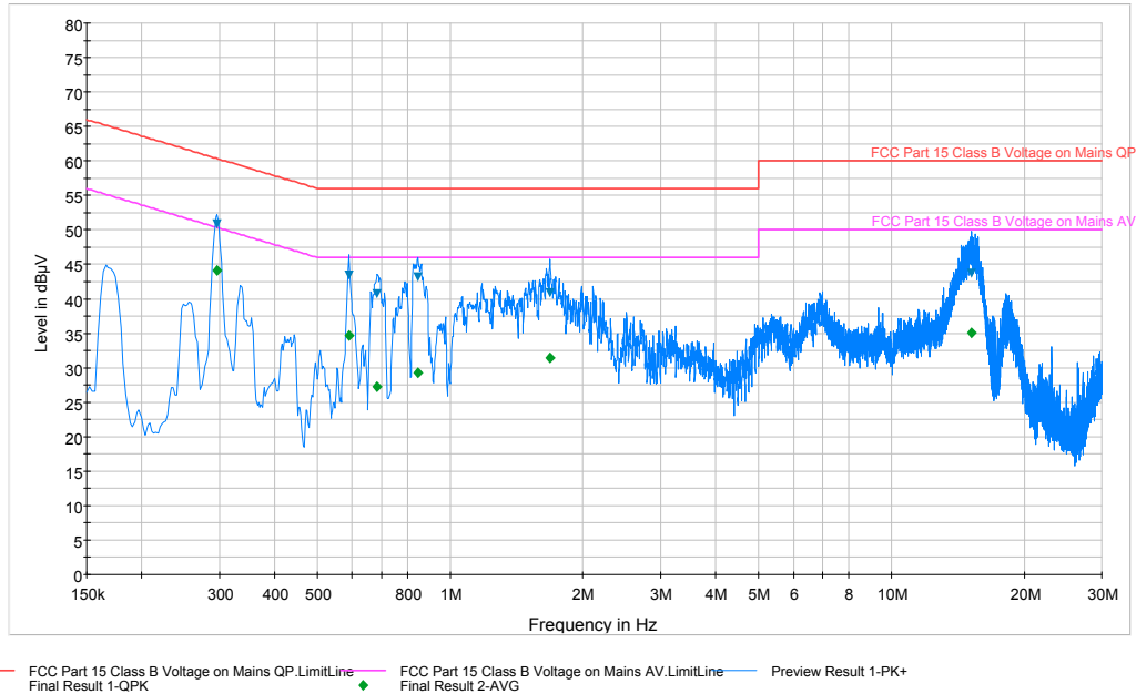
Plot 6-68. Line Conducted Plot with 802.11b (L1)
