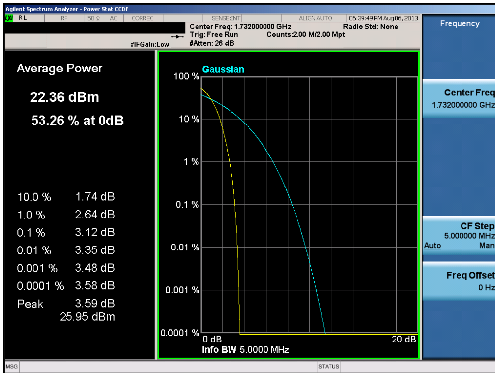
Plot 6-60. Peak-Average Ratio Plot (AWS WCDMA Mode – Ch. 1412)
