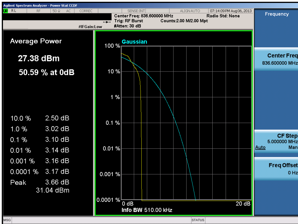
Plot 6-56. Peak-Average Ratio Plot (EDGE850 Mode – Ch. 190)
