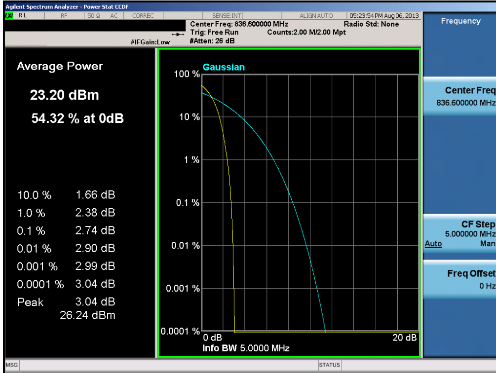
Plot 6-59. Peak-Average Ratio Plot (Cellular WCDMA Mode – Ch. 4183)
