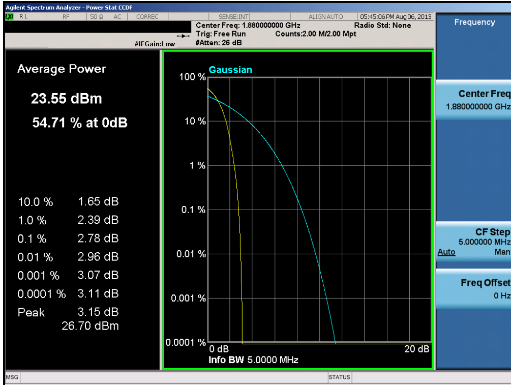
Plot 6-61. Peak-Average Ratio Plot (PCS WCDMA Mode – Ch. 9400)
