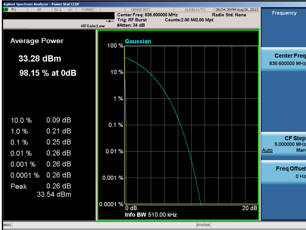
Plot 6-55. Peak-Average Ratio Plot (Cellular GSM Mode – Ch. 190)
