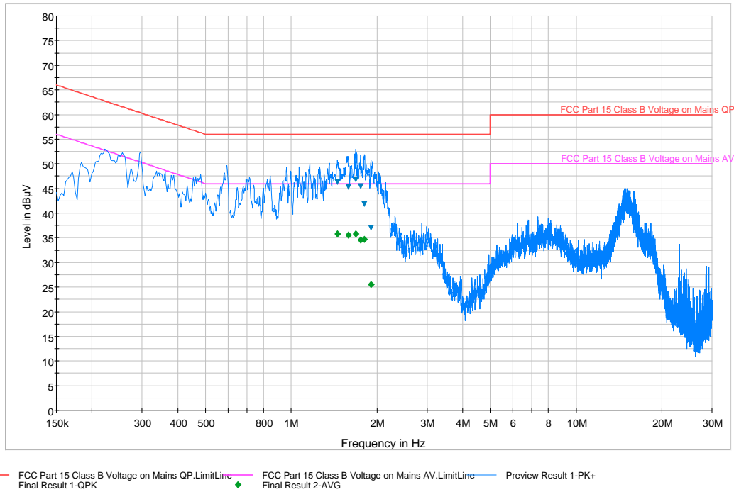
Plot 6-85. Line Conducted Plot with 802.11a UNII Band 2 (N)
