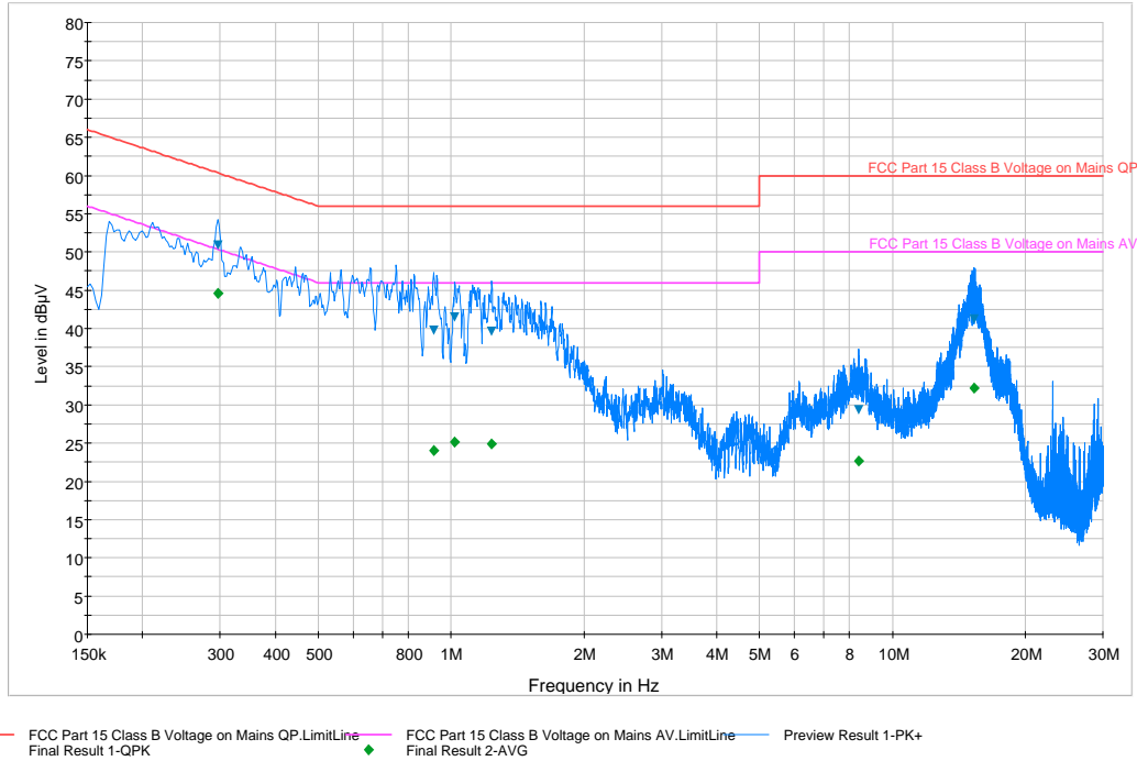
Plot 6-86. Line Conducted Plot with 802.11a UNII Band 3 (L1)
