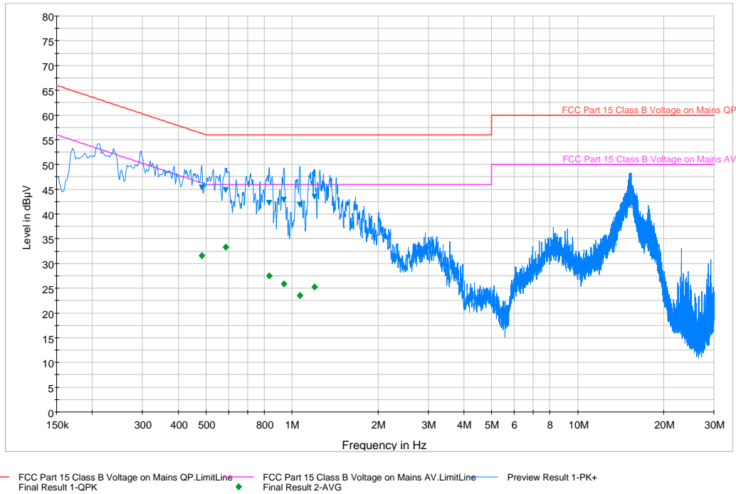
Plot 6-87. Line Conducted Plot with 802.11a UNII Band 3 (N)
