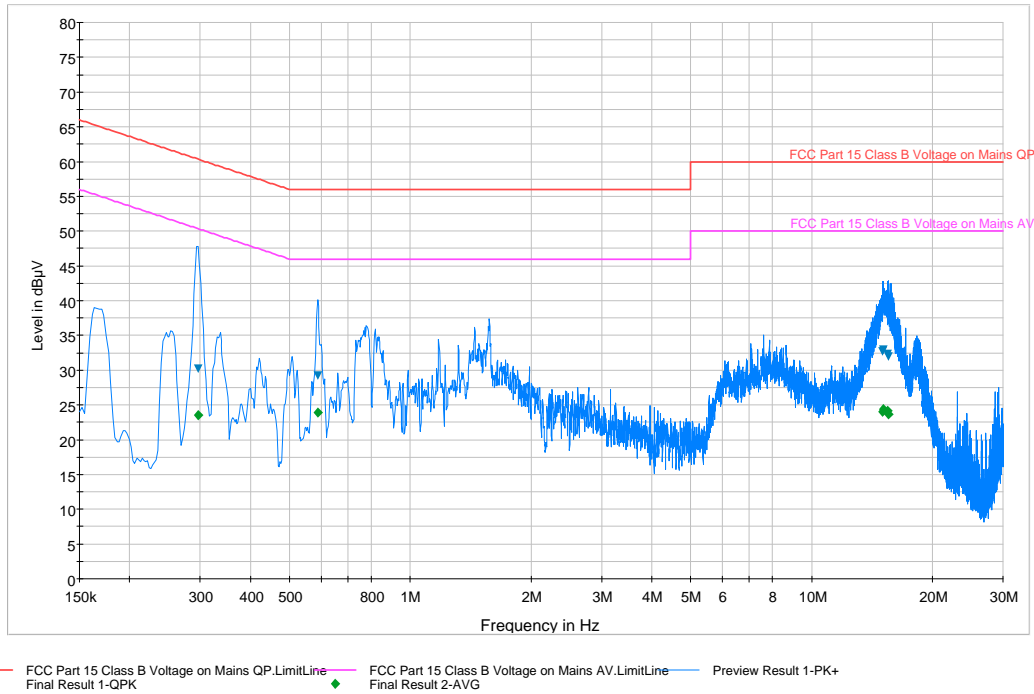
Plot 6-83. Line Conducted Plot with 802.11a UNII Band 1 (N)
