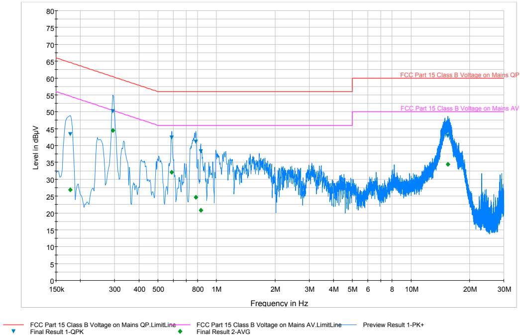
Plot 6-67. Line Conducted Plot with 802.11b (L1)
