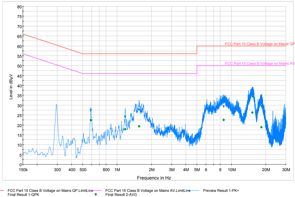
Plot 6-69. Line Conducted Plot with 802.11a (L1)
