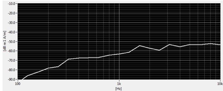
Figure 7-3 Worst-case ABM2 Plot for UMTS
