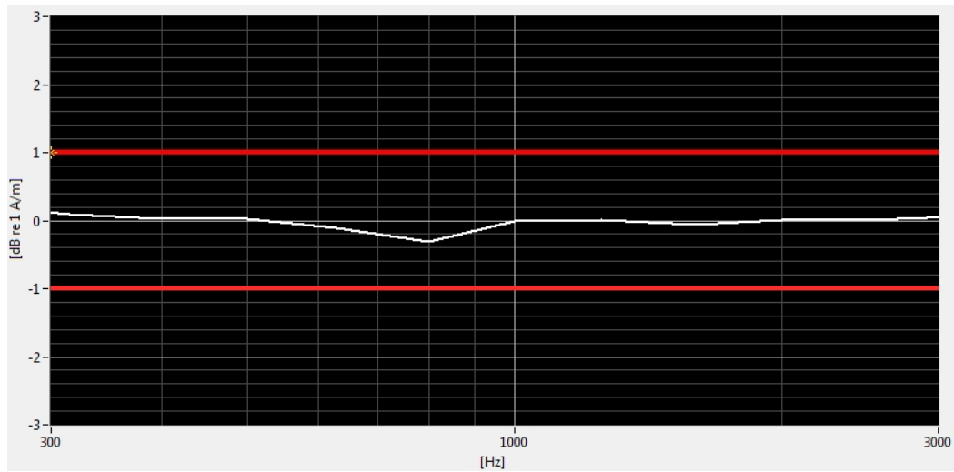
Figure 7-4 Helmholtz Coil Validation for Frequency Response
