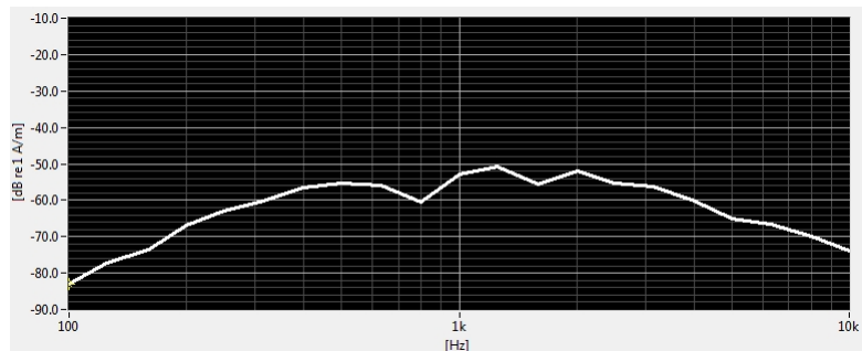
Figure 7-2 Worst-case ABM2 Plot for CDMA
