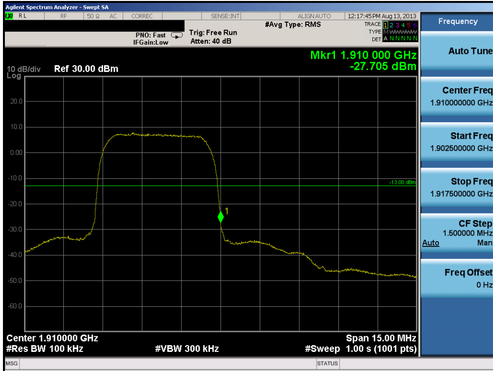
Plot 6-64. Band Edge Plot (PCS WCDMA Mode – Ch. 9538)
