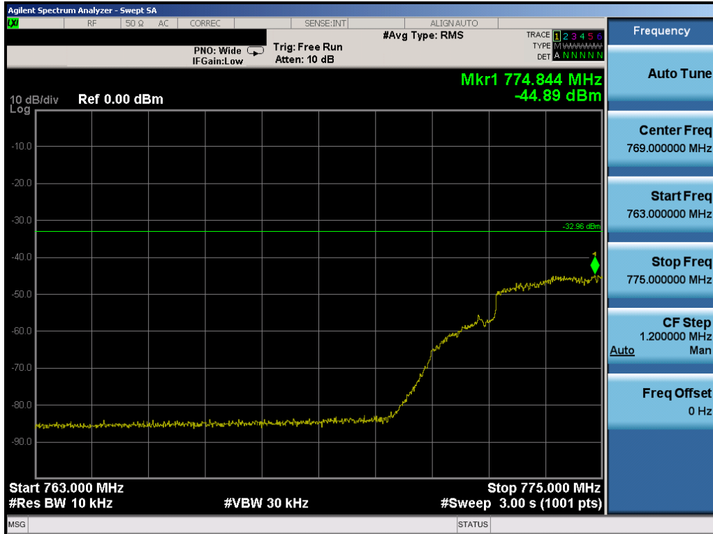
Plot 7-2. Lower Emission Mask Plot (5.0MHz QPSK – RB Size 25)
