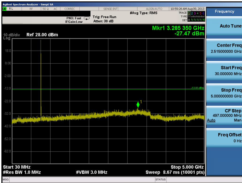
Plot 7-17. Conducted Spurious Plot (10.0MHz QPSK – RB Size 1, RB Offset 0)
