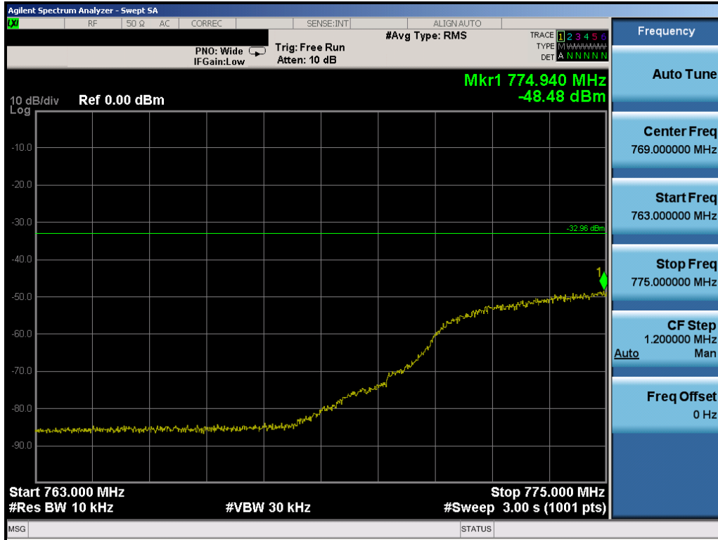
Plot 7-14. Lower Emission Mask Plot (10.0MHz QPSK – RB Size 50)
