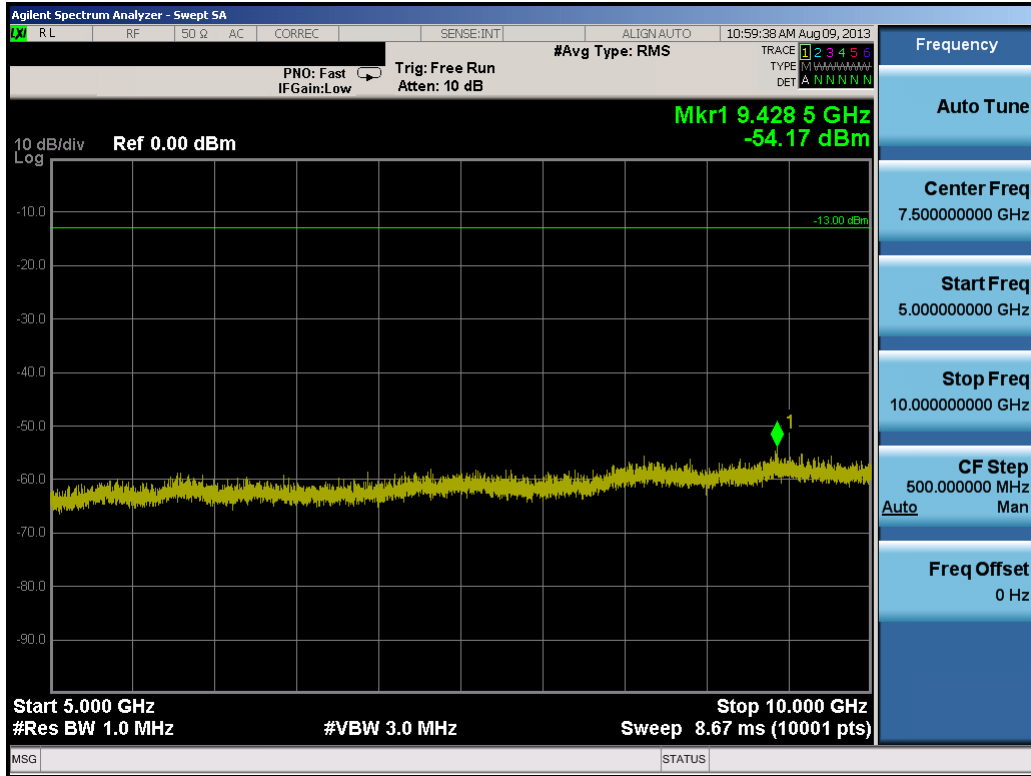
Plot 7-18. Conducted Spurious Plot (10.0MHz QPSK – RB Size 1, RB Offset 0)
