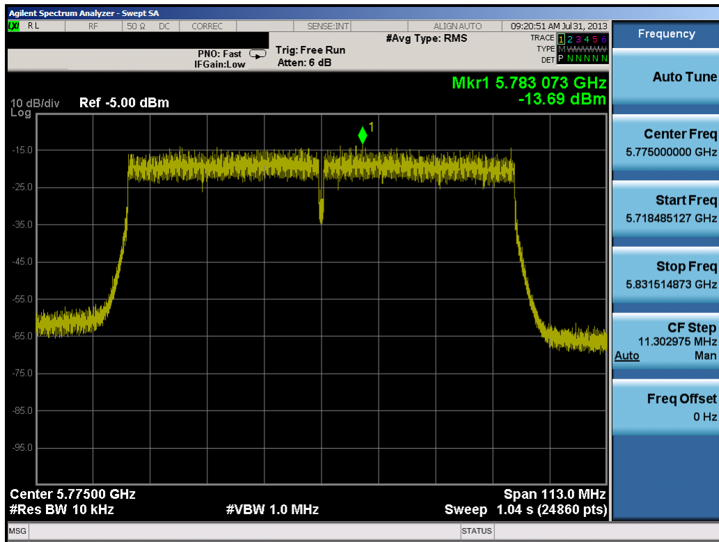
Plot 6-36. Power Spectral Density Plot (80MHz BW 802.11ac (5.8GHz) – Ch. 15)
