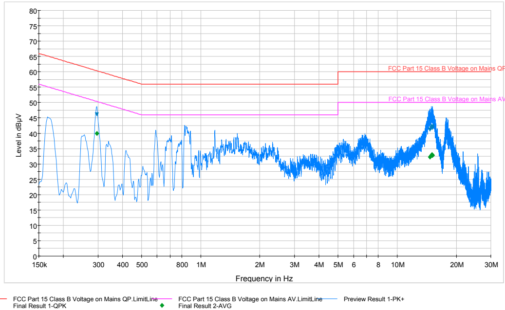
Plot 6-71. Line Conducted Plot with 802.11a (N)
