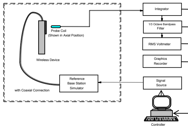
Figure 5-14 Audio Magnetic Field Test Setup for GSM/UMTS
