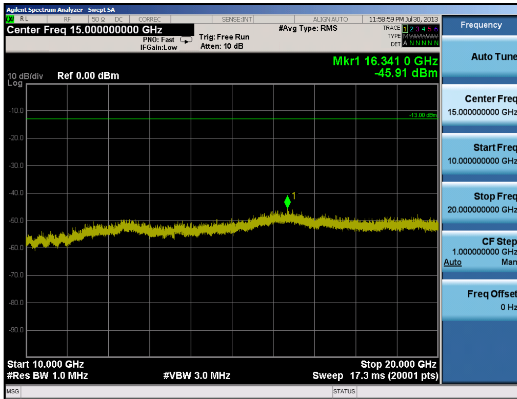
Plot 10-34. Conducted Spurious Plot (20.0MHz QPSK – RB Size 1, RB Offset 0 – High Channel)
