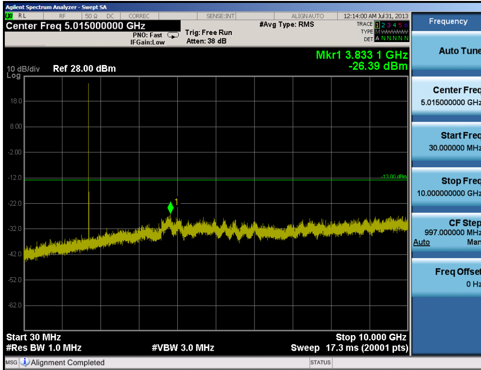
Plot 9-13. Conducted Spurious Plot (10.0MHz QPSK – RB Size 1, RB Offset 0– Low Channel)
