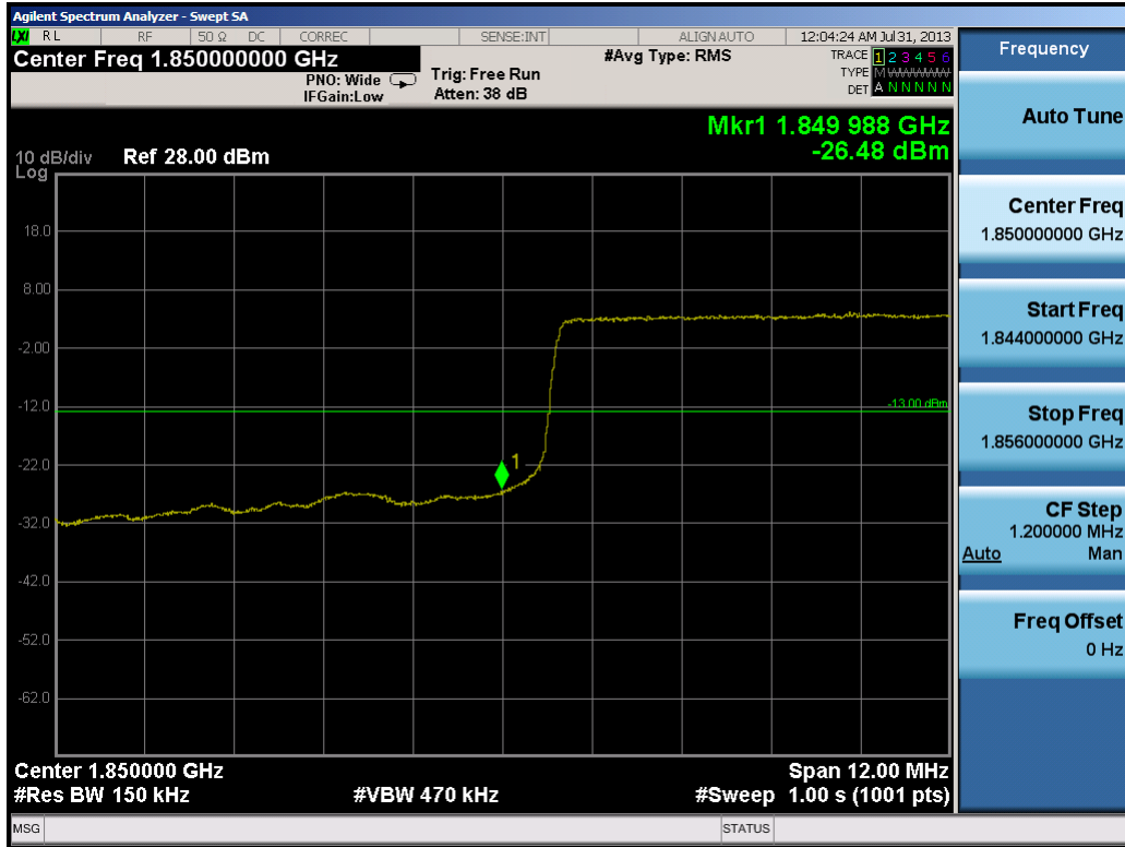
Plot 10-17. Lower Band Edge Plot (15.0MHz QPSK – RB Size 75)
