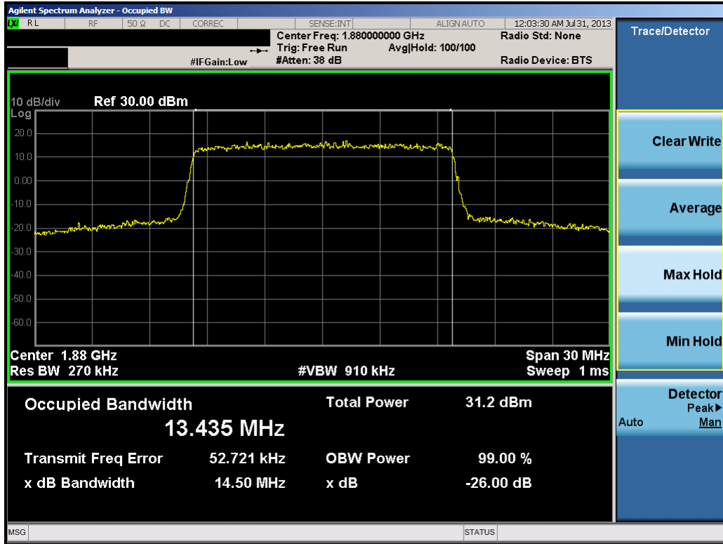
Plot 10-19. Occupied Bandwidth Plot (15.0MHz QPSK – RB Size 75)
