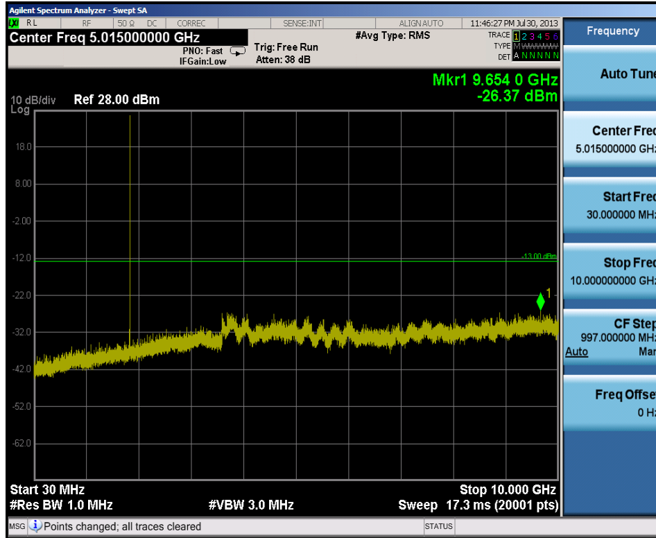
Plot 10-29. Conducted Spurious Plot (20.0MHz QPSK – RB Size 1, RB Offset 0– Low Channel)
