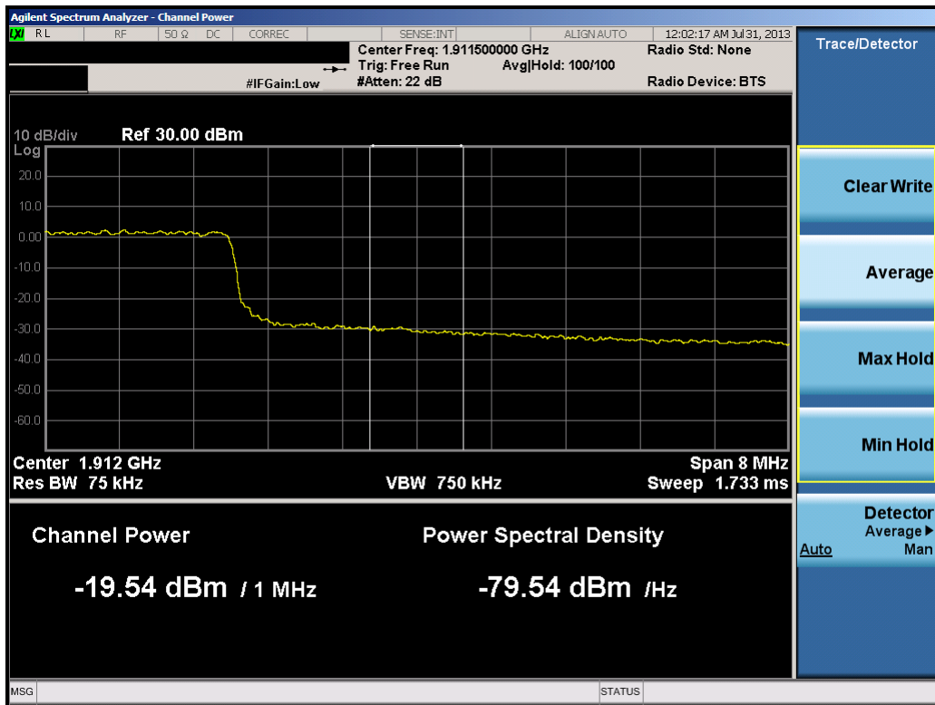
Plot 10-14. Upper Extended Band Edge Plot (10.0MHz QPSK – RB Size 50)
