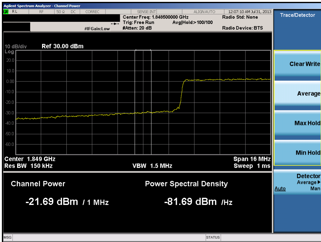
Plot 10-26. Lower Extended Band Edge Plot (20.0MHz QPSK – RB Size 100)
