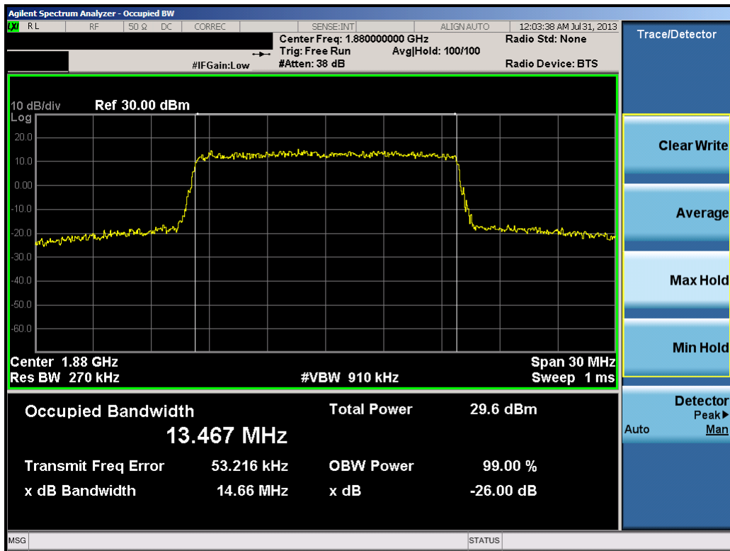
Plot 10-20. Occupied Bandwidth Plot (15.0MHz 16-QAM – RB Size 75)
