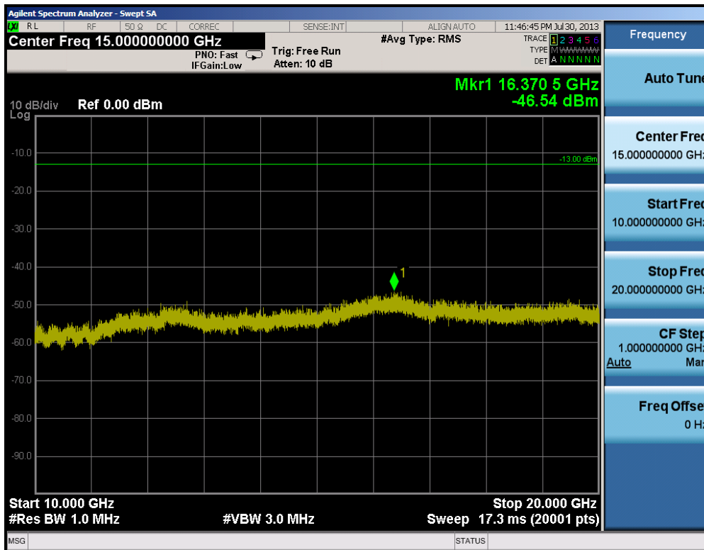
Plot 10-30. Conducted Spurious Plot (20.0MHz QPSK – RB Size 1, RB Offset 0 – Low Channel)
