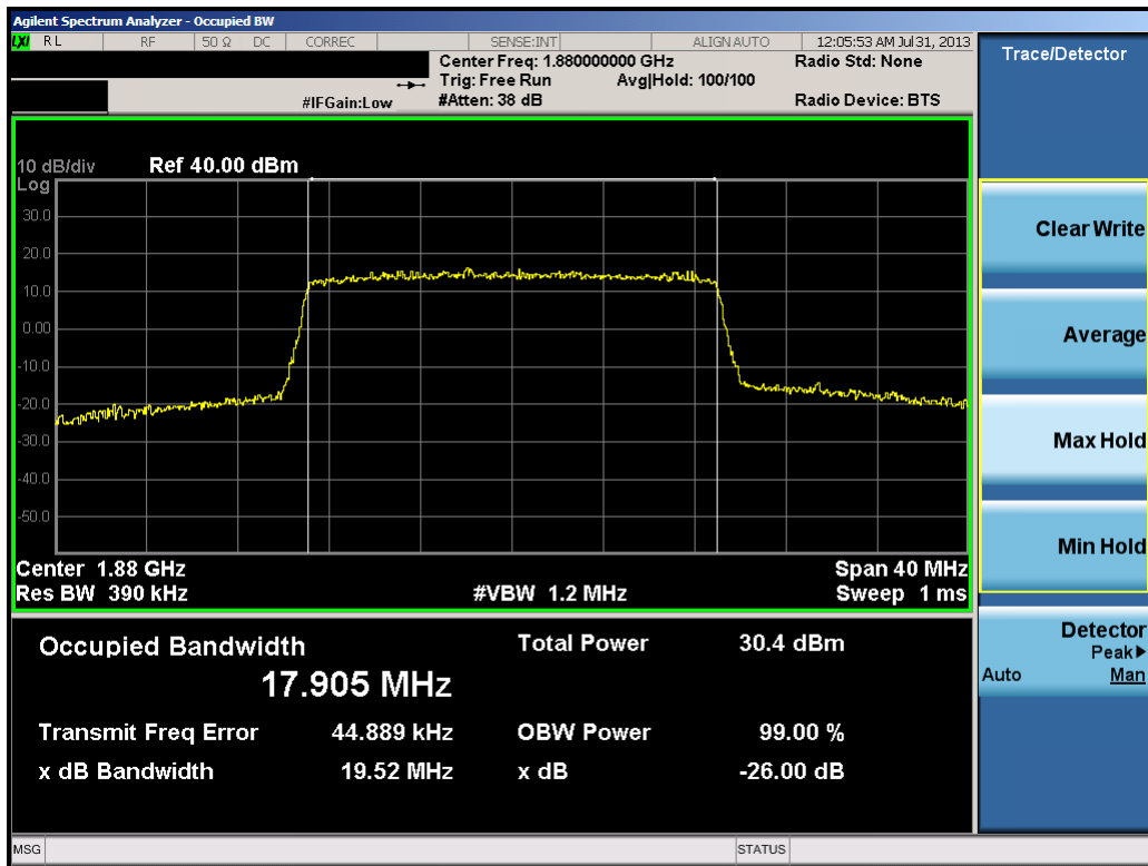
Plot 10-28. Occupied Bandwidth Plot (20.0MHz 16-QAM – RB Size 100)
