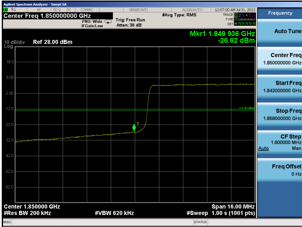
Plot 10-25. Lower Band Edge Plot (20.0MHz QPSK – RB Size 100)
