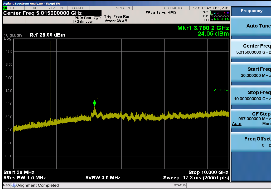
Plot 9-15. Conducted Spurious Plot (10.0MHz QPSK – RB Size 1, RB Offset 0 – Mid Channel)
