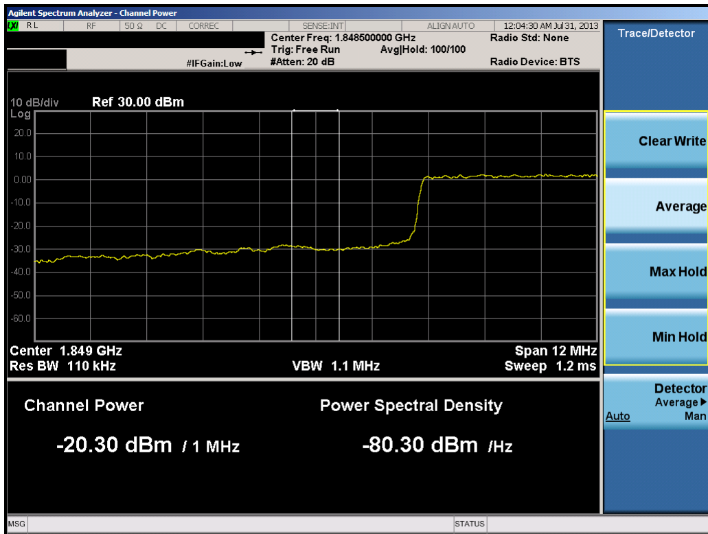
Plot 10-18. Lower Extended Band Edge Plot (15.0MHz QPSK – RB Size 75)
