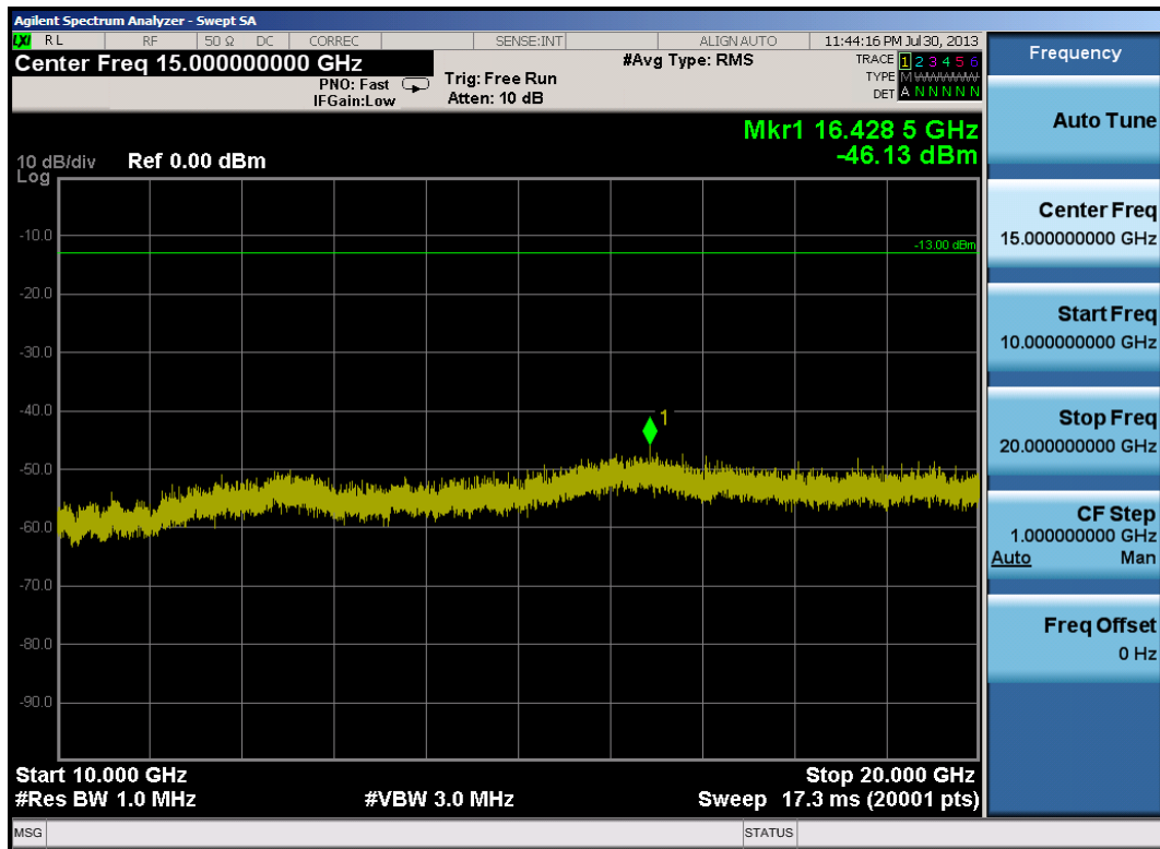
Plot 10-32. Conducted Spurious Plot (20.0MHz QPSK – RB Size 1, RB Offset 0 – Mid Channel)
