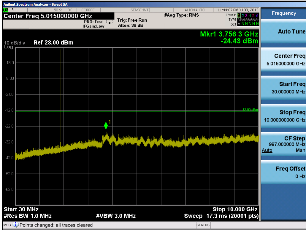
Plot 10-31. Conducted Spurious Plot (20.0MHz QPSK – RB Size 1, RB Offset 0 – Mid Channel)
