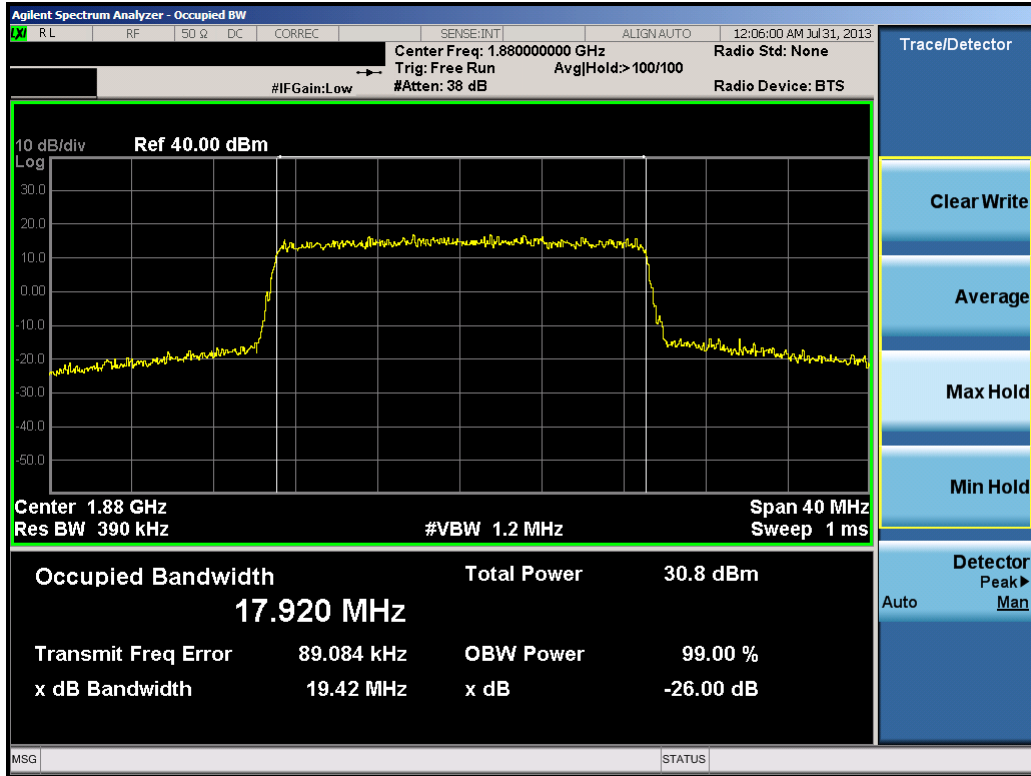
Plot 10-27. Occupied Bandwidth Plot (20.0MHz QPSK – RB Size 100)
