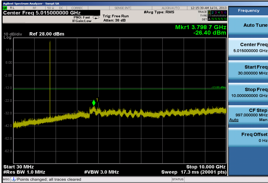
Plot 9-17. Conducted Spurious Plot (10.0MHz QPSK – RB Size 1, RB Offset 0 – High Channel)
