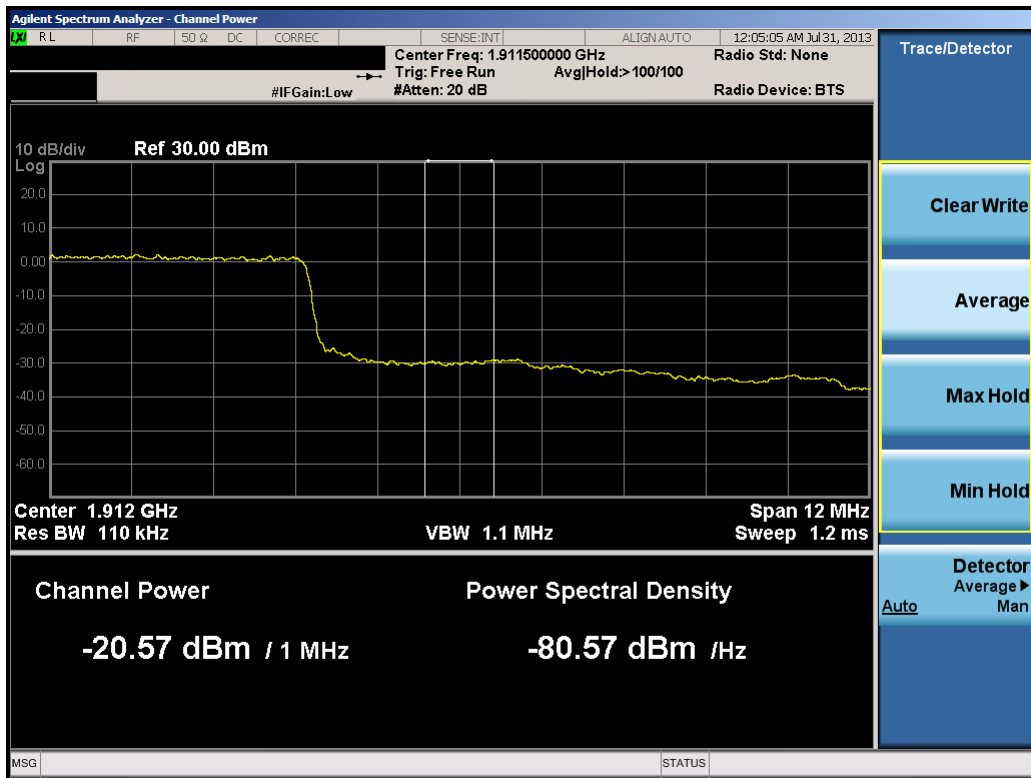
Plot 10-22. Upper Extended Band Edge Plot (15.0MHz QPSK – RB Size 75)
