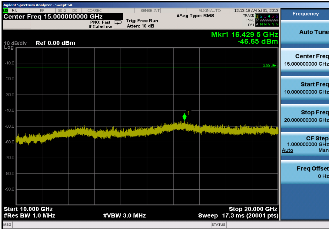
Plot 9-16. Conducted Spurious Plot (10.0MHz QPSK – RB Size 1, RB Offset 0 – Mid Channel)
