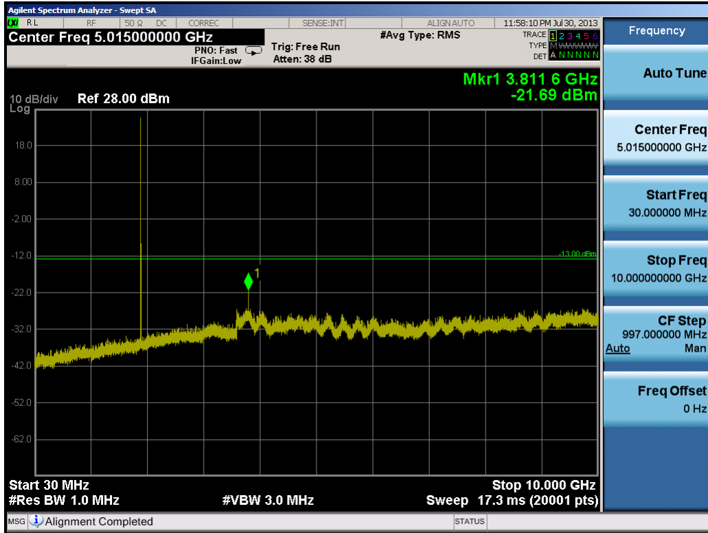
Plot 10-33. Conducted Spurious Plot (20.0MHz QPSK – RB Size 1, RB Offset 0 – High Channel)
