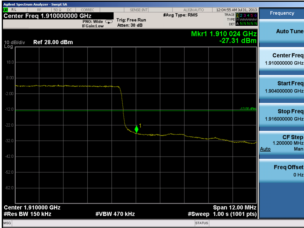
Plot 10-21. Upper Band Edge Plot (15.0MHz QPSK – RB Size 75)
