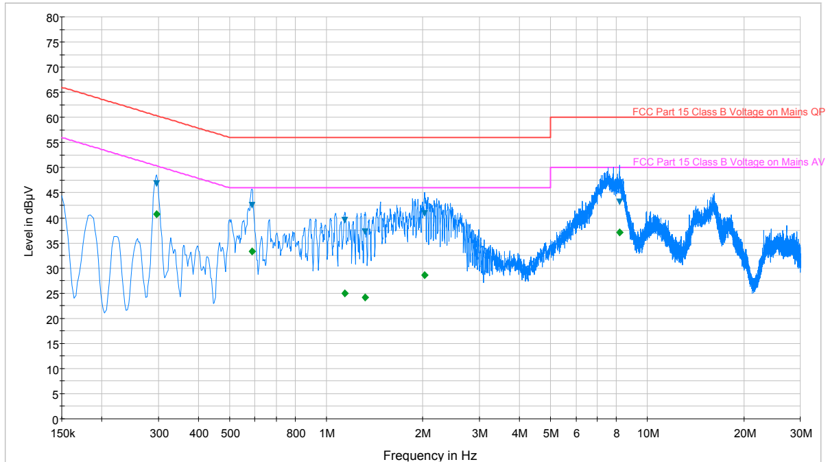
Plot 6-8. Line-Conducted Test Plot (L1)
