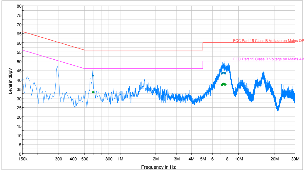
Plot 6-9. Line-Conducted Test Plot (N)
