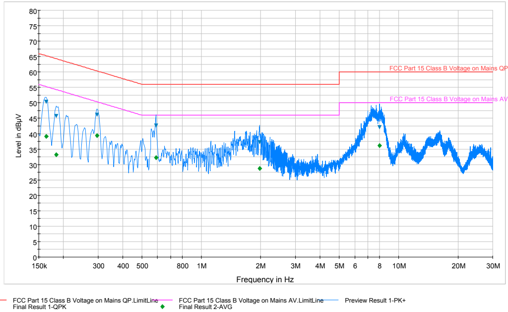
Plot 6-69. Line Conducted Plot with 802.11b (L1)
