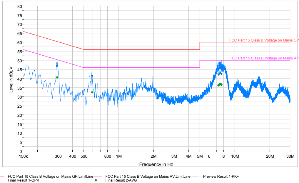
Plot 6-70. Line Conducted Plot with 802.11b (N)
