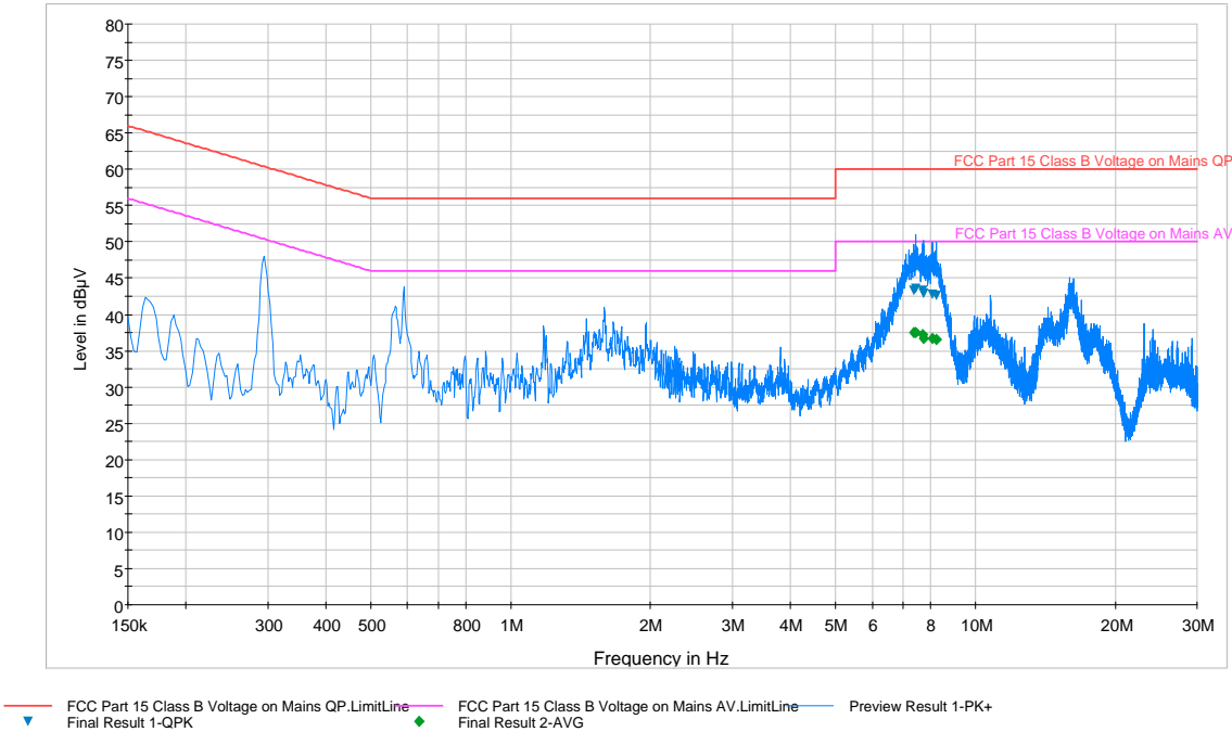
Plot 6-91. Line Conducted Plot with 802.11a UNII Band 2 (N)
