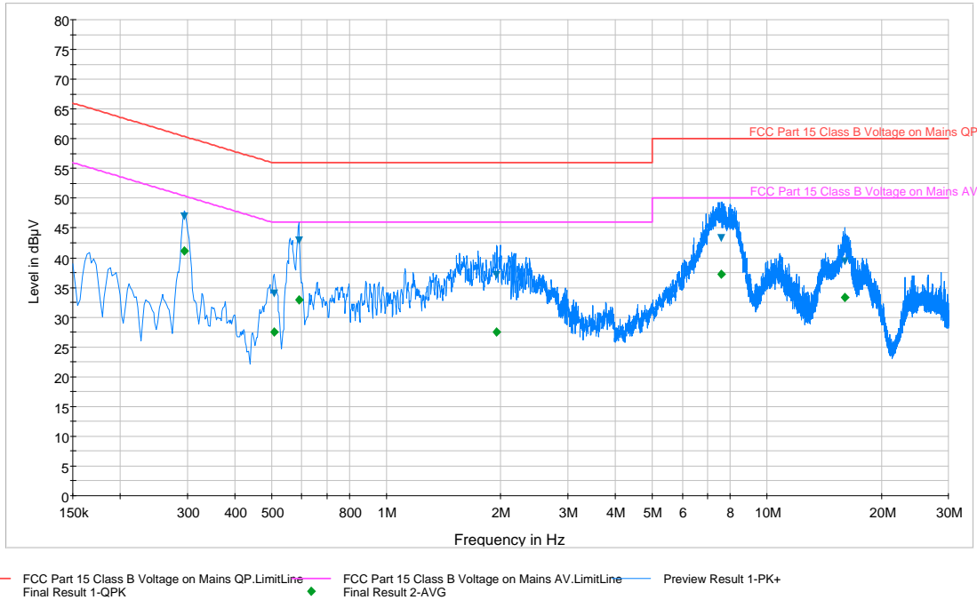
Plot 6-92. Line Conducted Plot with 802.11a UNII Band 3 (L1)
