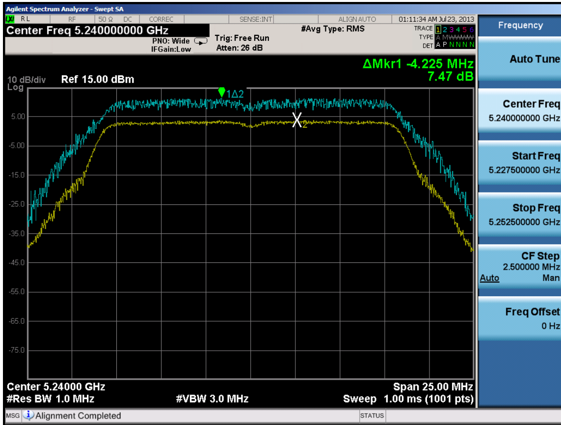
Plot 6-58. Peak Excursion Ratio Plot (802.11a)
