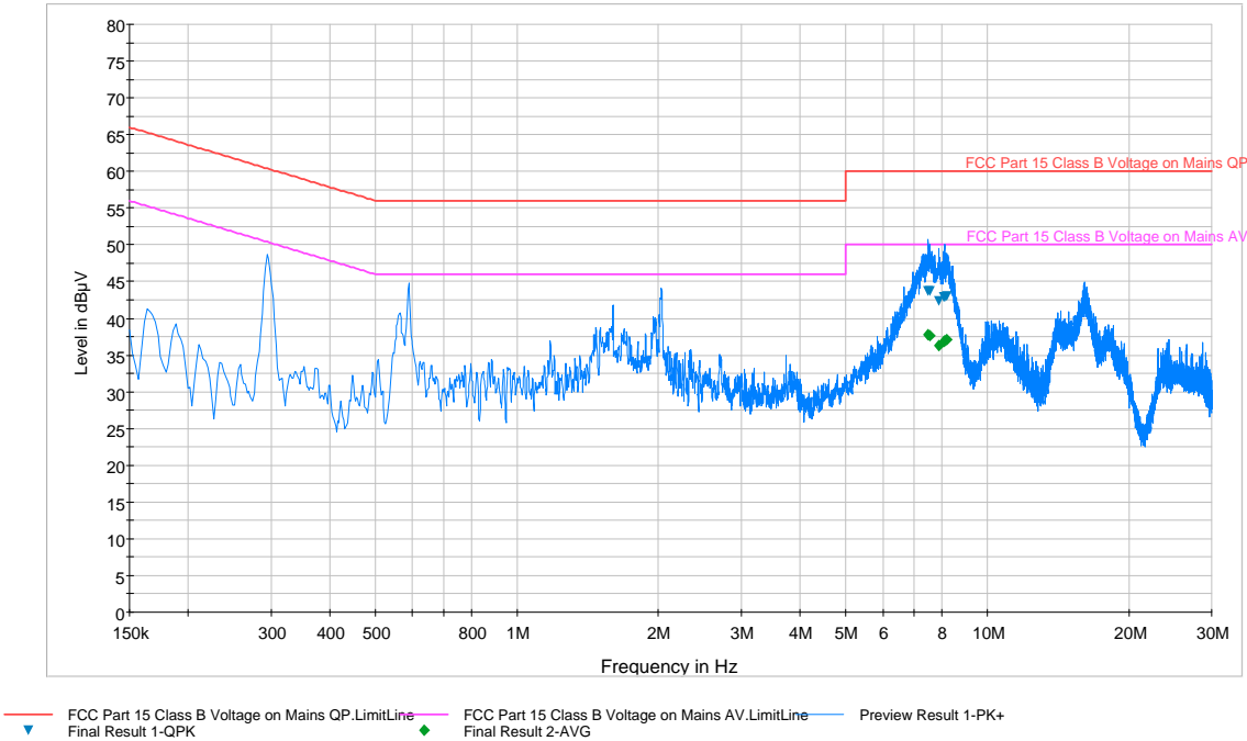
Plot 6-93. Line Conducted Plot with 802.11a UNII Band 3 (N)
