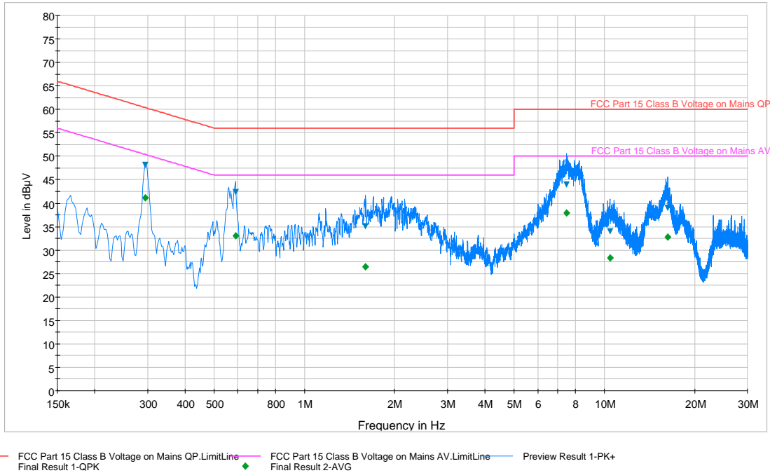
Plot 6-90. Line Conducted Plot with 802.11a UNII Band 2 (L1)
