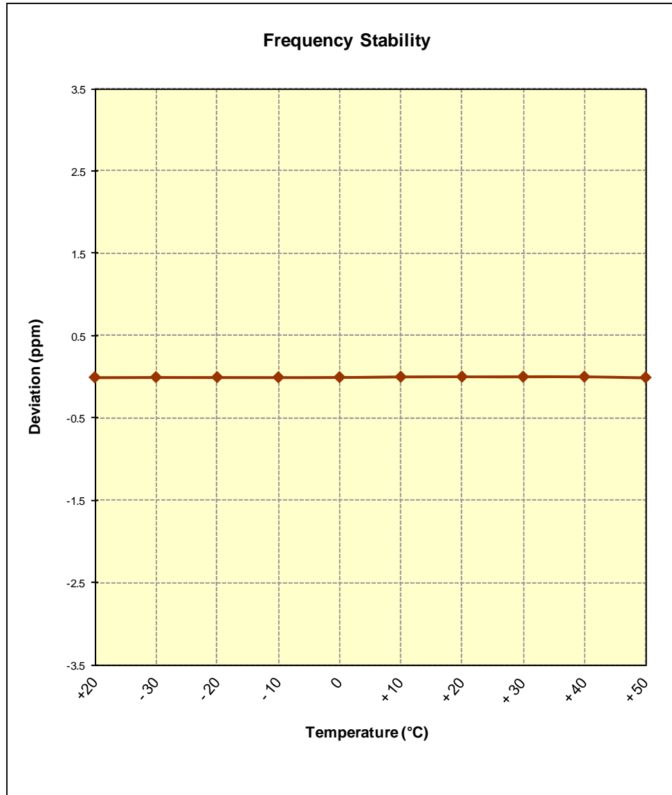
Figure 6-4. Frequency Stability Graph (Band 25)
