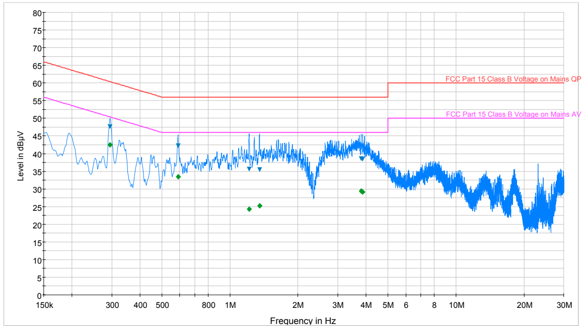
Plot 6-9. Line-Conducted Test Plot (N)
