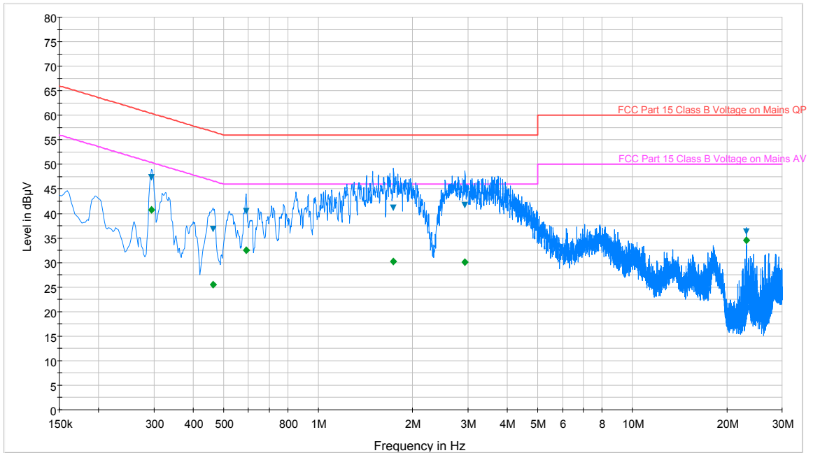
Plot 6-8. Line-Conducted Test Plot (L1)
